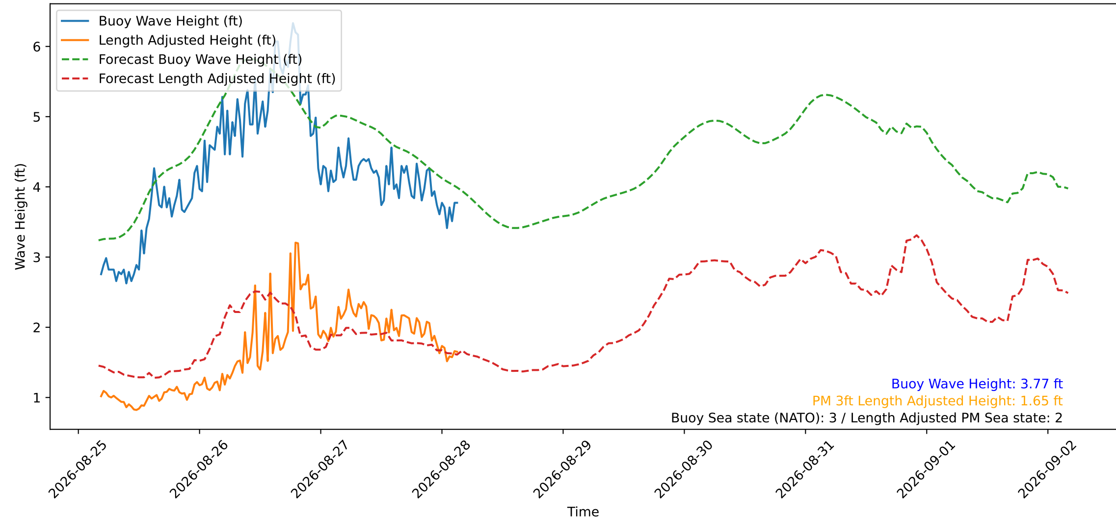
Wave Heights over Time for Green Beach at 2026-08-28 04:01:12
