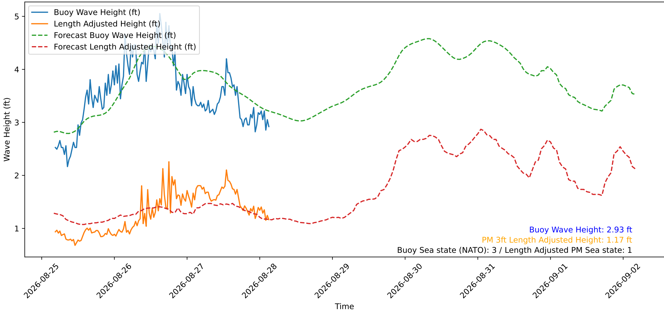
Wave Heights over Time for Red Beach at 2026-08-28 04:00:49
