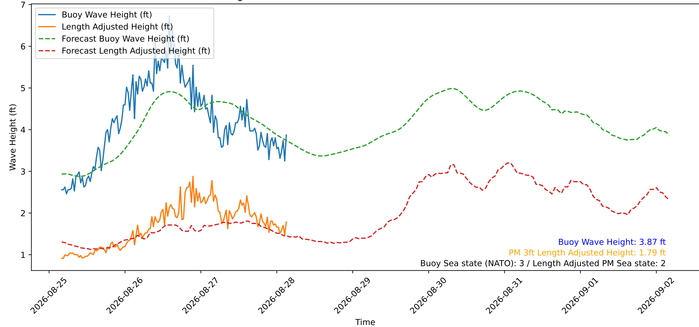
Wave Heights over Time for Oceanside Harbor at 2026-08-28 04:00:29
