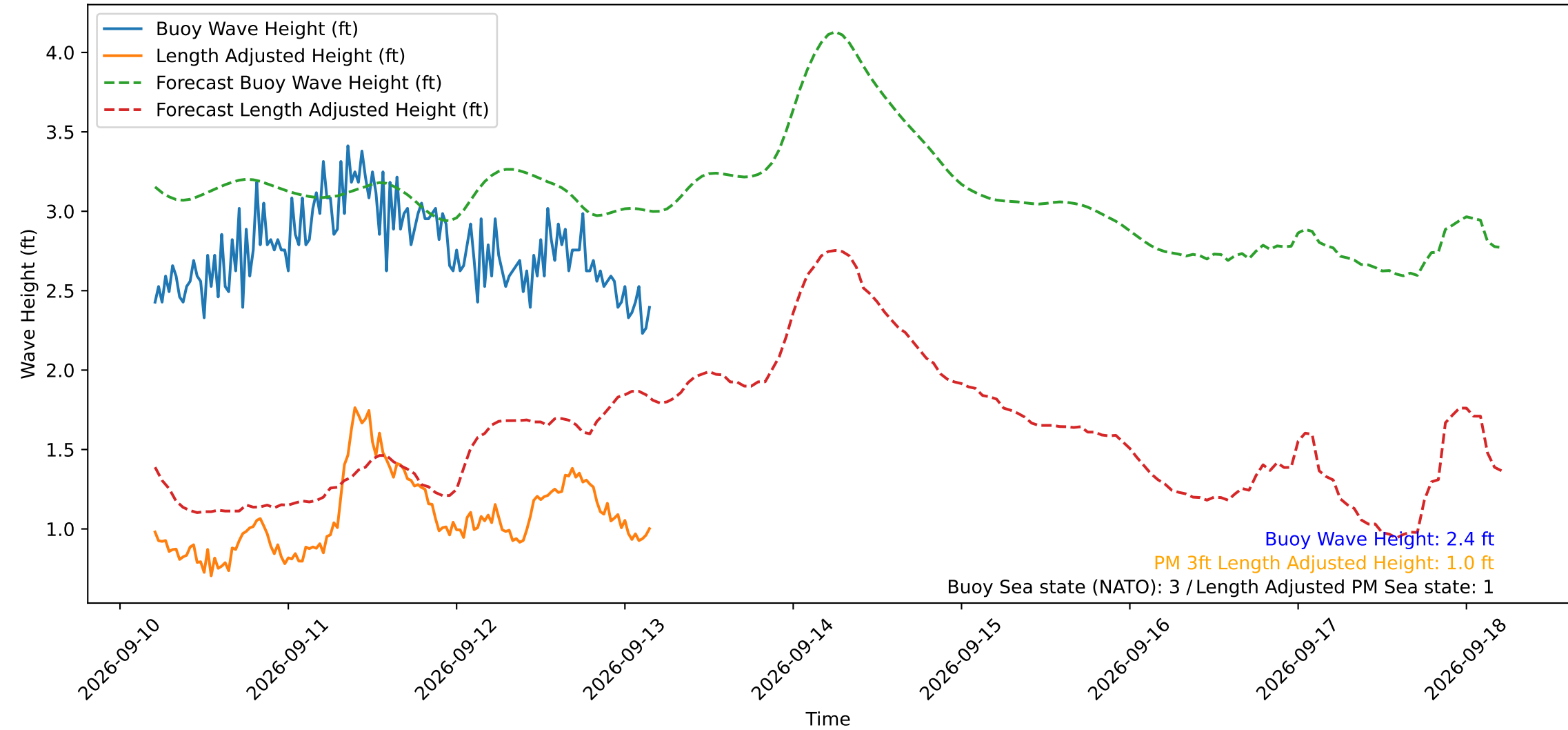
Wave Heights over Time for Red Beach at 2026-09-13 04:30:49
