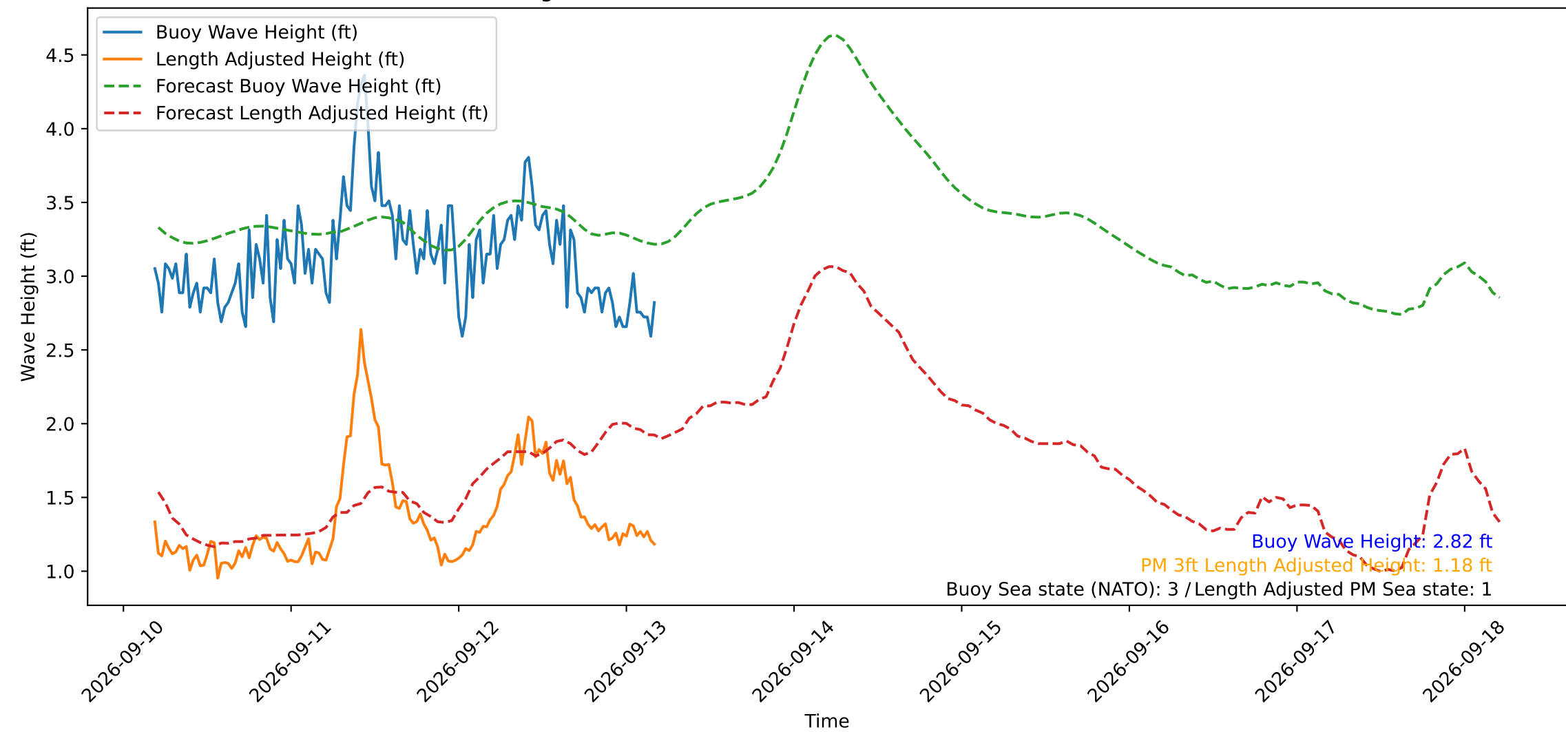
Wave Heights over Time for Oceanside Harbor at 2026-09-13 04:30:30
