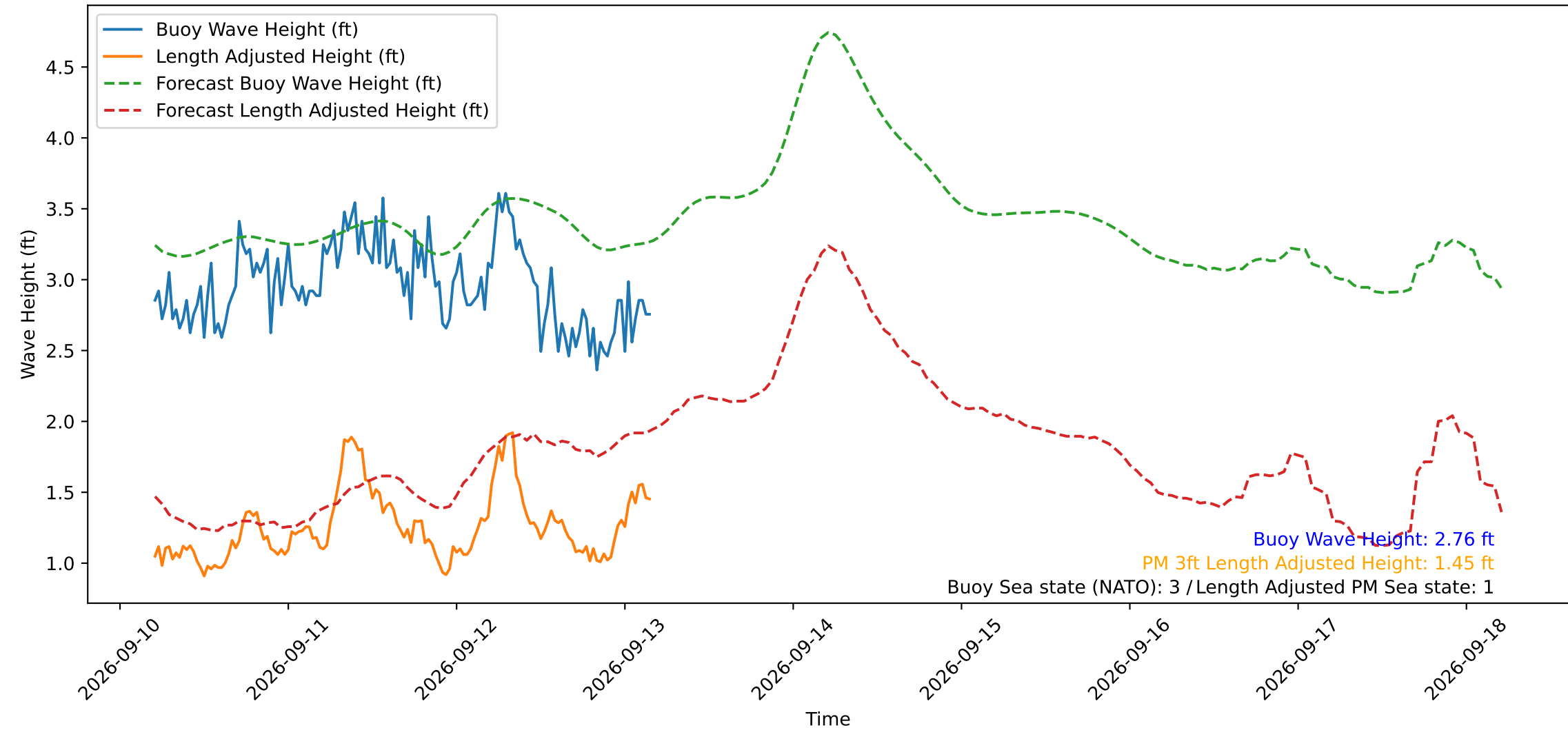
Wave Heights over Time for Green Beach at 2026-09-13 04:31:11
