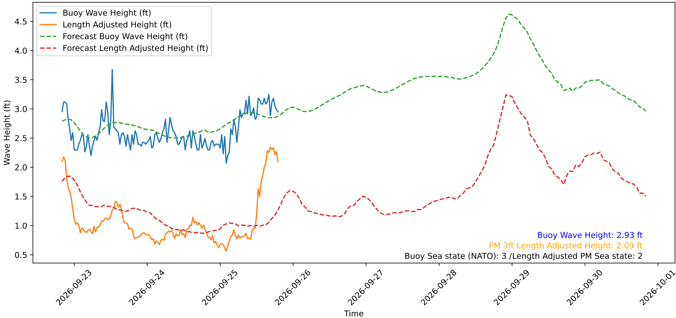
Wave Heights over Time for Red Beach at 2026-09-25 19:50:50
