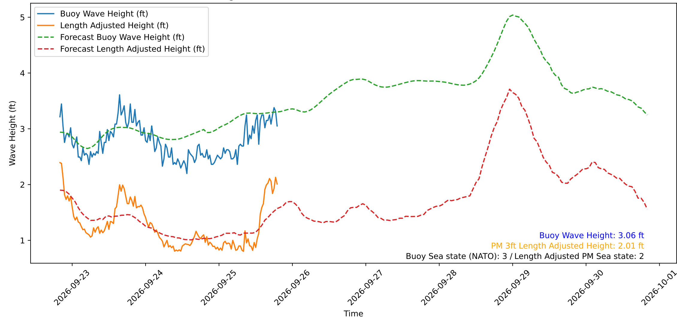
Wave Heights over Time for Oceanside Harbor at 2026-09-25 19:50:29
