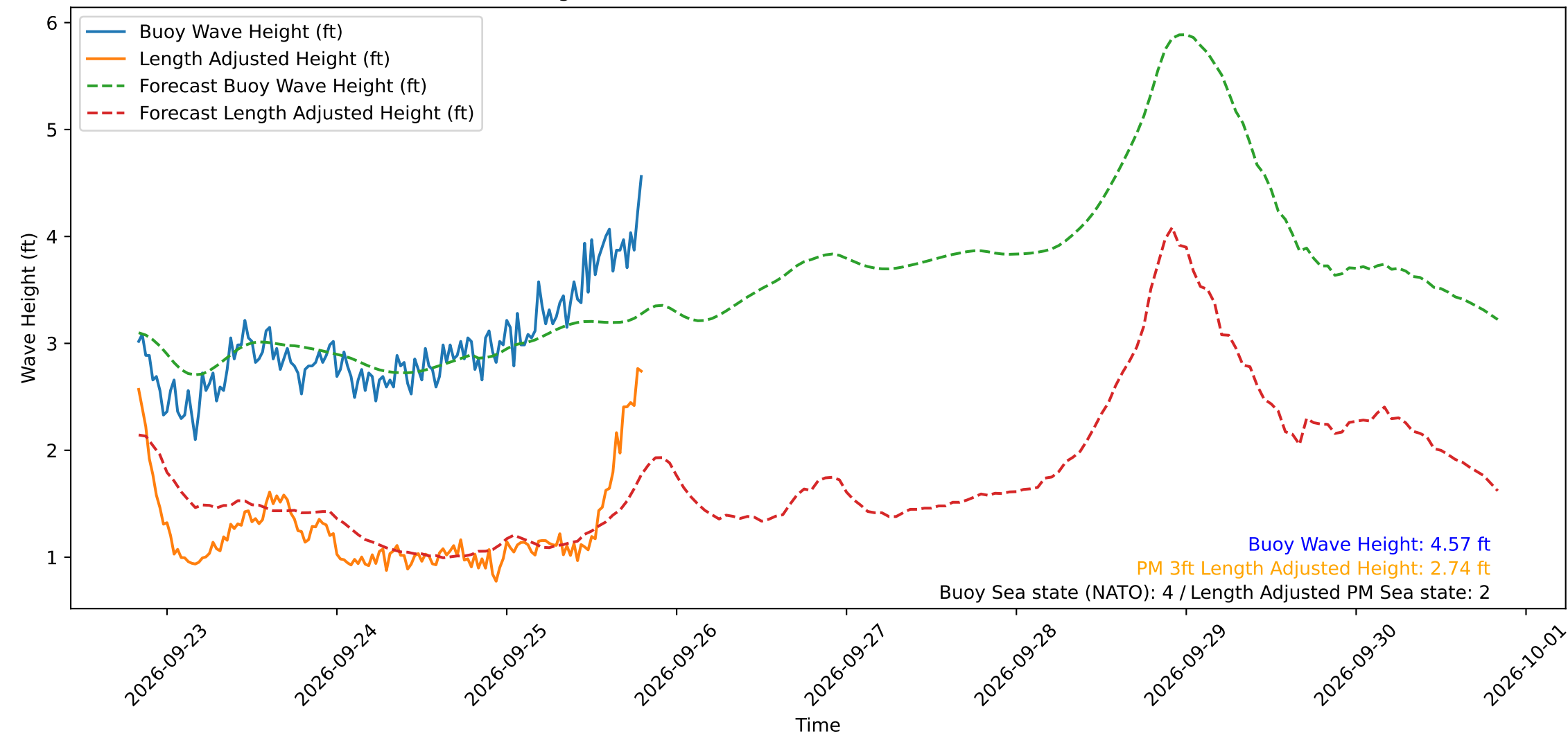
Wave Heights over Time for Green Beach at 2026-09-25 19:51:14
