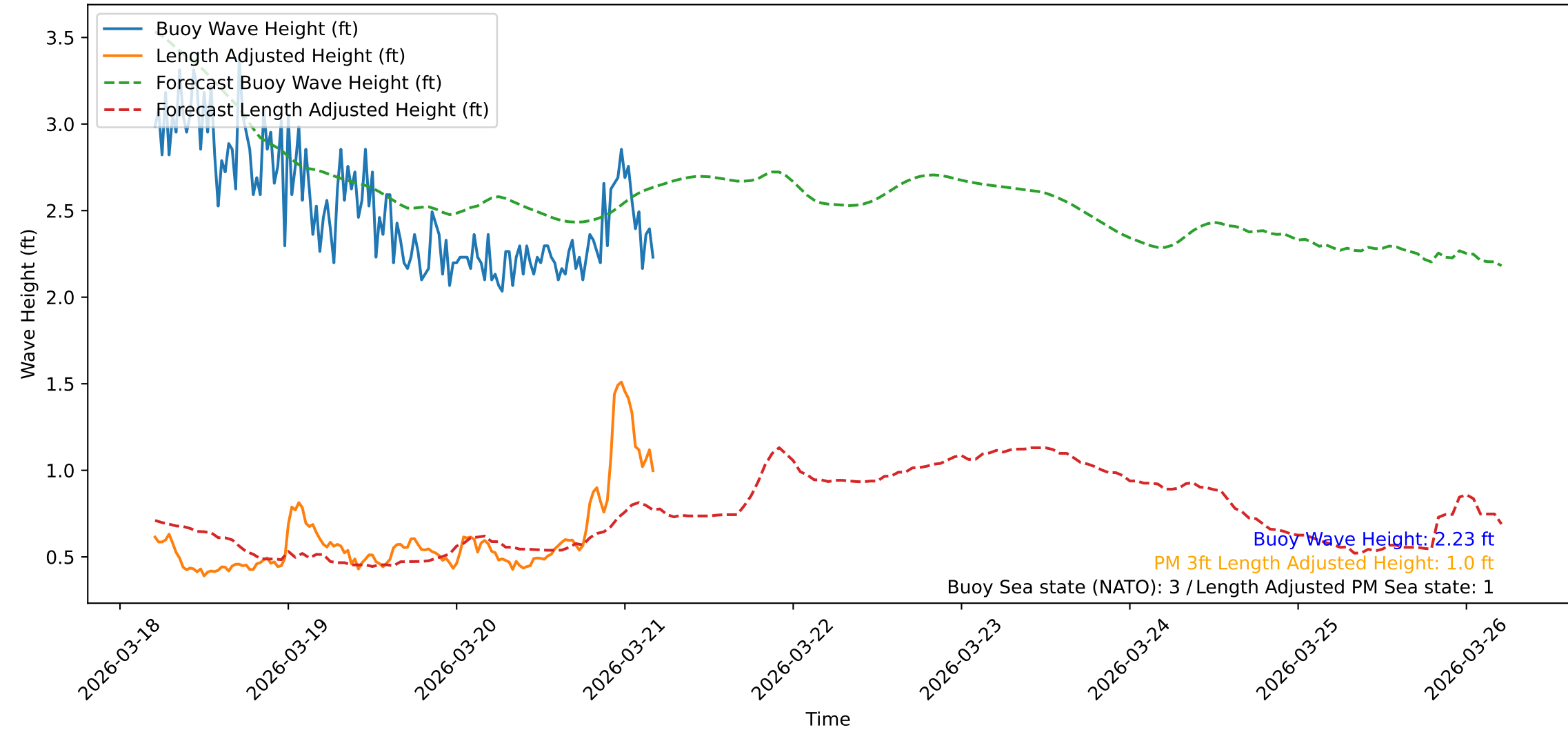
Wave Heights over Time for Green Beach at 2026-03-21 04:51:09
