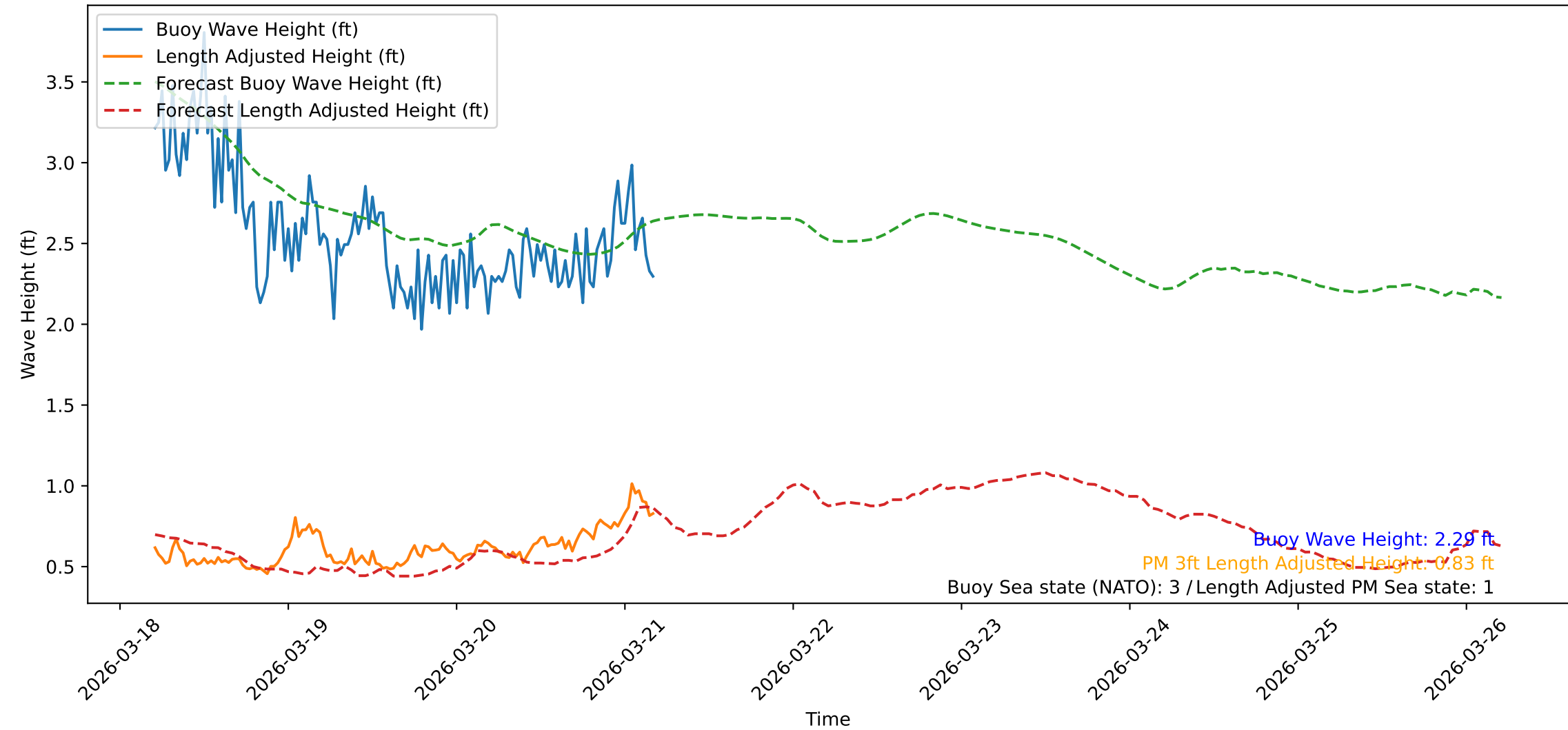
Wave Heights over Time for Oceanside Harbor at 2026-03-21 04:50:31
