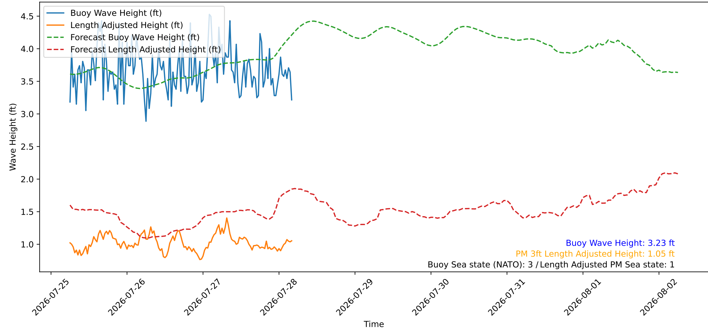
Wave Heights over Time for Red Beach at 2026-07-28 05:30:47
