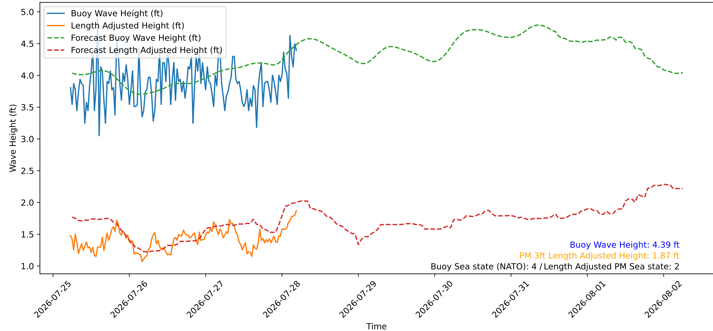
Wave Heights over Time for Oceanside Harbor at 2026-07-28 05:30:27
