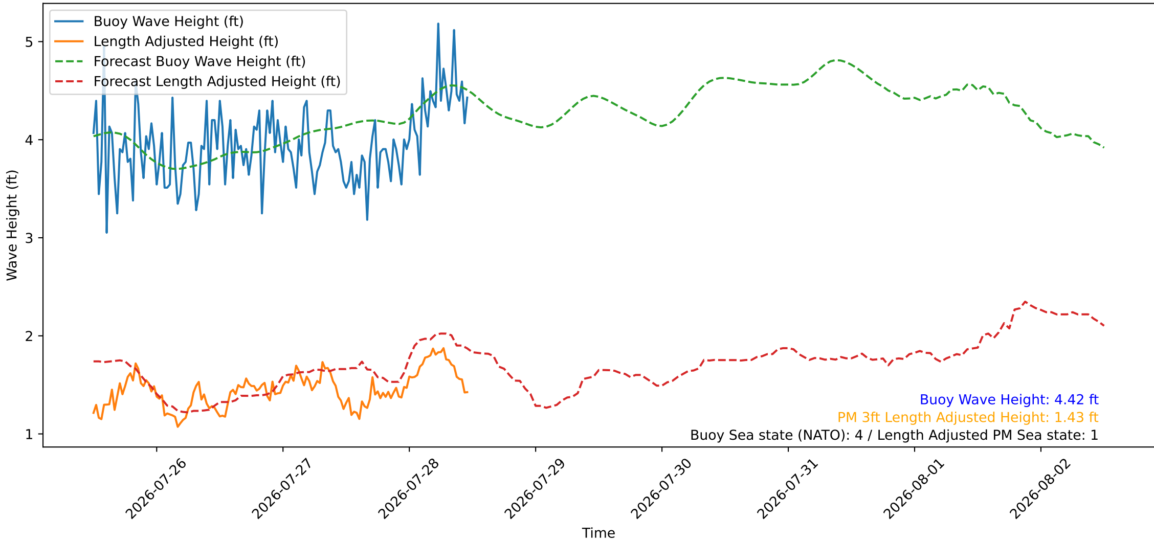
Wave Heights over Time for Oceanside Harbor at 2026-07-28 12:00:26
