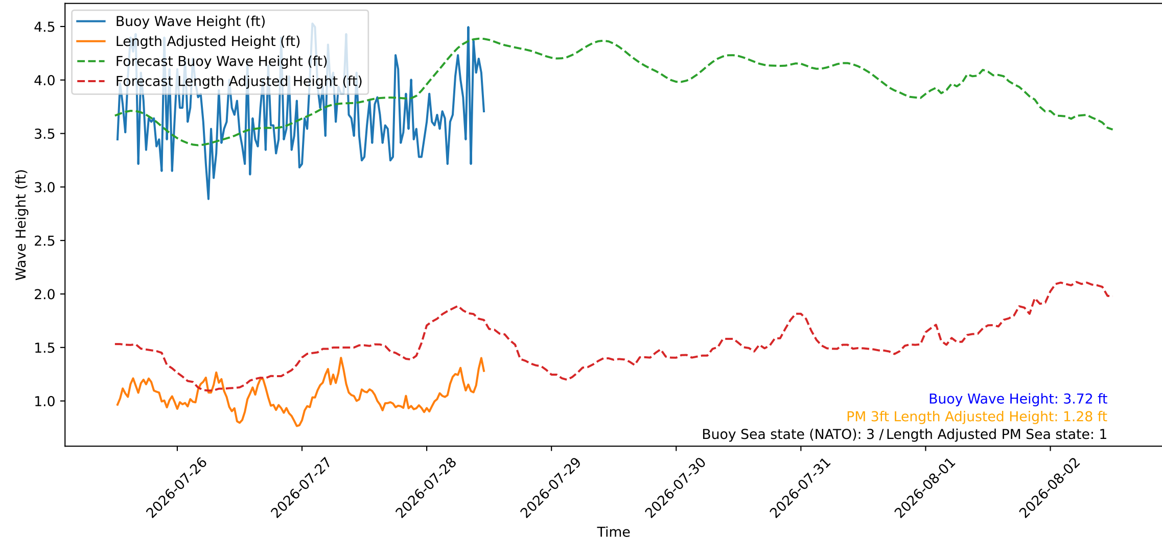
Wave Heights over Time for Red Beach at 2026-07-28 12:00:46
