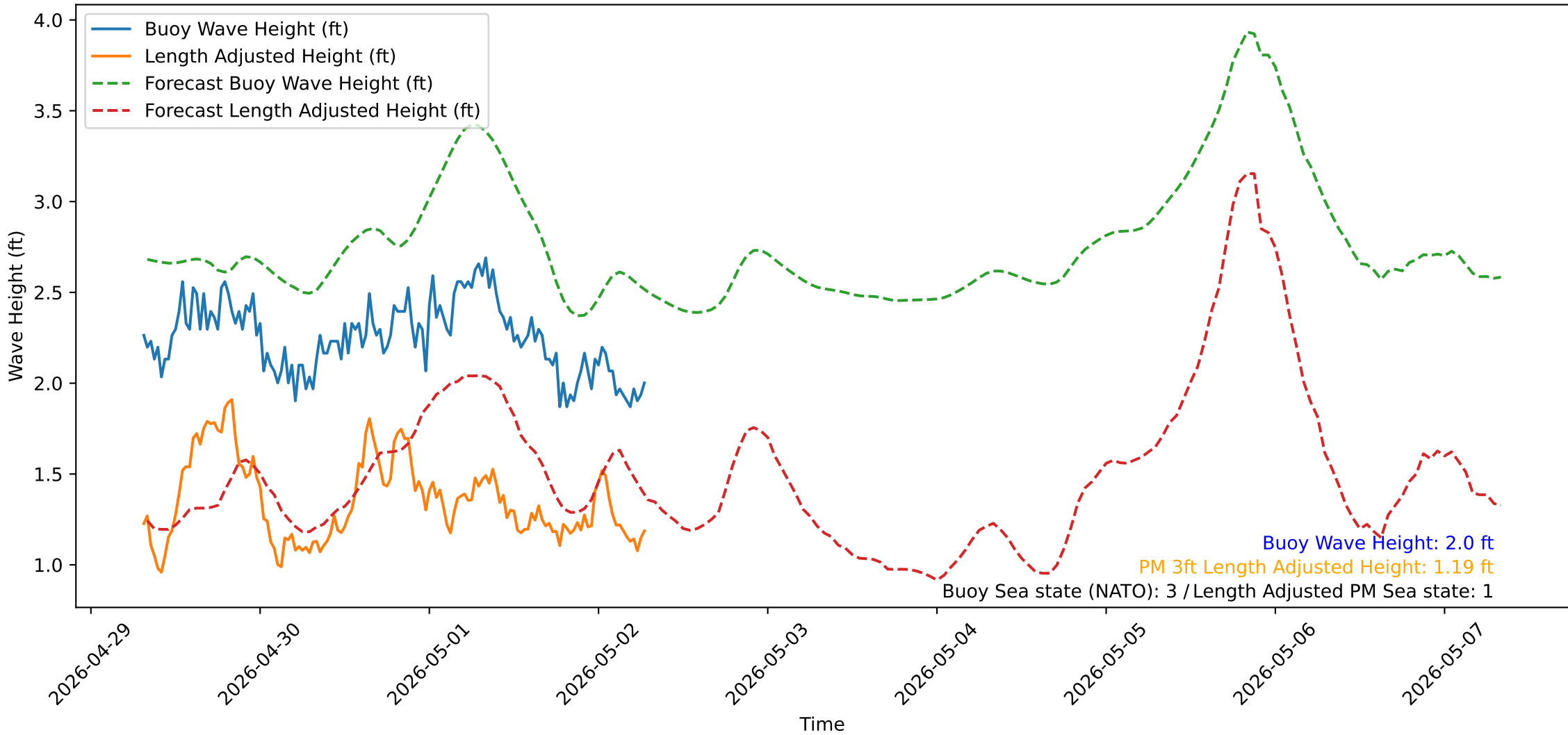
Wave Heights over Time for Oceanside Harbor at 2026-05-02 07:30:32
