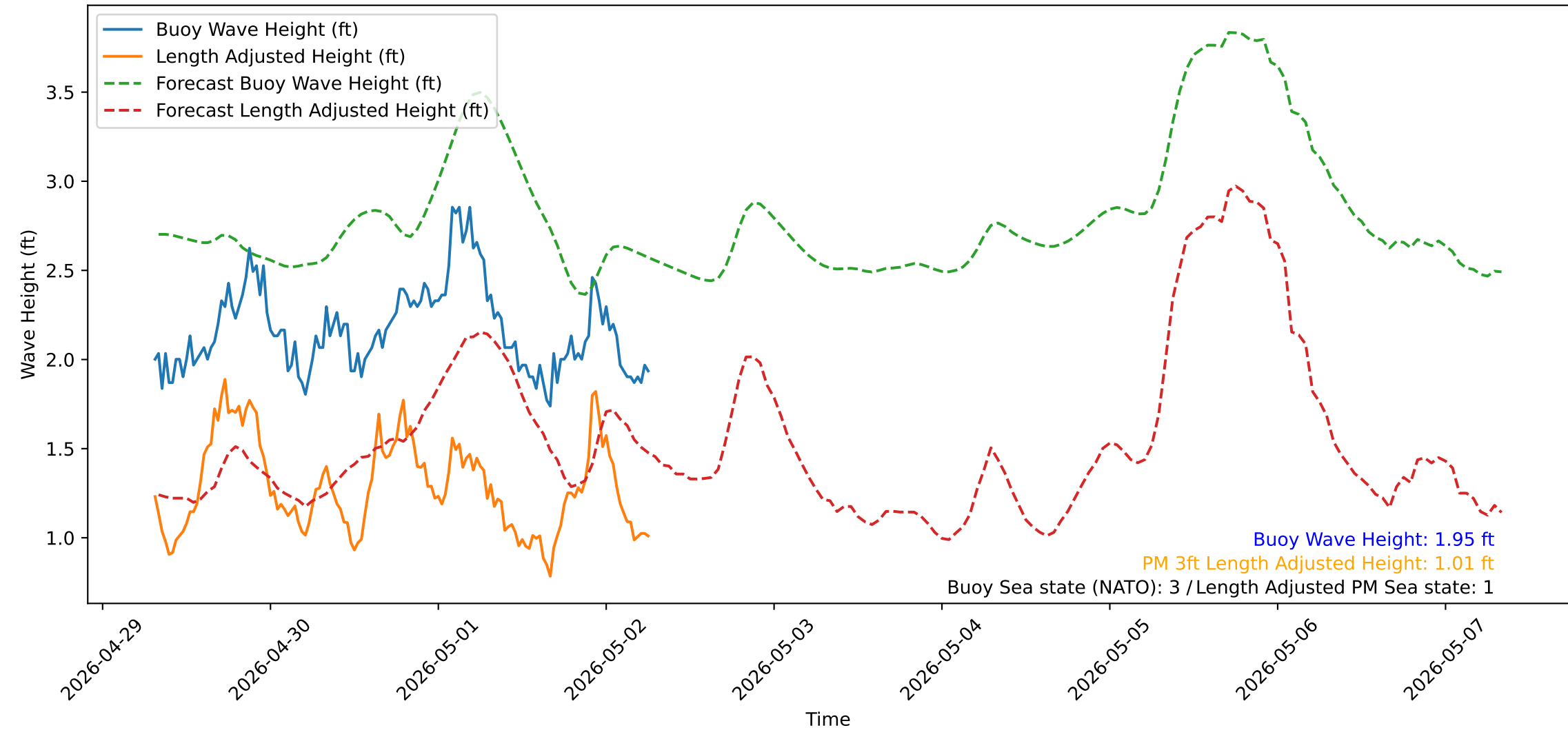
Wave Heights over Time for Green Beach at 2026-05-02 07:31:13
