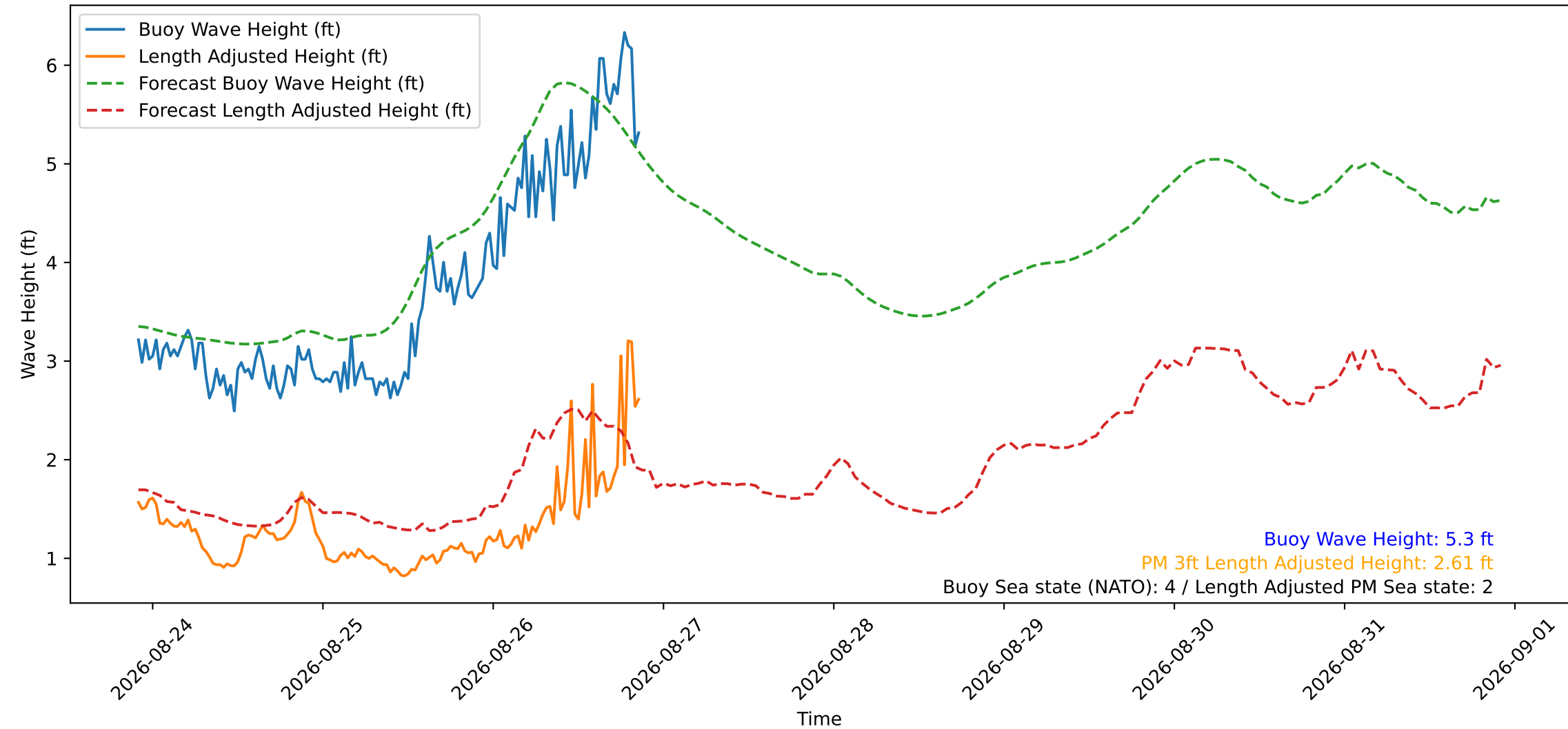
Wave Heights over Time for Green Beach at 2026-08-26 21:31:12
