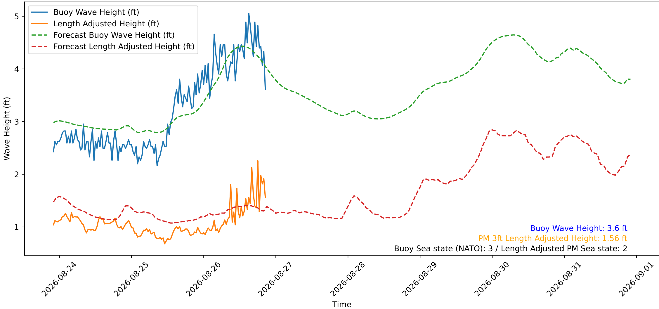
Wave Heights over Time for Red Beach at 2026-08-26 21:30:49
