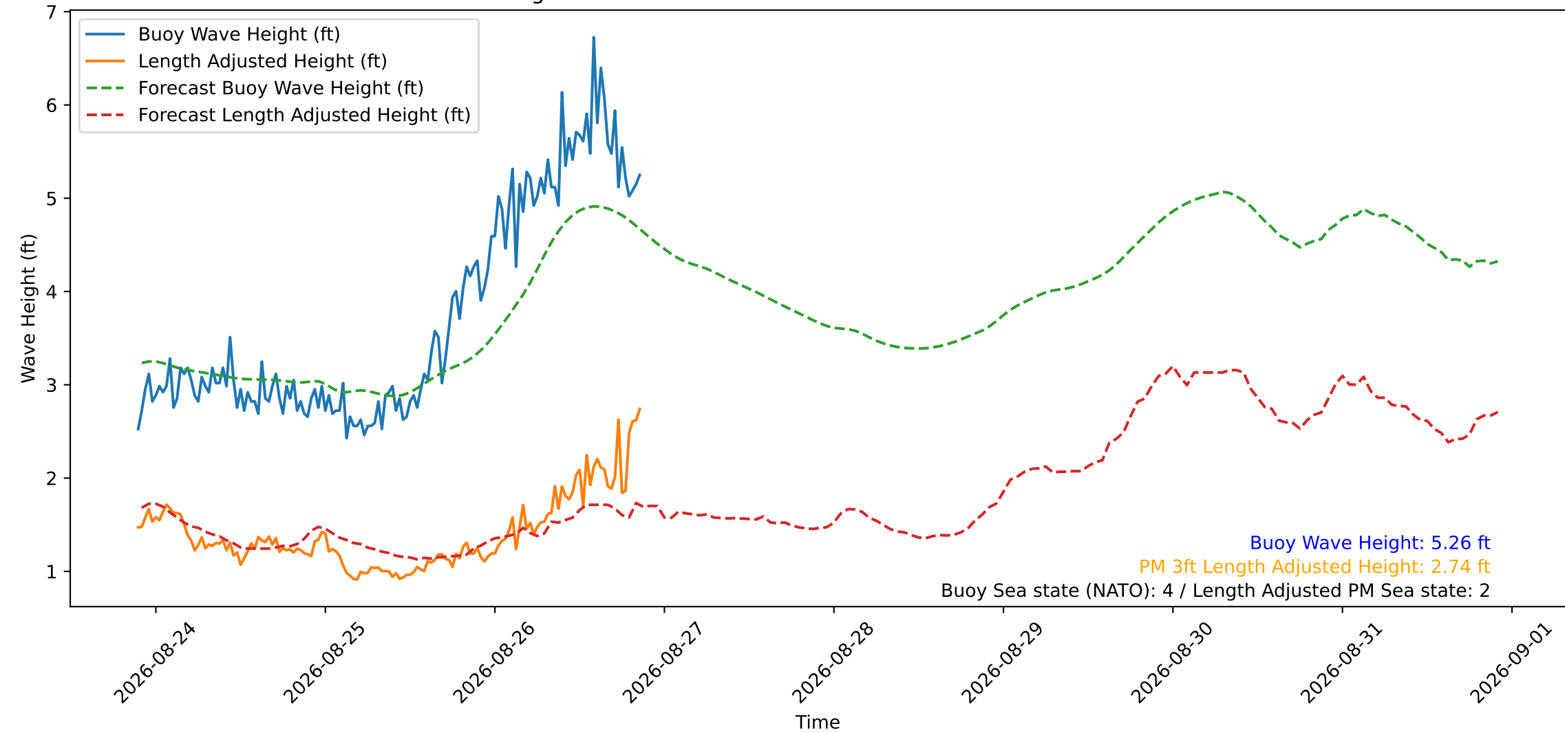
Wave Heights over Time for Oceanside Harbor at 2026-08-26 21:30:30
