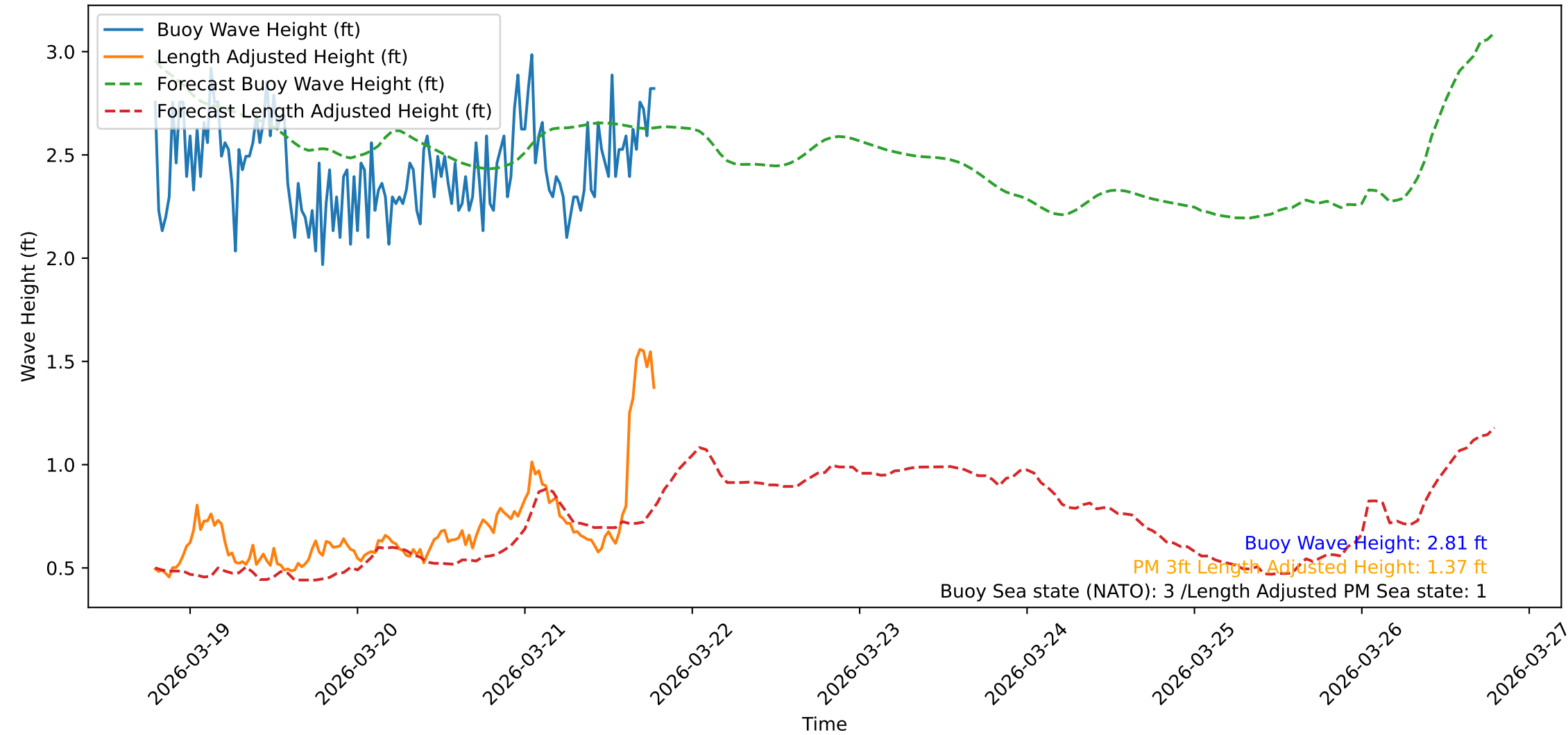
Wave Heights over Time for Oceanside Harbor at 2026-03-21 19:10:31
