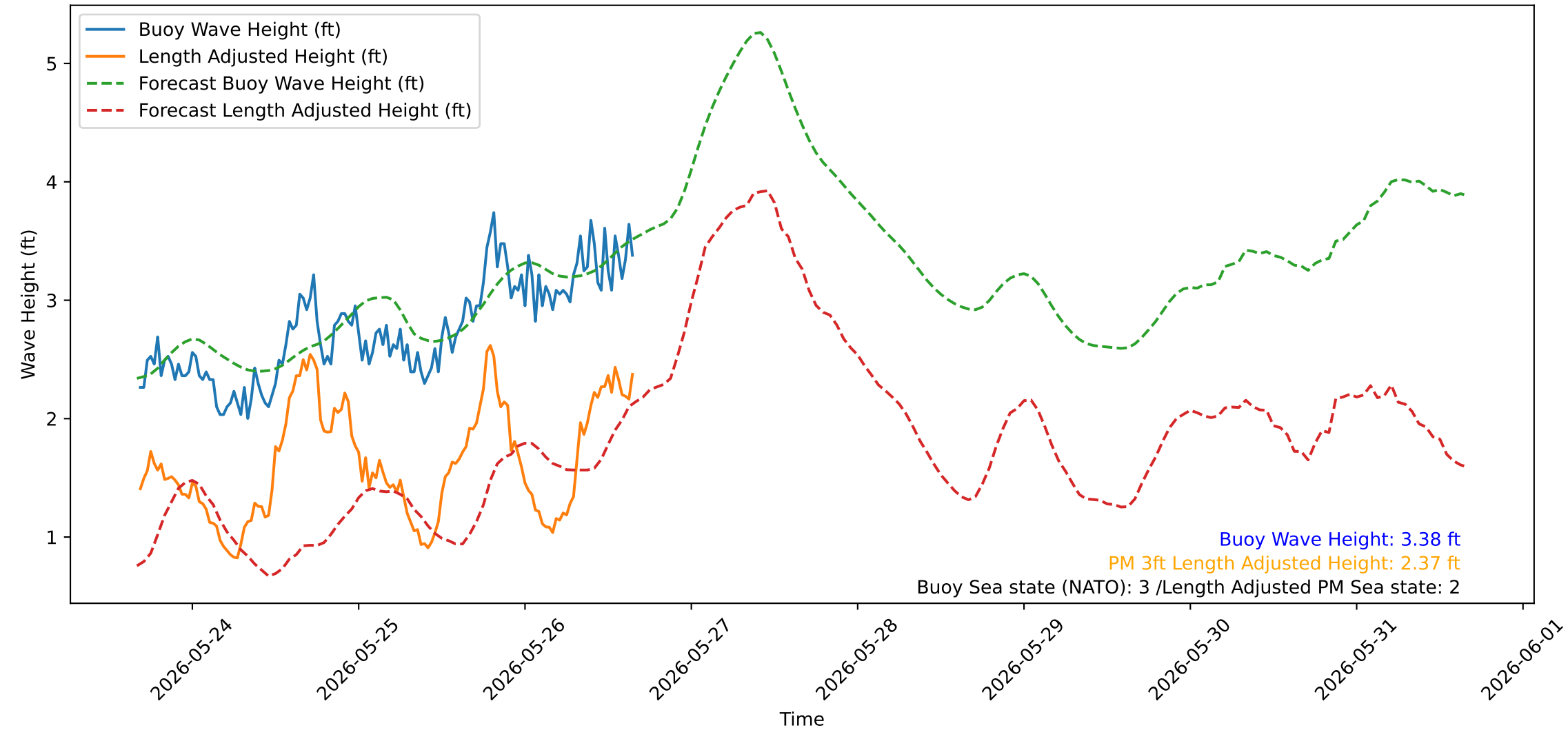
Wave Heights over Time for Red Beach at 2026-05-26 16:10:47
