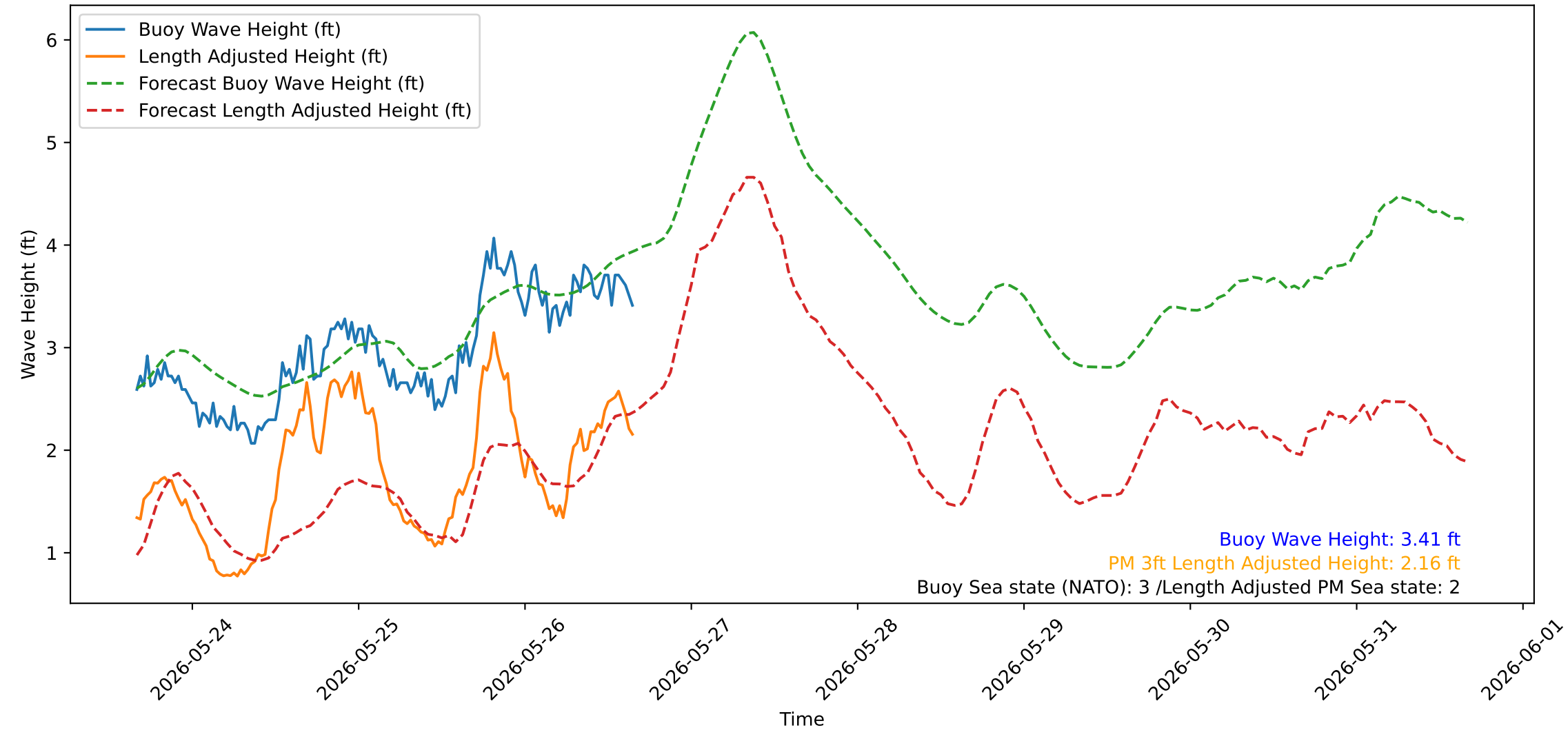
Wave Heights over Time for Green Beach at 2026-05-26 16:11:10
