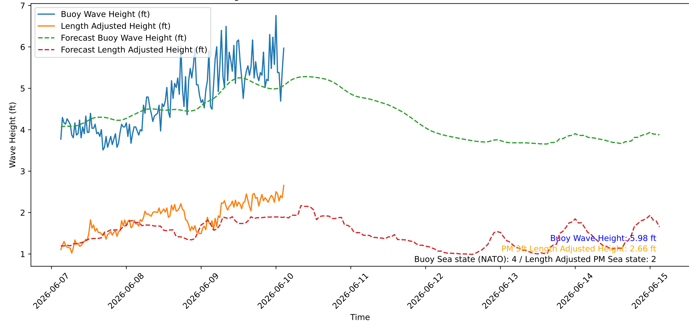
Wave Heights over Time for Oceanside Harbor at 2026-06-10 03:10:26
