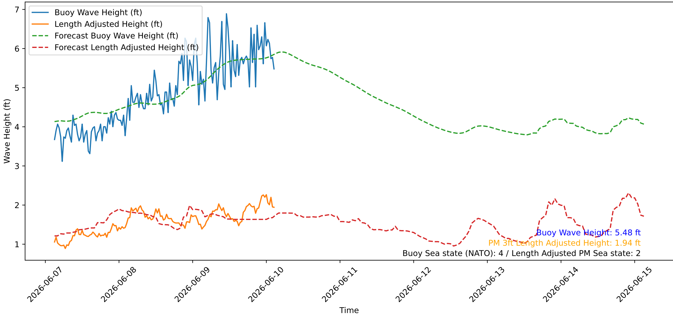
Wave Heights over Time for Green Beach at 2026-06-10 03:11:09
