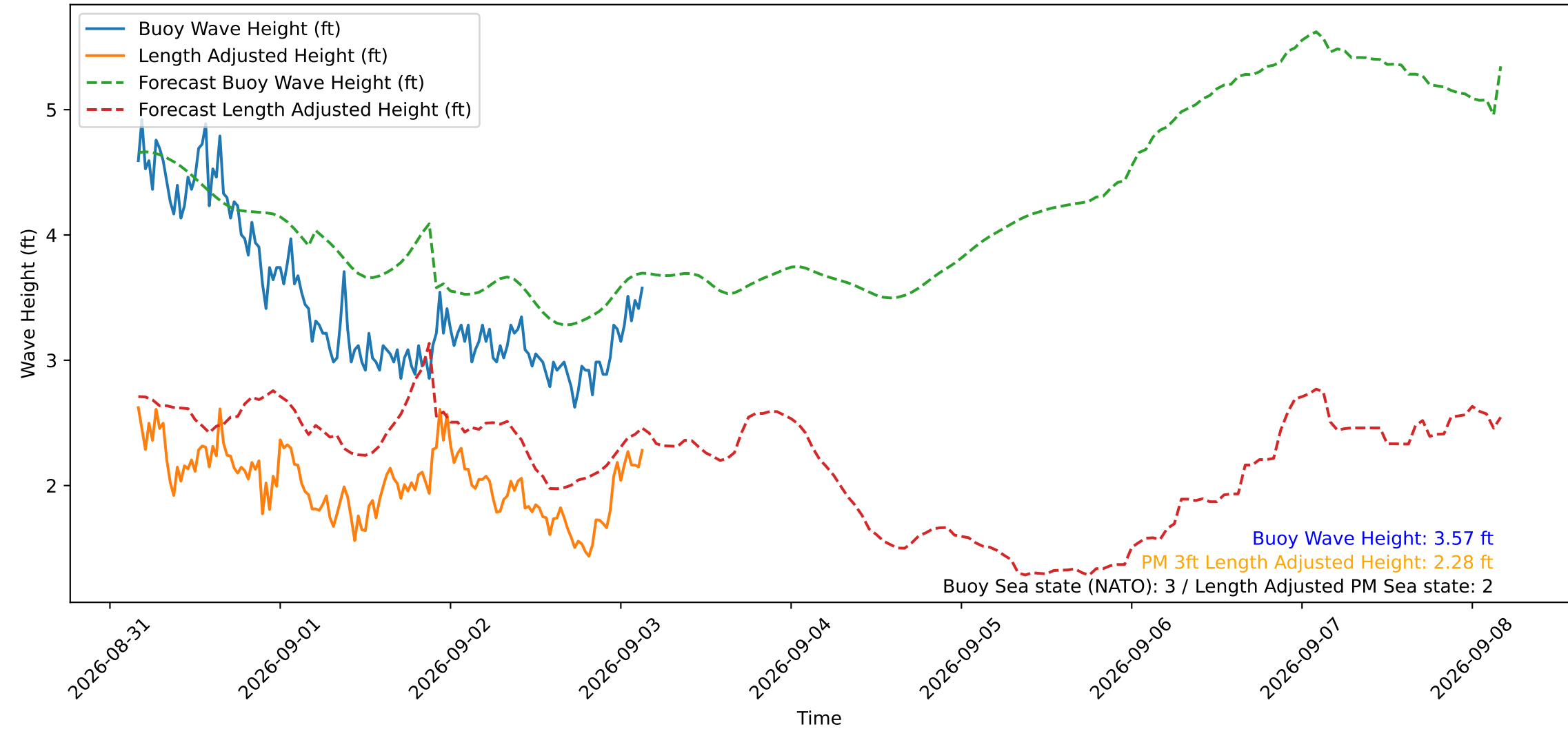
Wave Heights over Time for Oceanside Harbor at 2026-09-03 03:50:29
