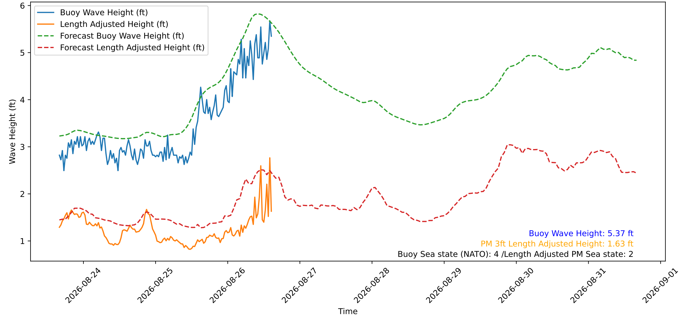
Wave Heights over Time for Green Beach at 2026-08-26 15:41:11
