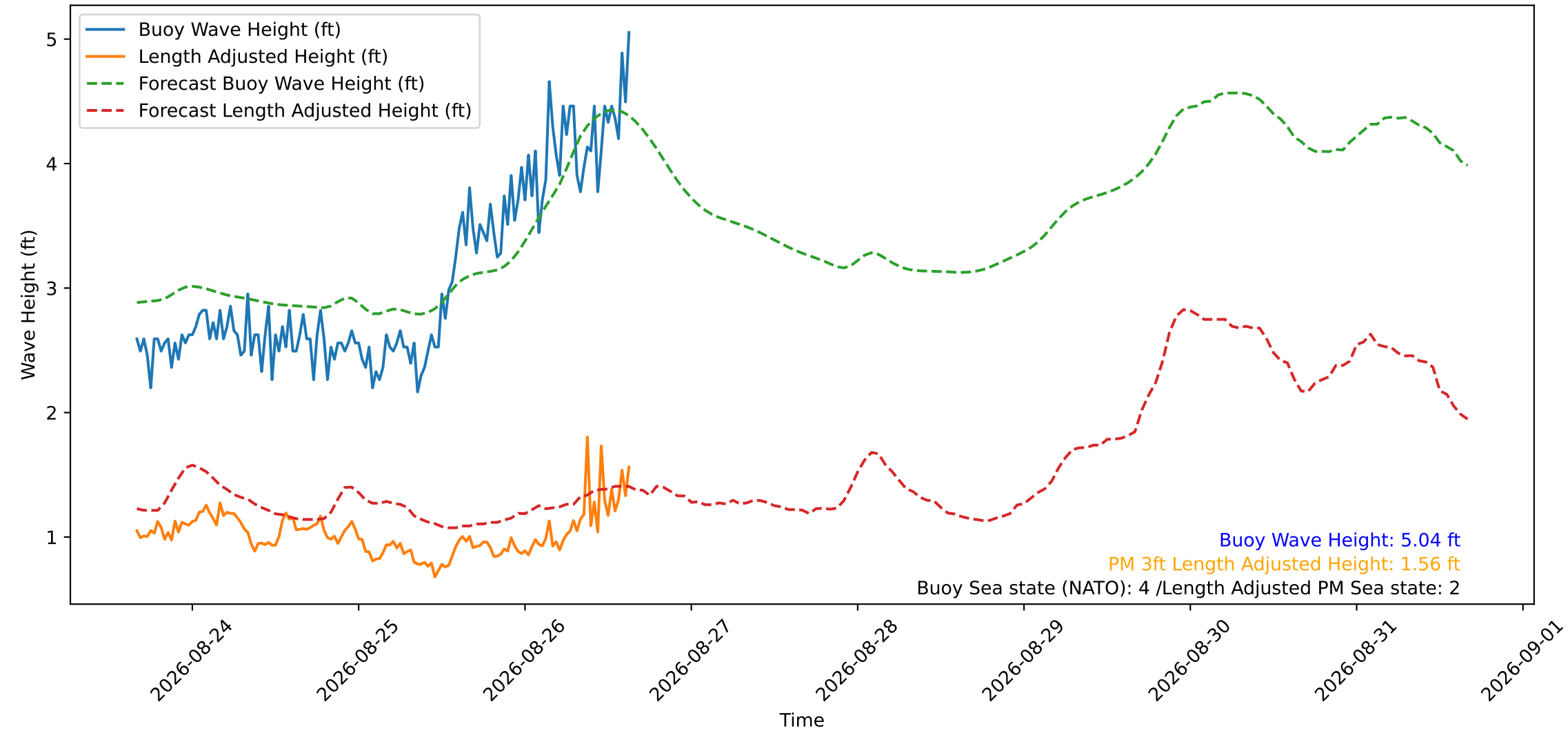
Wave Heights over Time for Red Beach at 2026-08-26 15:40:49
