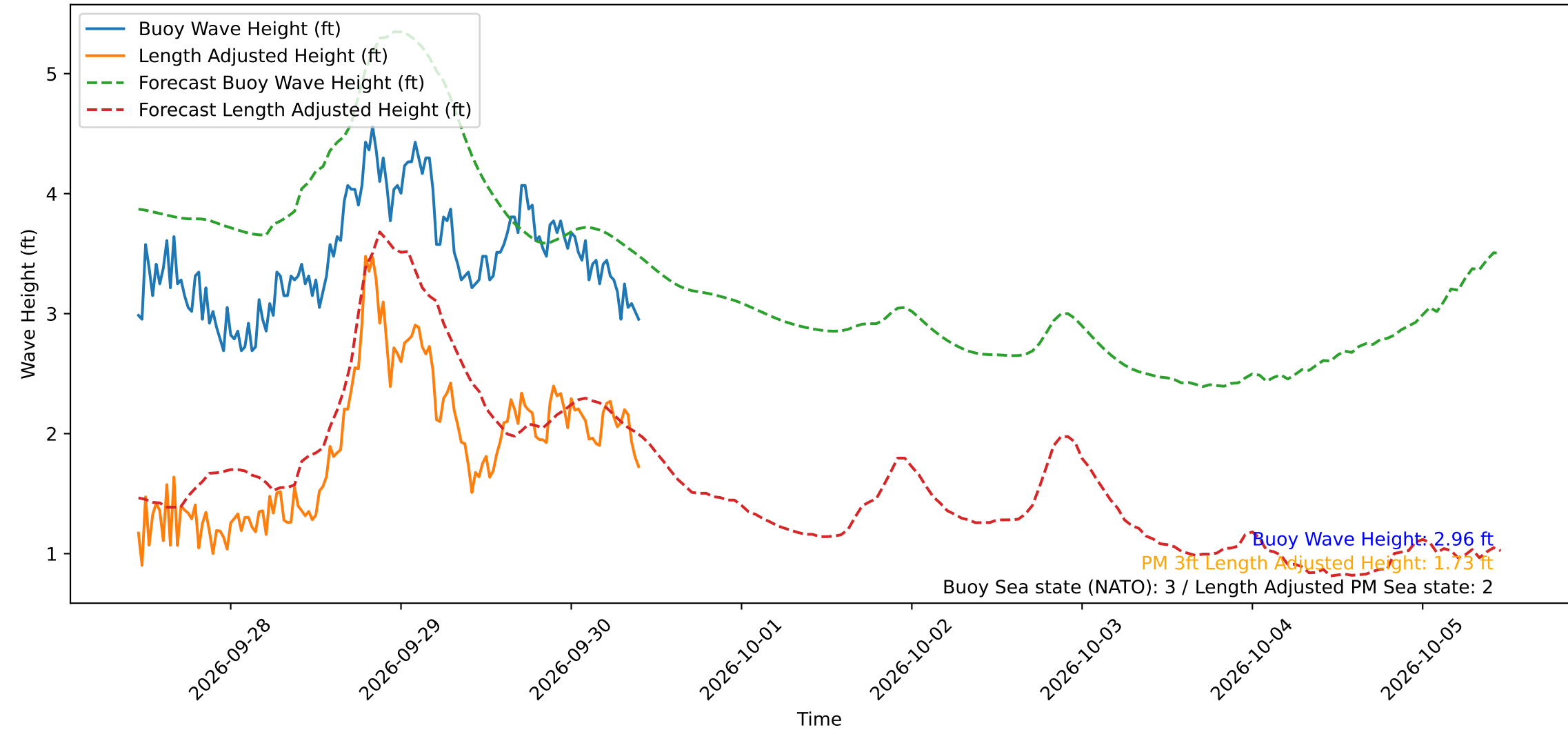
Wave Heights over Time for Green Beach at 2026-09-30 10:31:12
