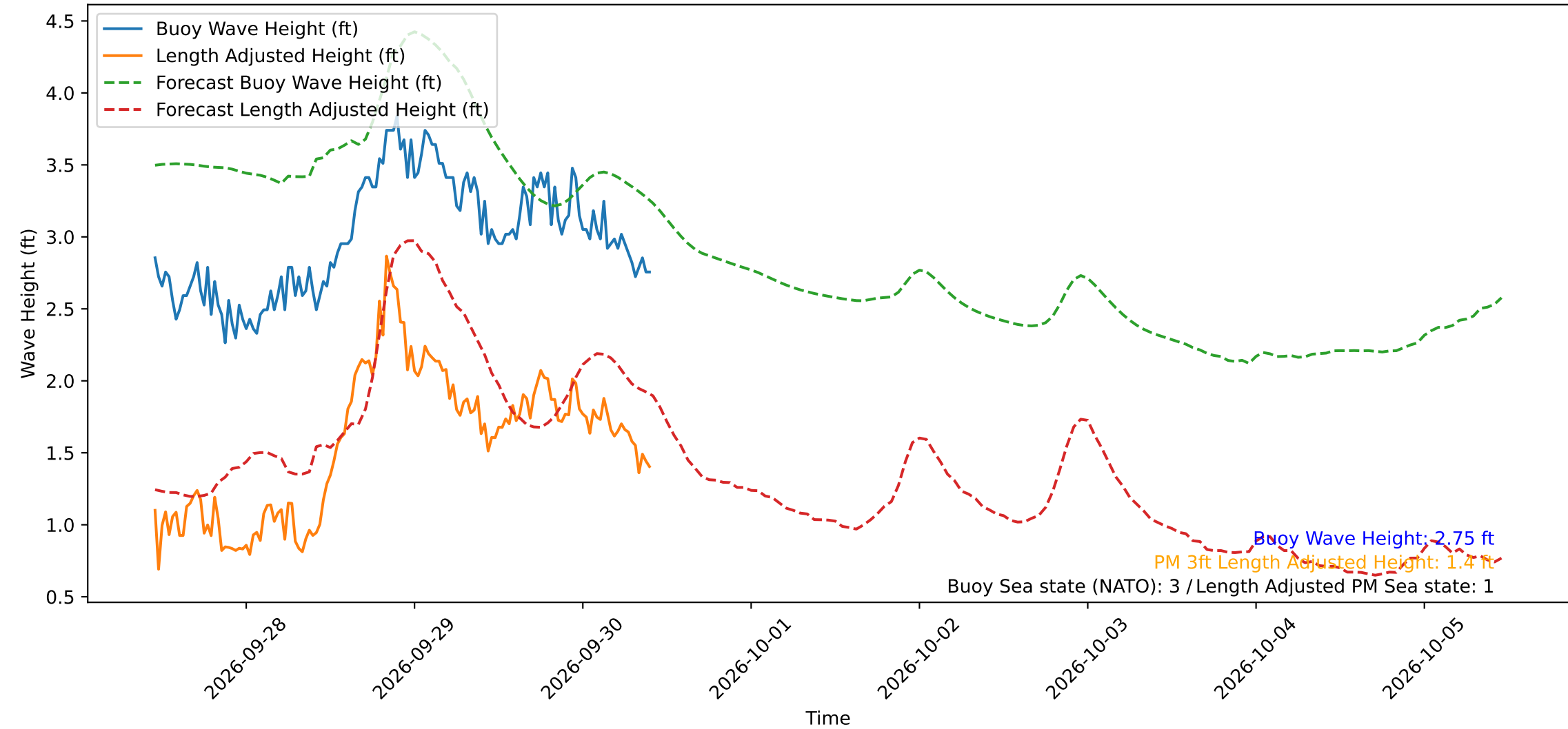
Wave Heights over Time for Red Beach at 2026-09-30 10:30:49
