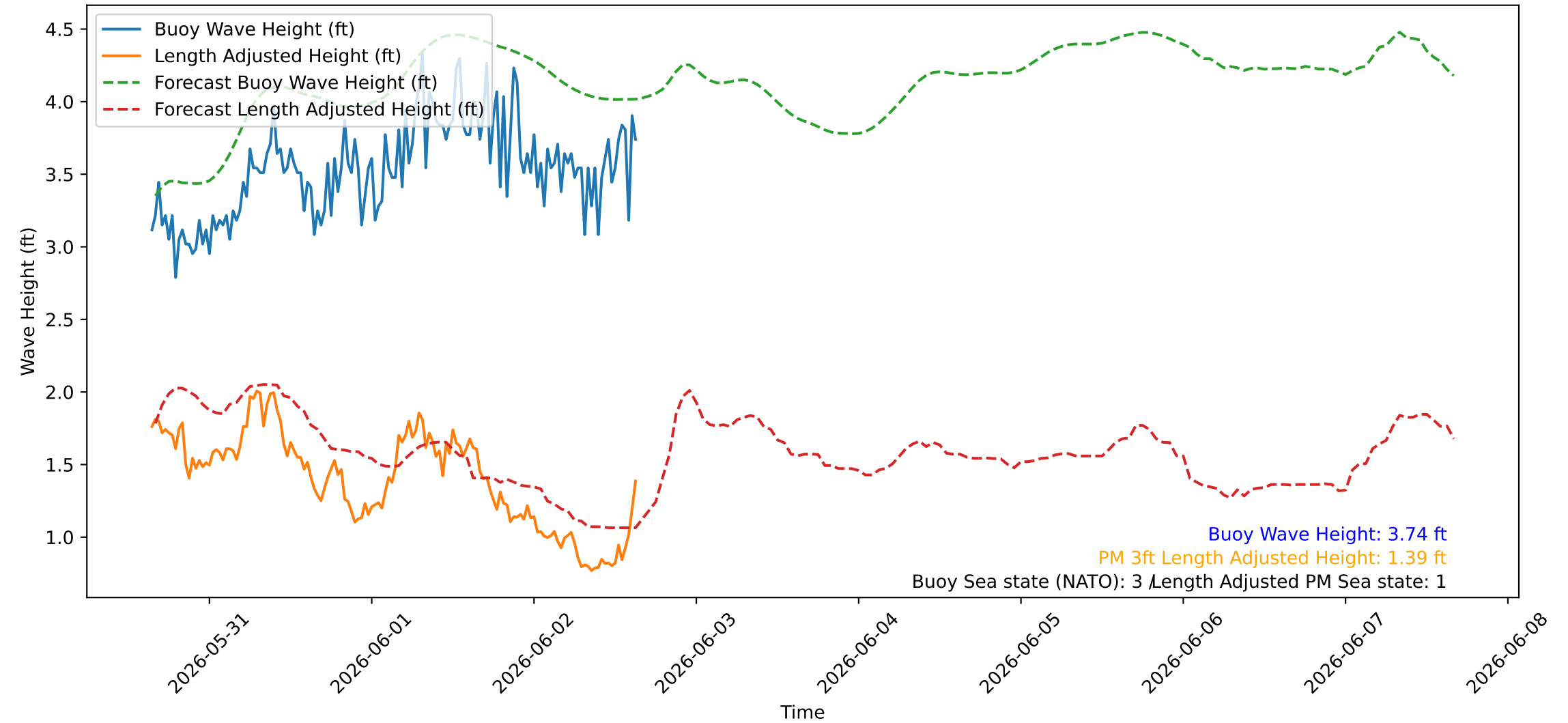
Wave Heights over Time for Green Beach at 2026-06-02 15:41:07
