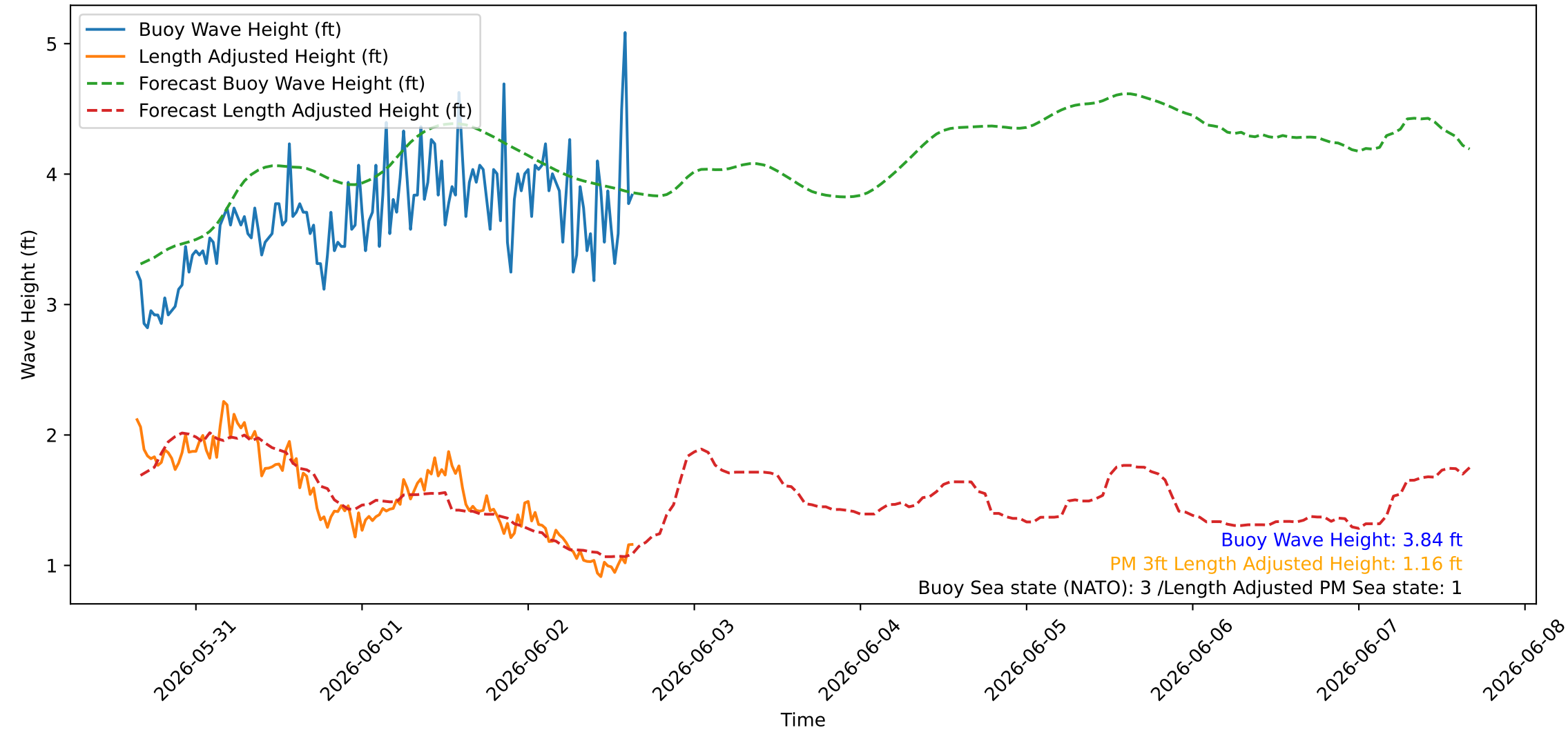
Wave Heights over Time for Oceanside Harbor at 2026-06-02 15:40:26
