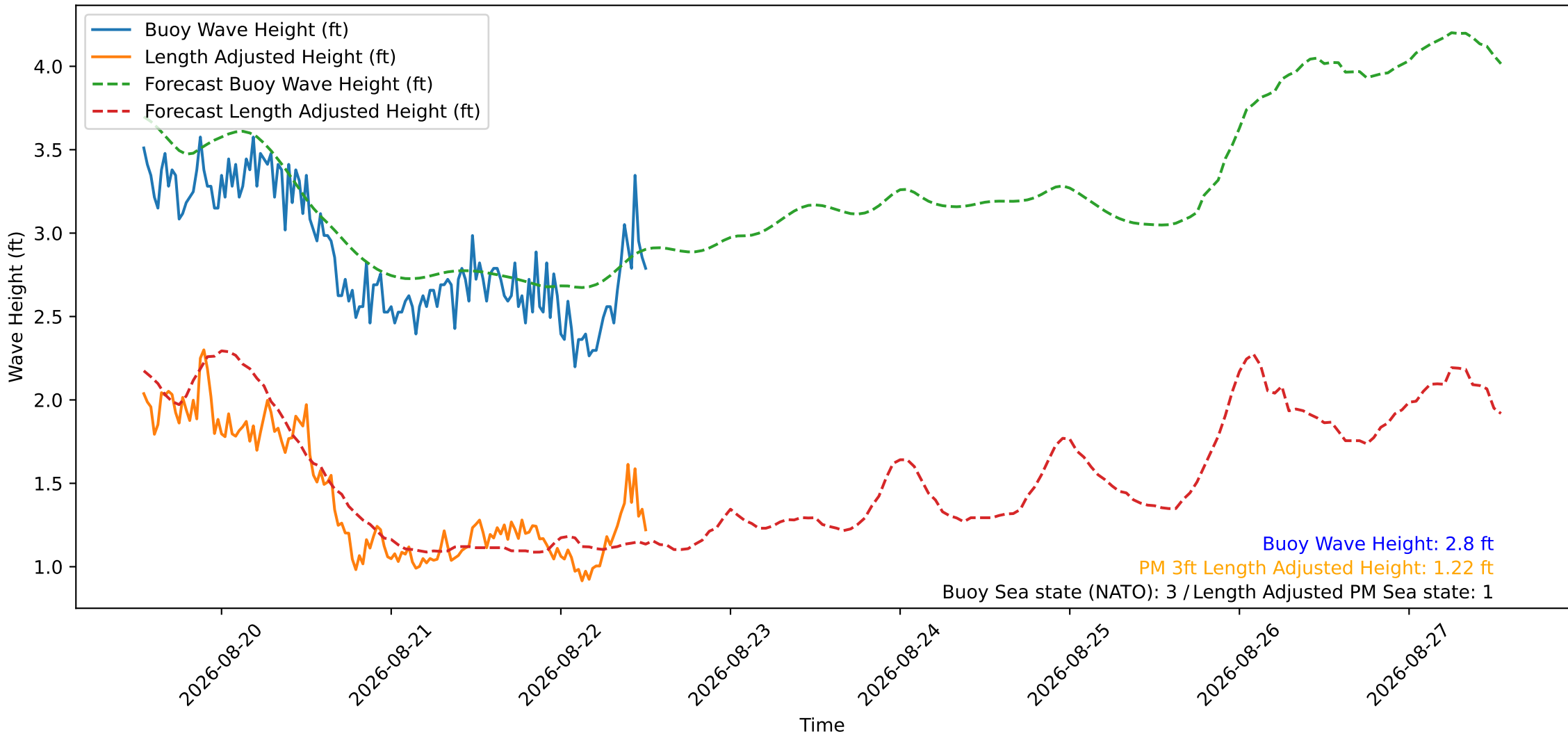
Wave Heights over Time for Oceanside Harbor at 2026-08-22 12:50:30
