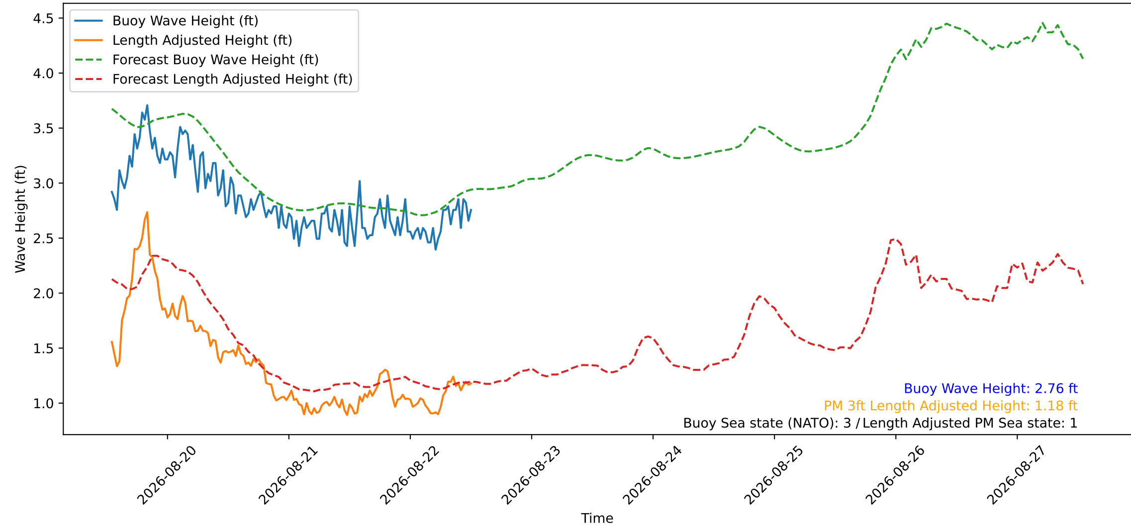
Wave Heights over Time for Green Beach at 2026-08-22 12:51:14
