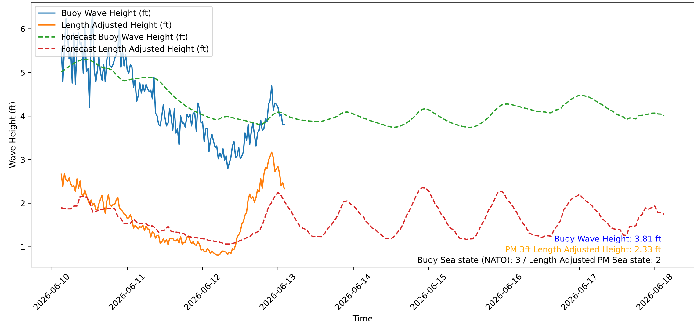
Wave Heights over Time for Oceanside Harbor at 2026-06-13 03:00:26
