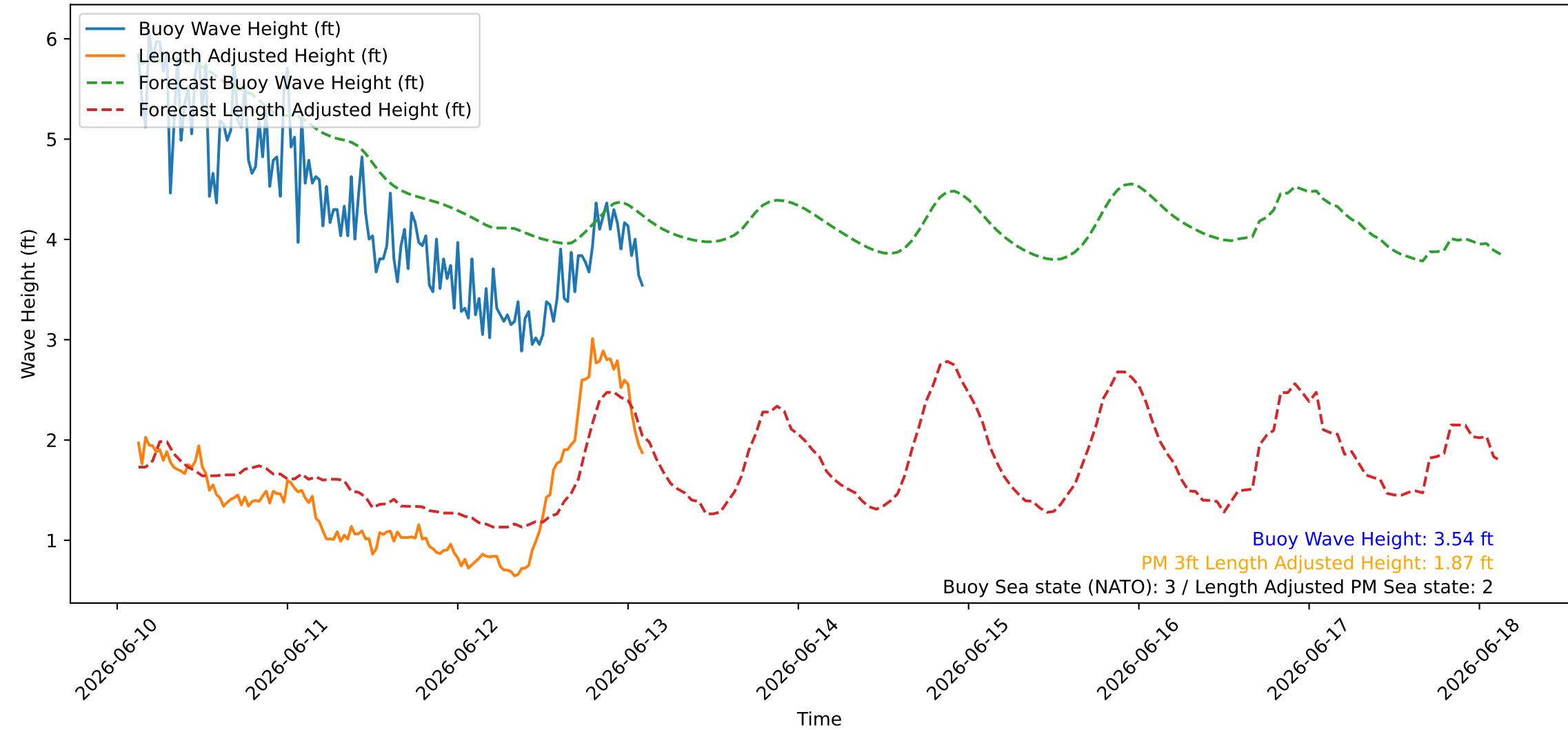
Wave Heights over Time for Green Beach at 2026-06-13 03:01:08
