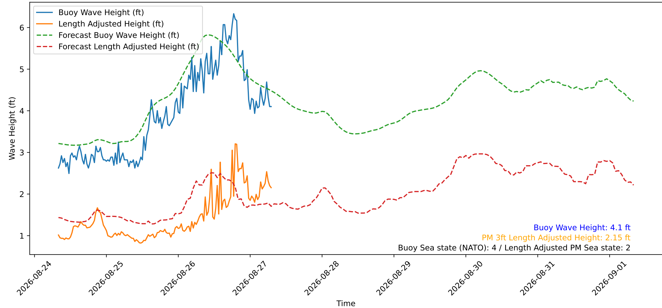
Wave Heights over Time for Green Beach at 2026-08-27 07:41:13
