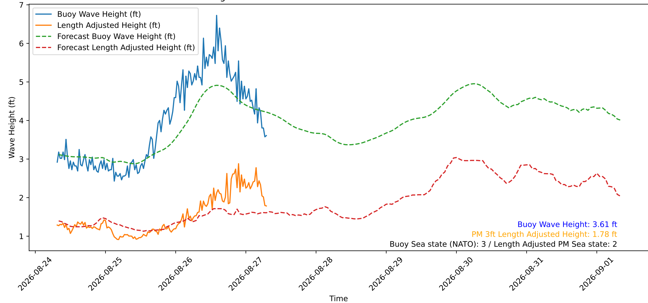
Wave Heights over Time for Oceanside Harbor at 2026-08-27 07:40:30
