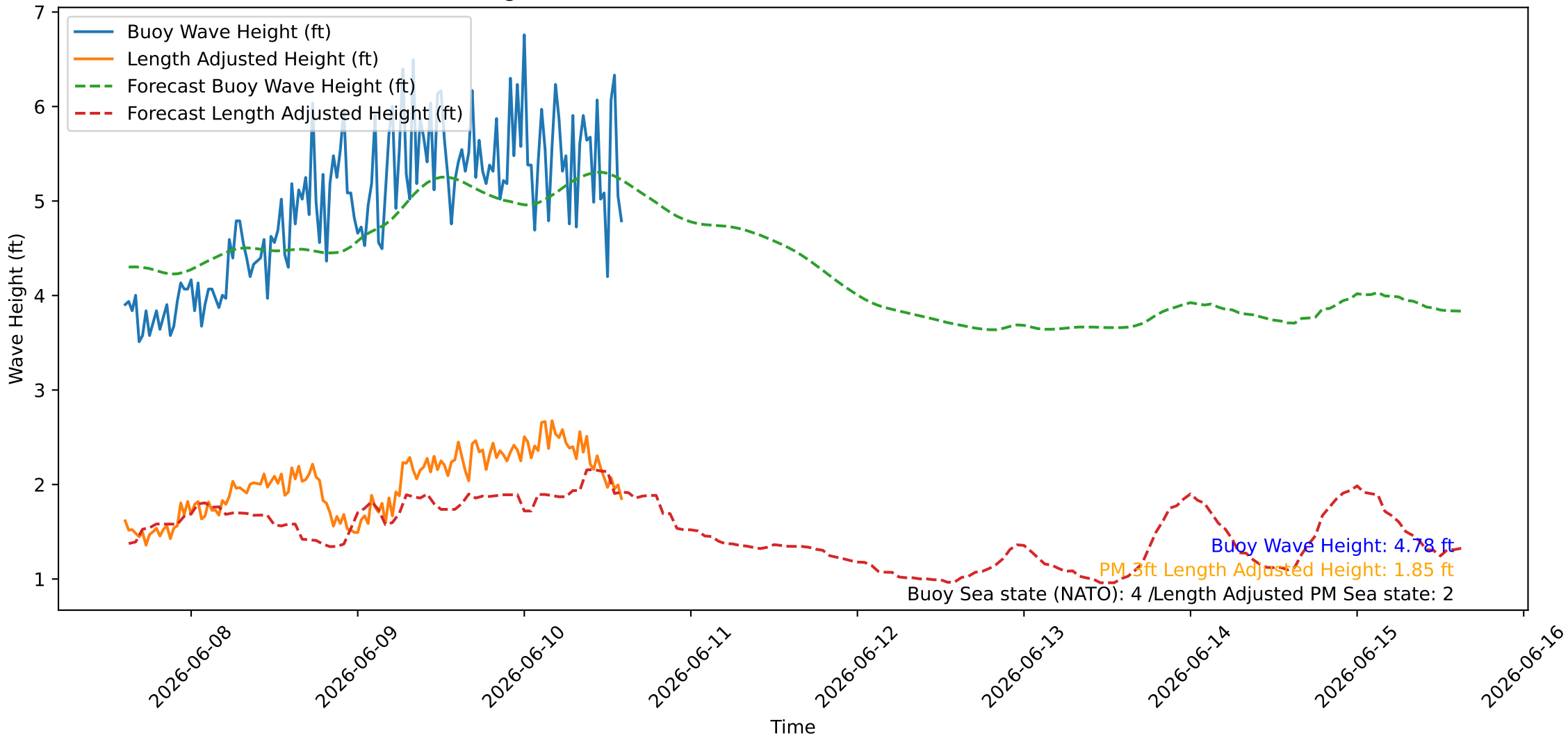
Wave Heights over Time for Oceanside Harbor at 2026-06-10 14:40:27
