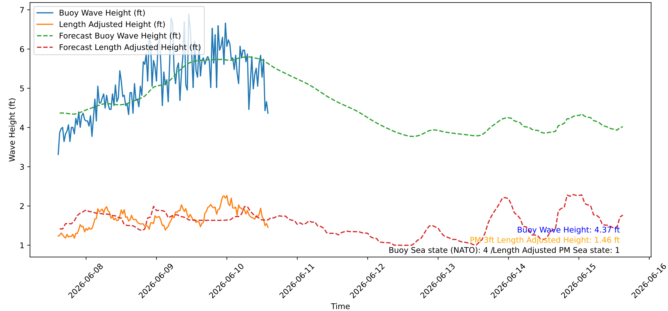
Wave Heights over Time for Green Beach at 2026-06-10 14:41:10
