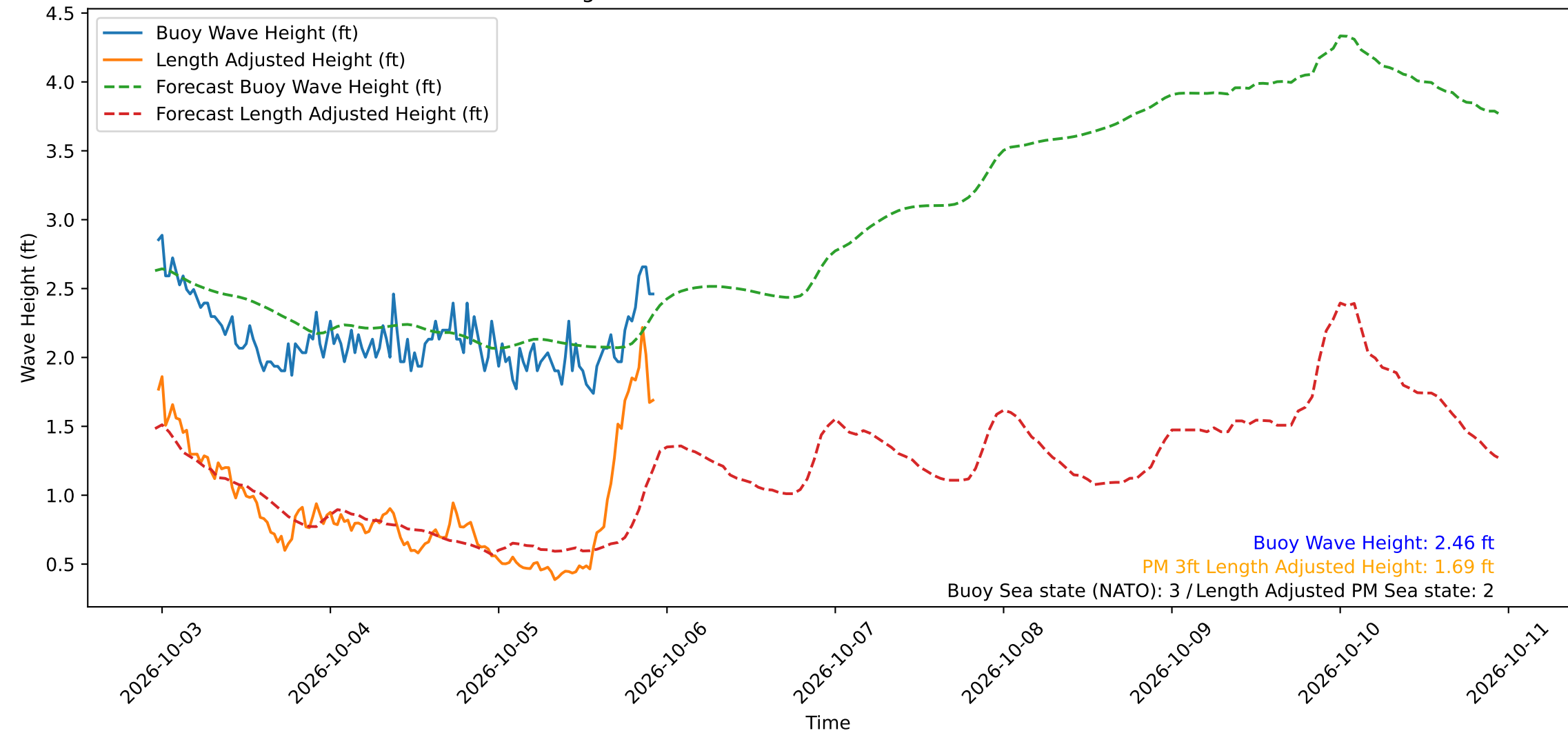
Wave Heights over Time for Red Beach at 2026-10-05 23:00:49
