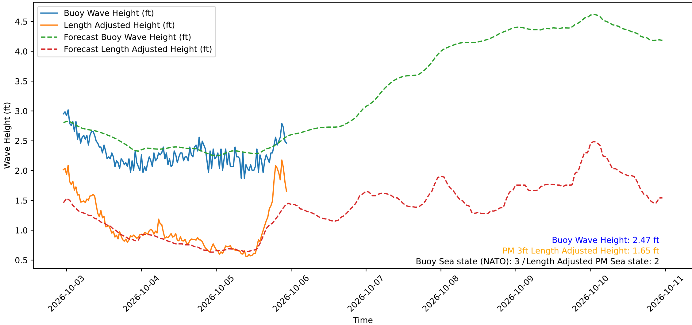
Wave Heights over Time for Oceanside Harbor at 2026-10-05 23:00:29
