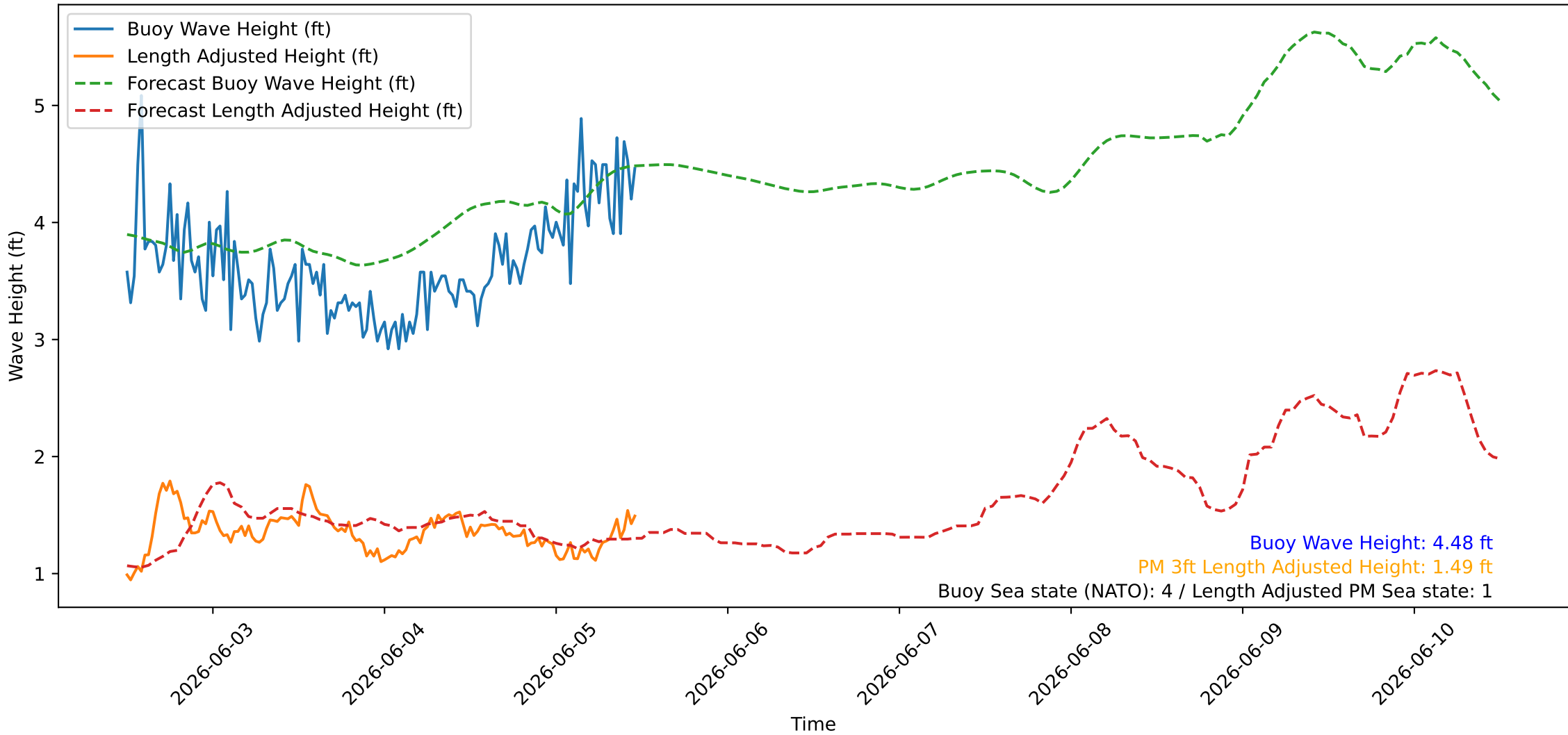
Wave Heights over Time for Oceanside Harbor at 2026-06-05 11:50:26
