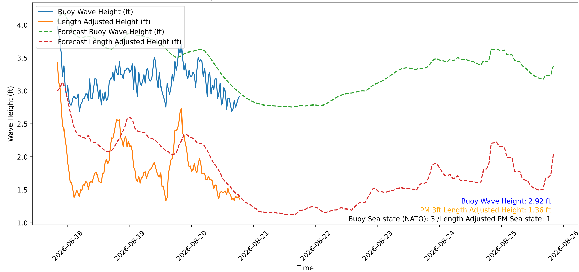
Wave Heights over Time for Green Beach at 2026-08-20 19:31:08
