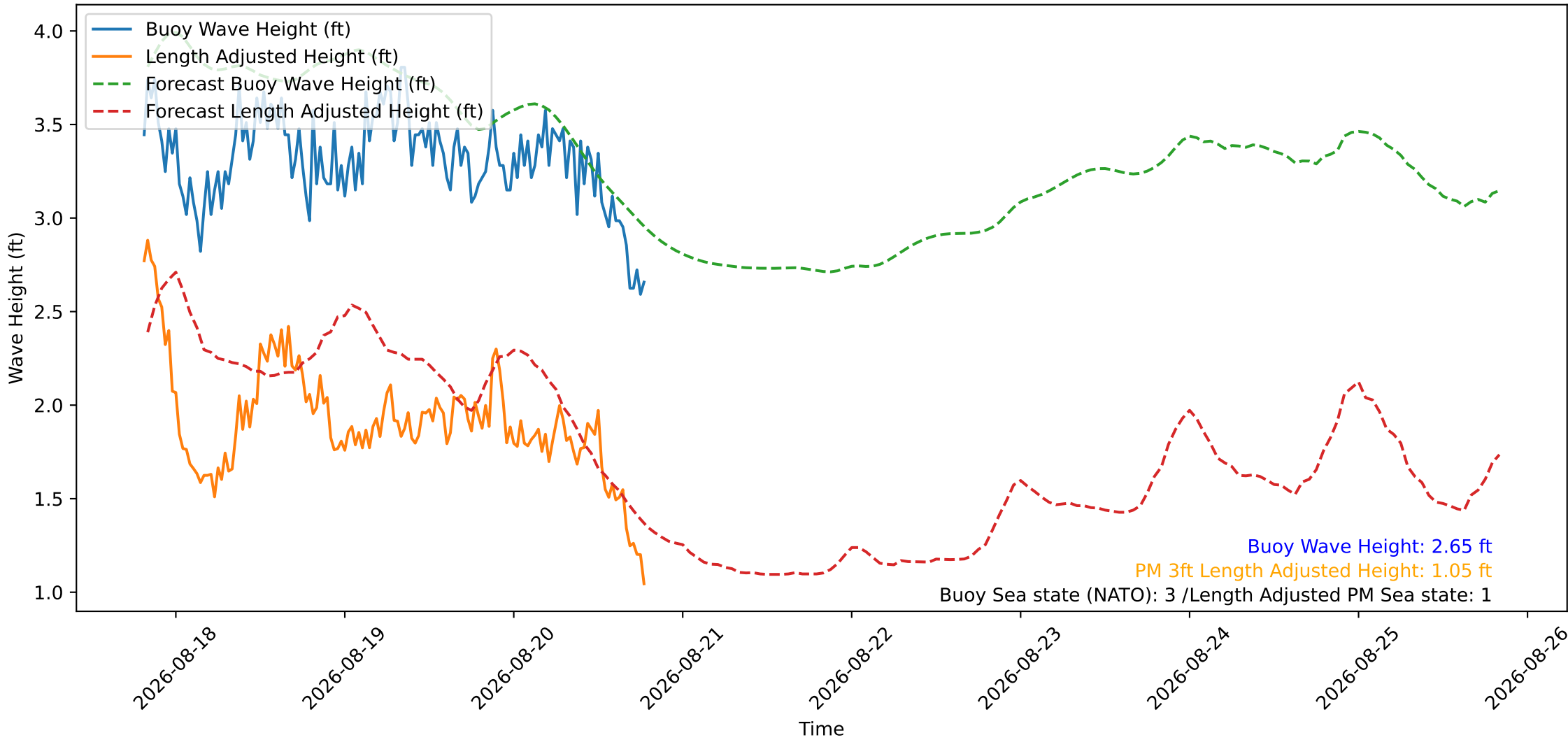
Wave Heights over Time for Oceanside Harbor at 2026-08-20 19:30:26
