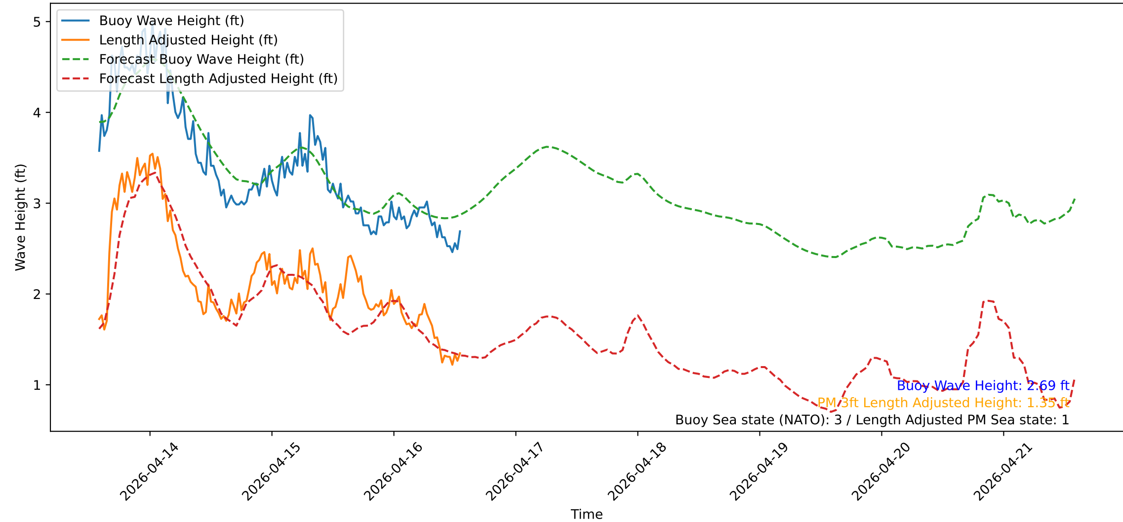
Wave Heights over Time for Green Beach at 2026-04-16 14:01:13
