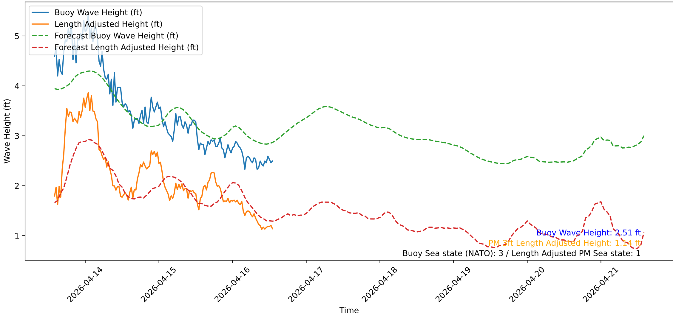
Wave Heights over Time for Oceanside Harbor at 2026-04-16 14:00:31
