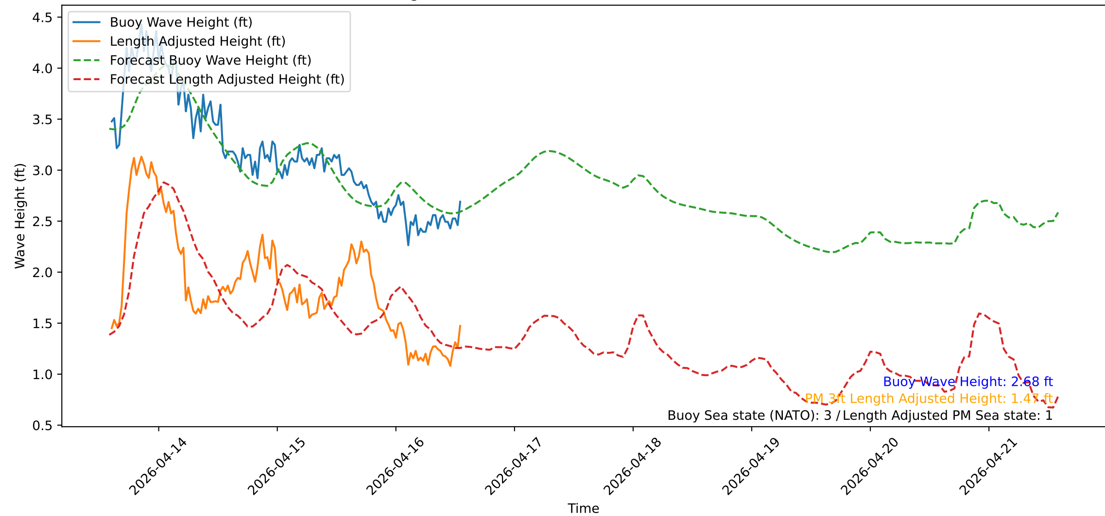
Wave Heights over Time for Red Beach at 2026-04-16 14:00:50
