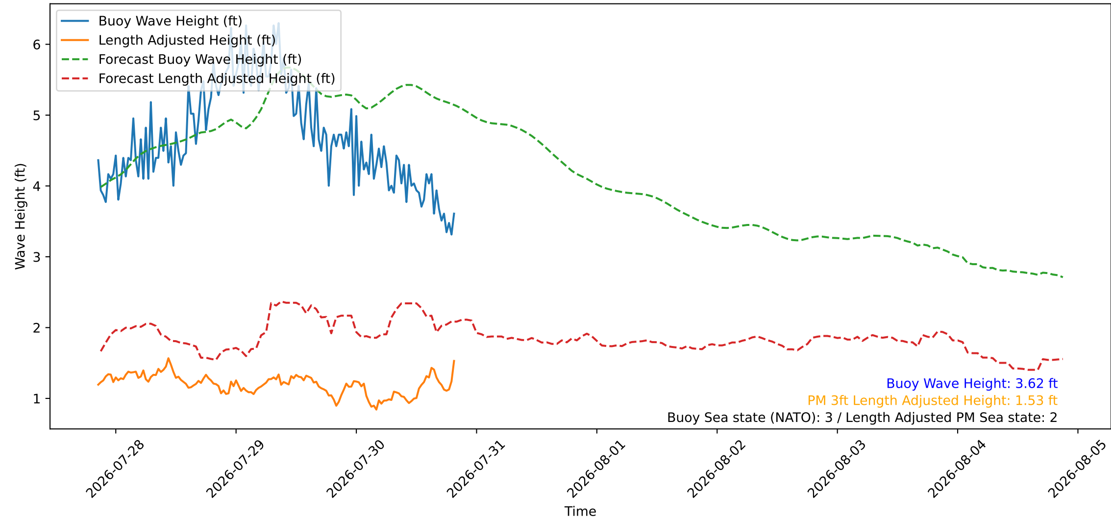
Wave Heights over Time for Green Beach at 2026-07-30 20:31:09
