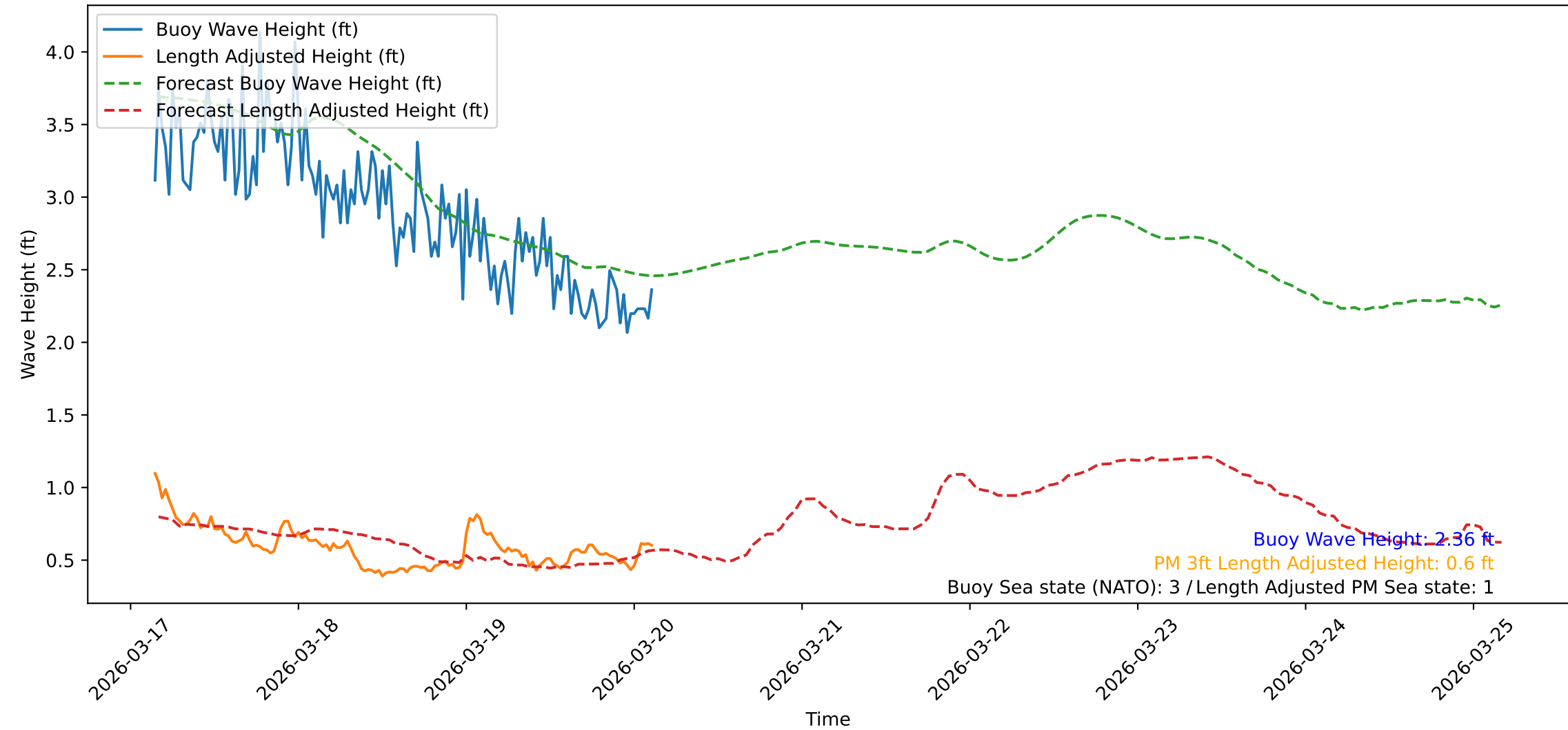
Wave Heights over Time for Green Beach at 2026-03-20 03:31:09
