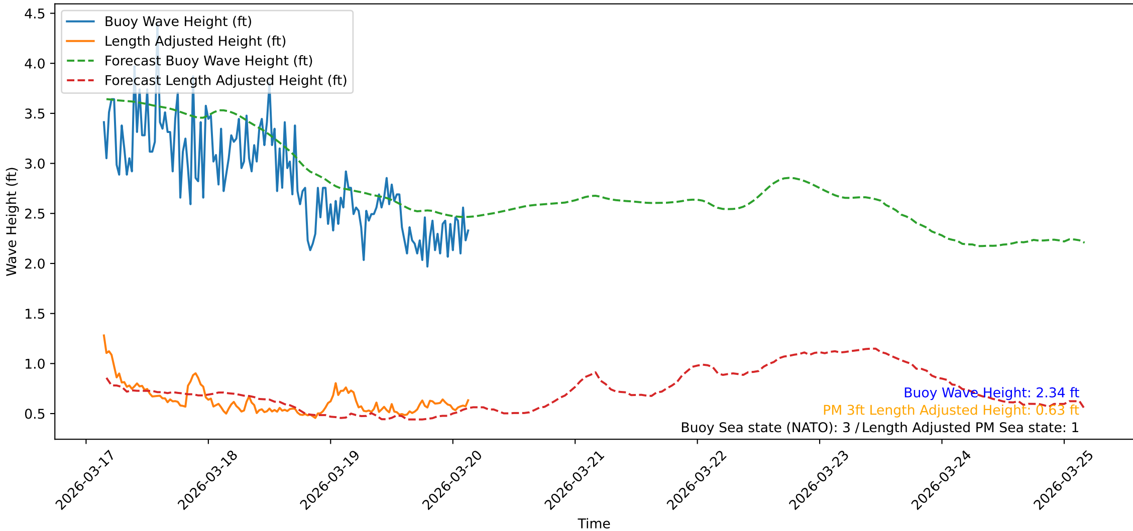
Wave Heights over Time for Oceanside Harbor at 2026-03-20 03:30:31
