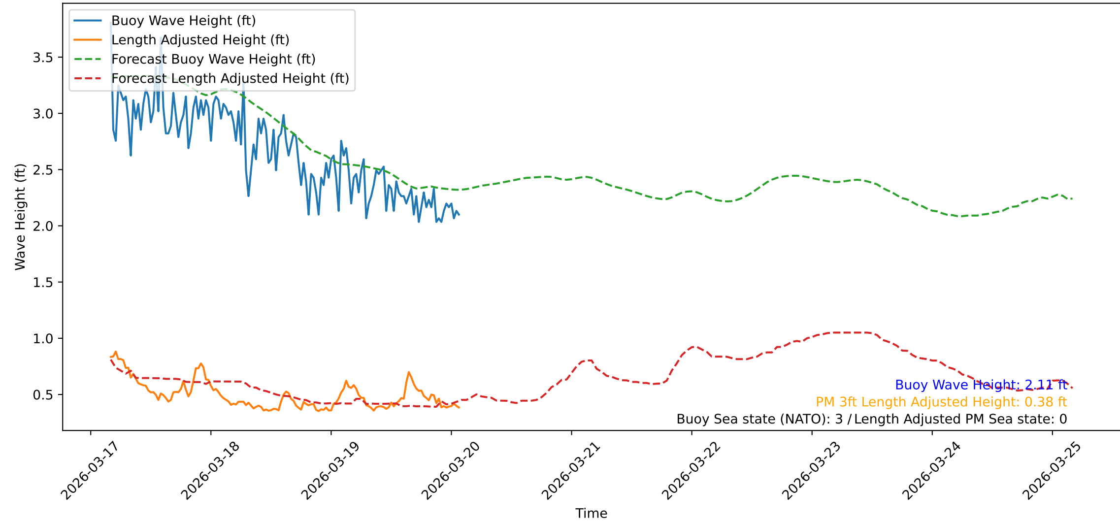
Wave Heights over Time for Red Beach at 2026-03-20 03:30:47
