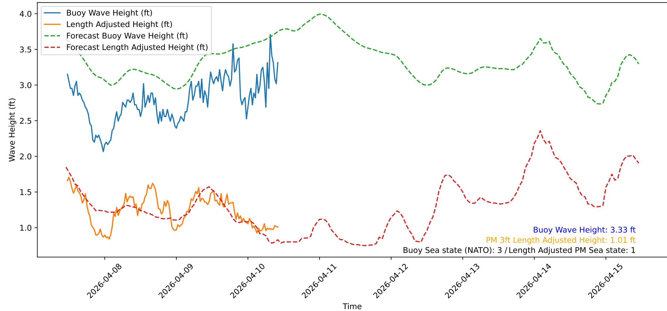
Wave Heights over Time for Red Beach at 2026-04-10 11:00:50
