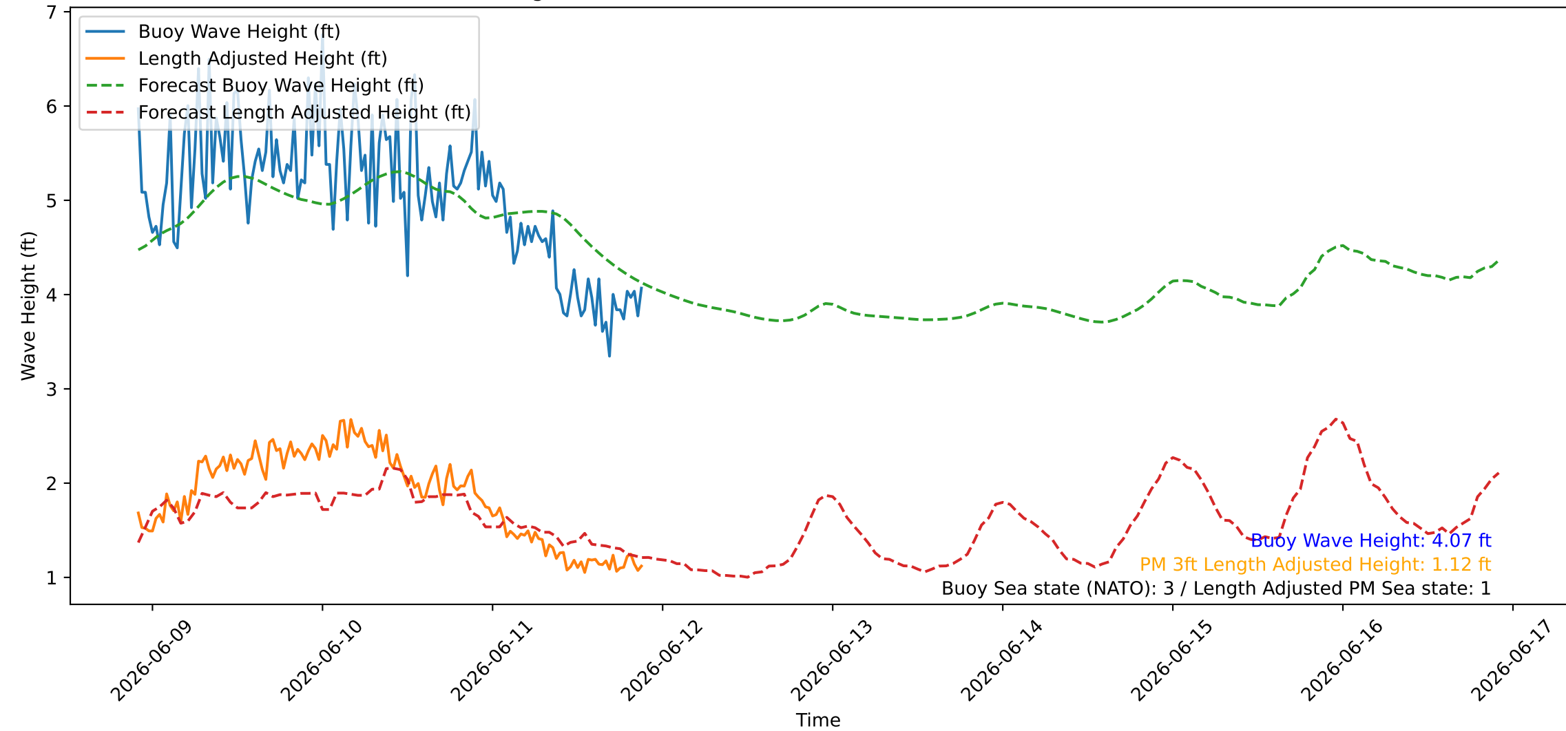
Wave Heights over Time for Oceanside Harbor at 2026-06-11 21:50:26
