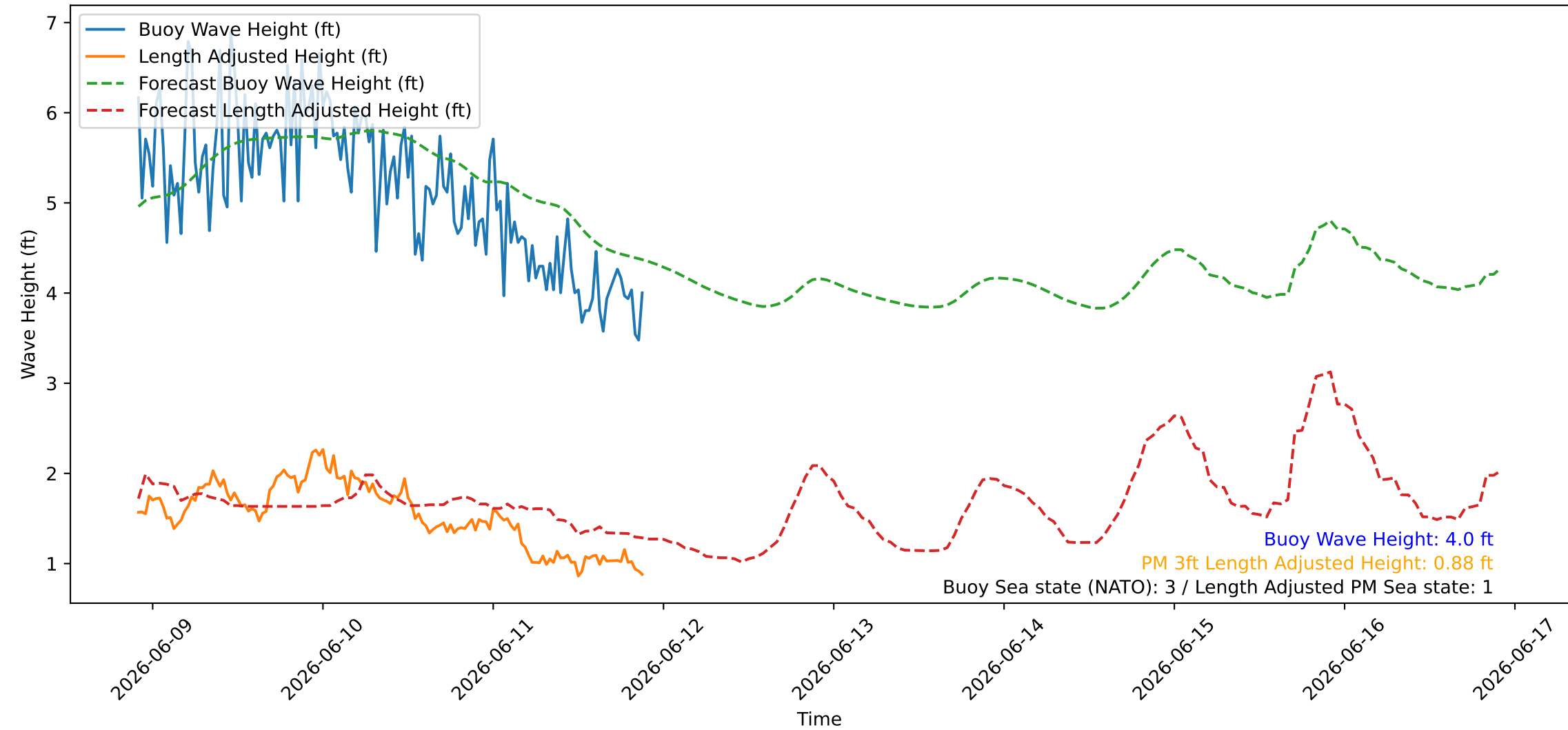
Wave Heights over Time for Green Beach at 2026-06-11 21:51:09
