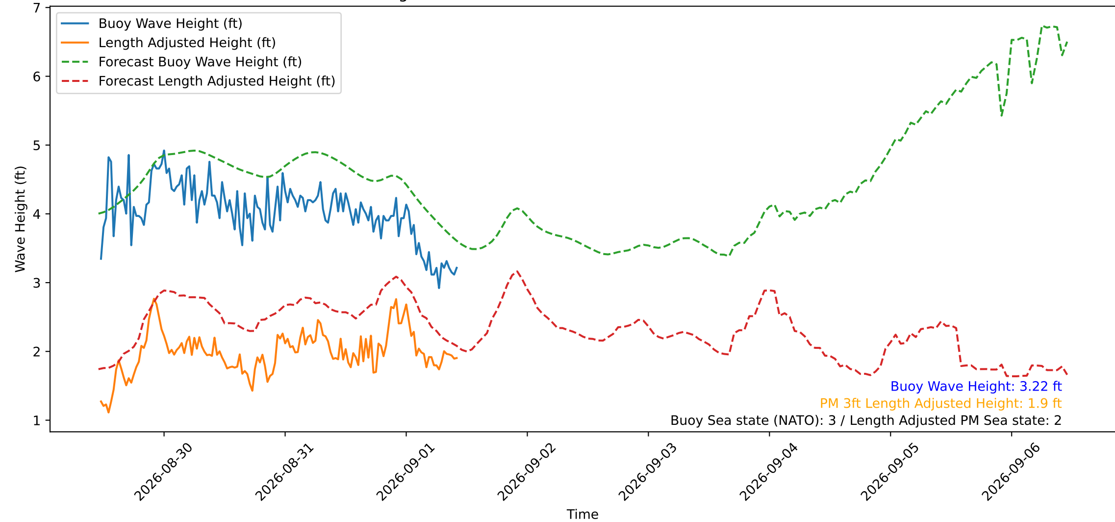
Wave Heights over Time for Green Beach at 2026-09-01 11:01:12
