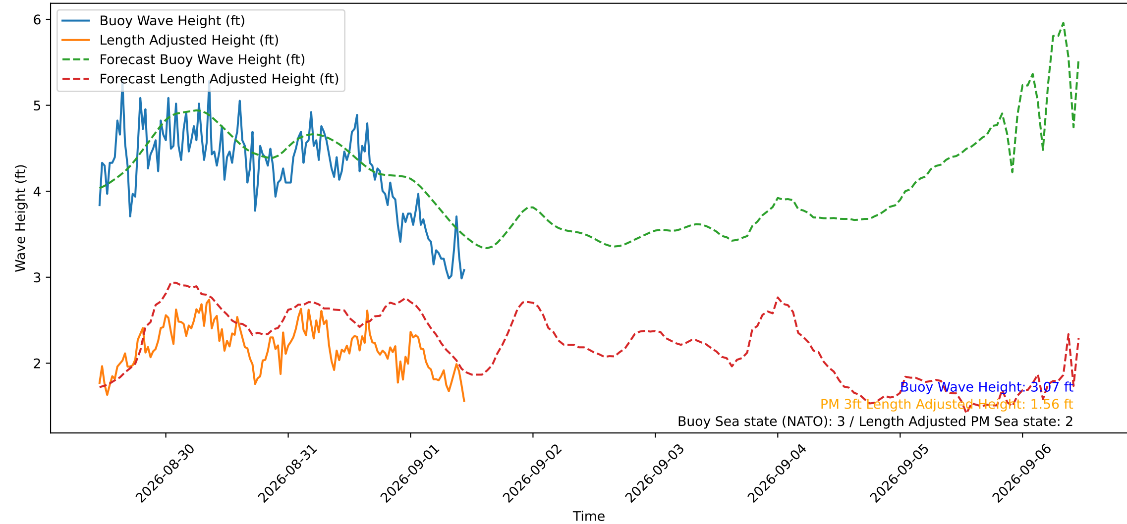
Wave Heights over Time for Oceanside Harbor at 2026-09-01 11:00:30
