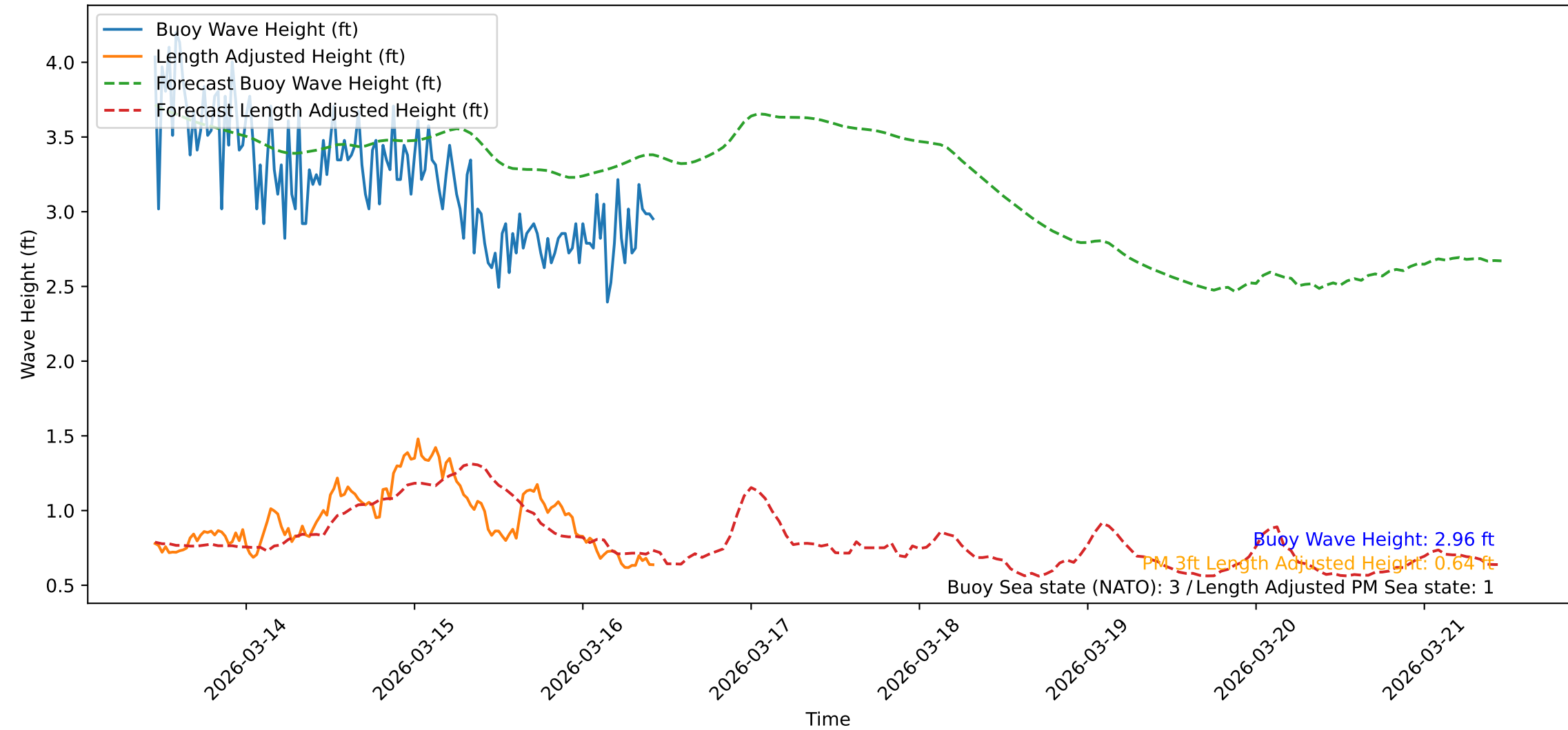
Wave Heights over Time for Oceanside Harbor at 2026-03-16 11:10:43
