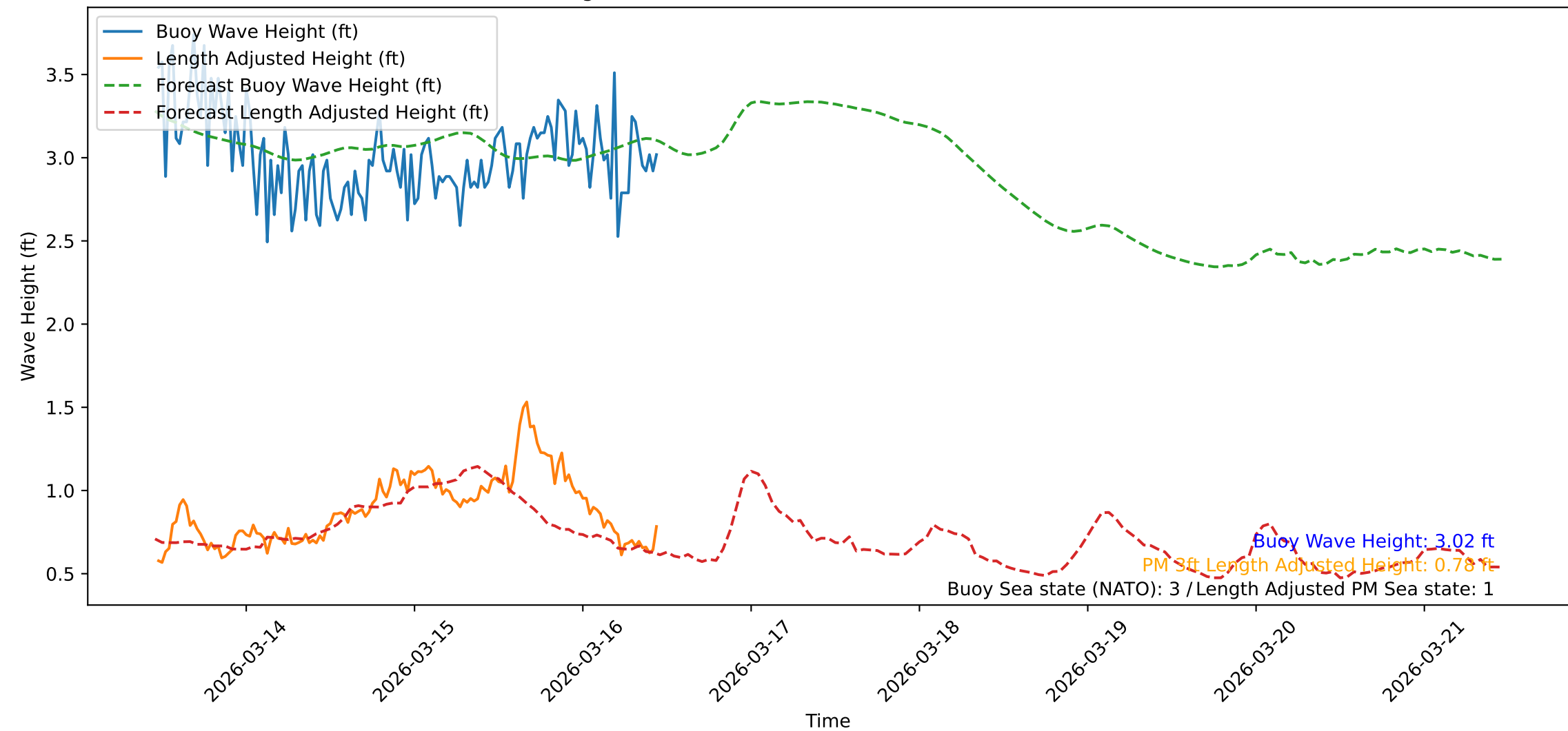
Wave Heights over Time for Red Beach at 2026-03-16 11:11:06
