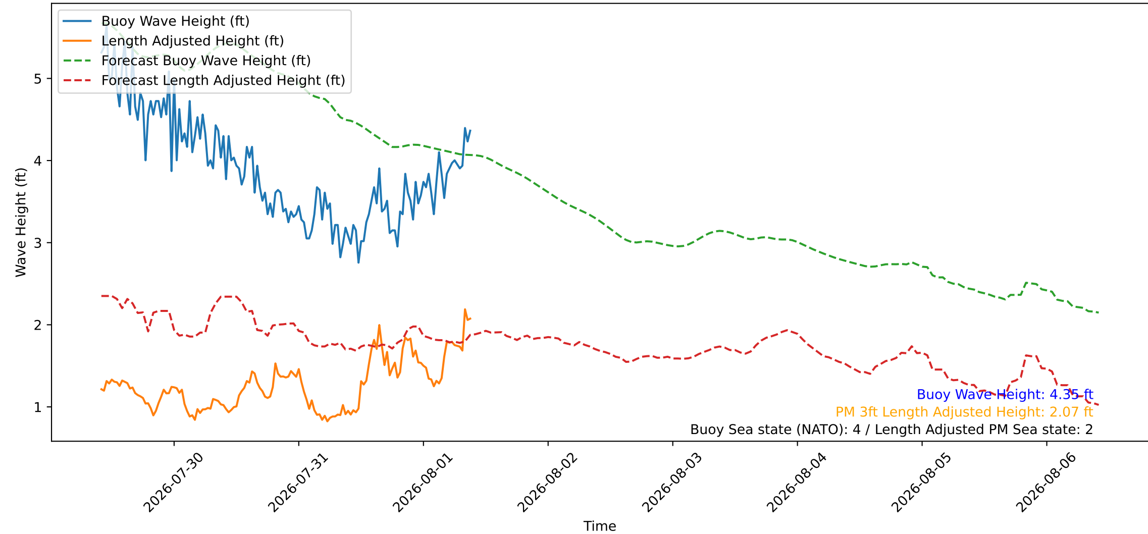
Wave Heights over Time for Green Beach at 2026-08-01 09:51:10
