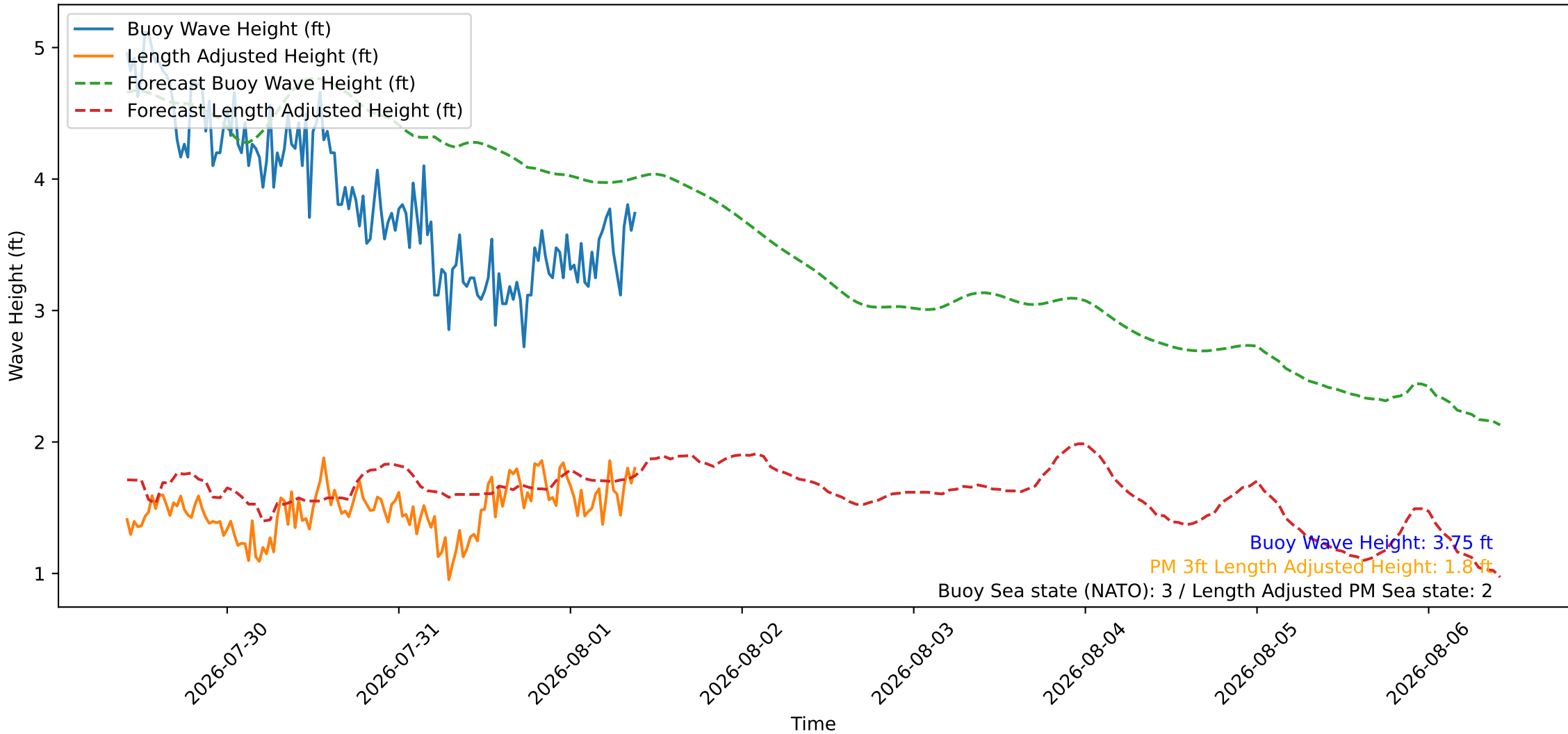
Wave Heights over Time for Oceanside Harbor at 2026-08-01 09:50:26
