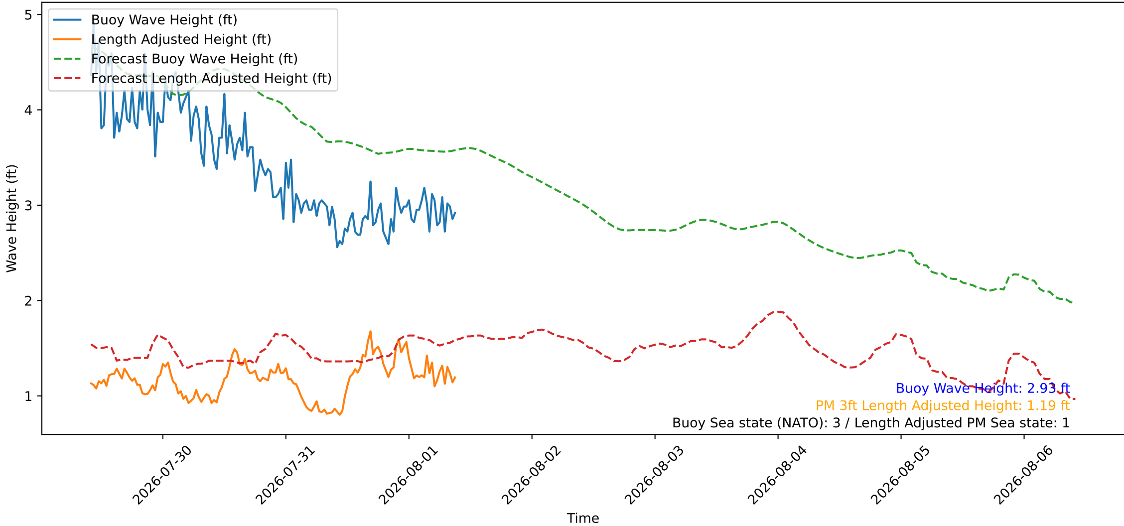
Wave Heights over Time for Red Beach at 2026-08-01 09:50:47
