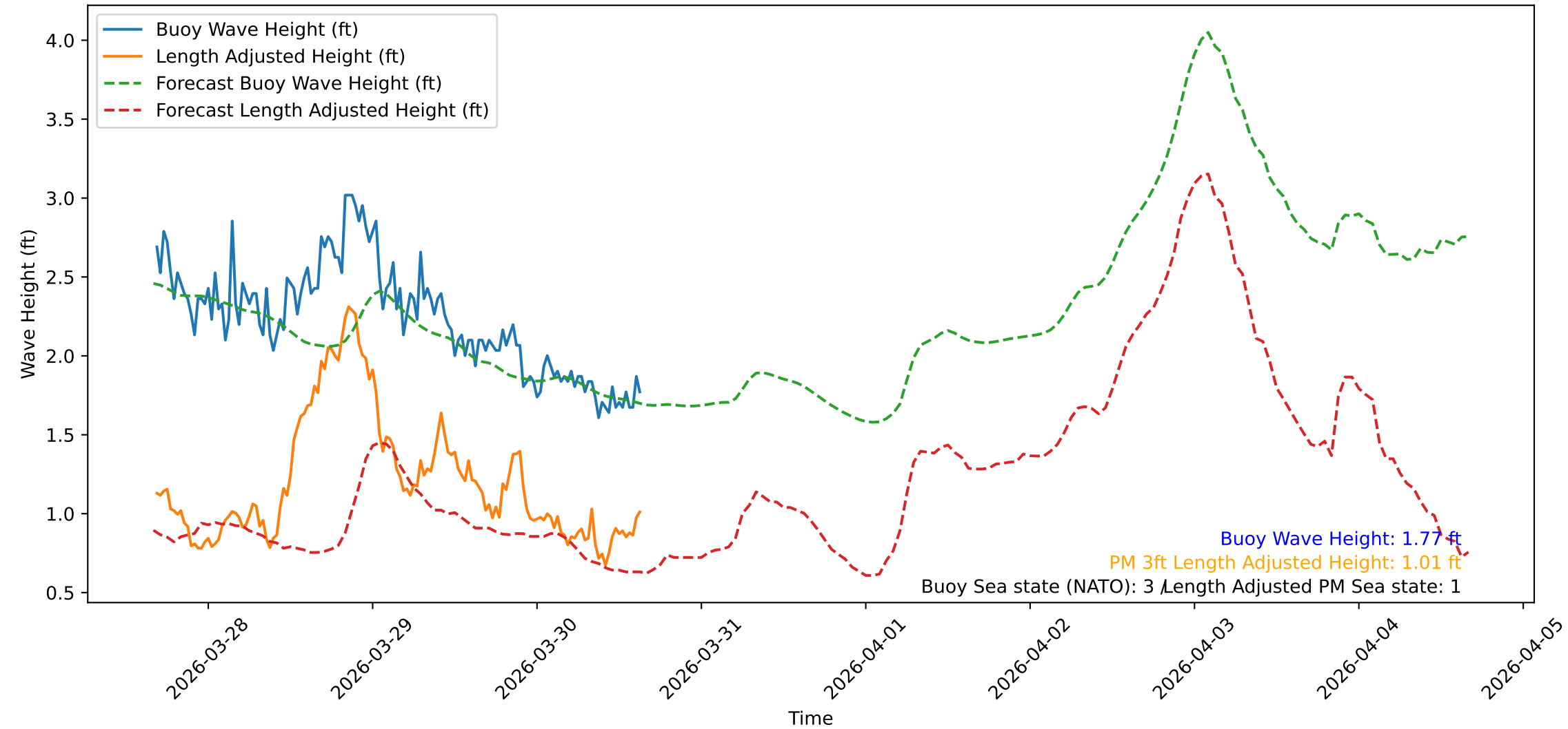
Wave Heights over Time for Red Beach at 2026-03-30 16:10:48
