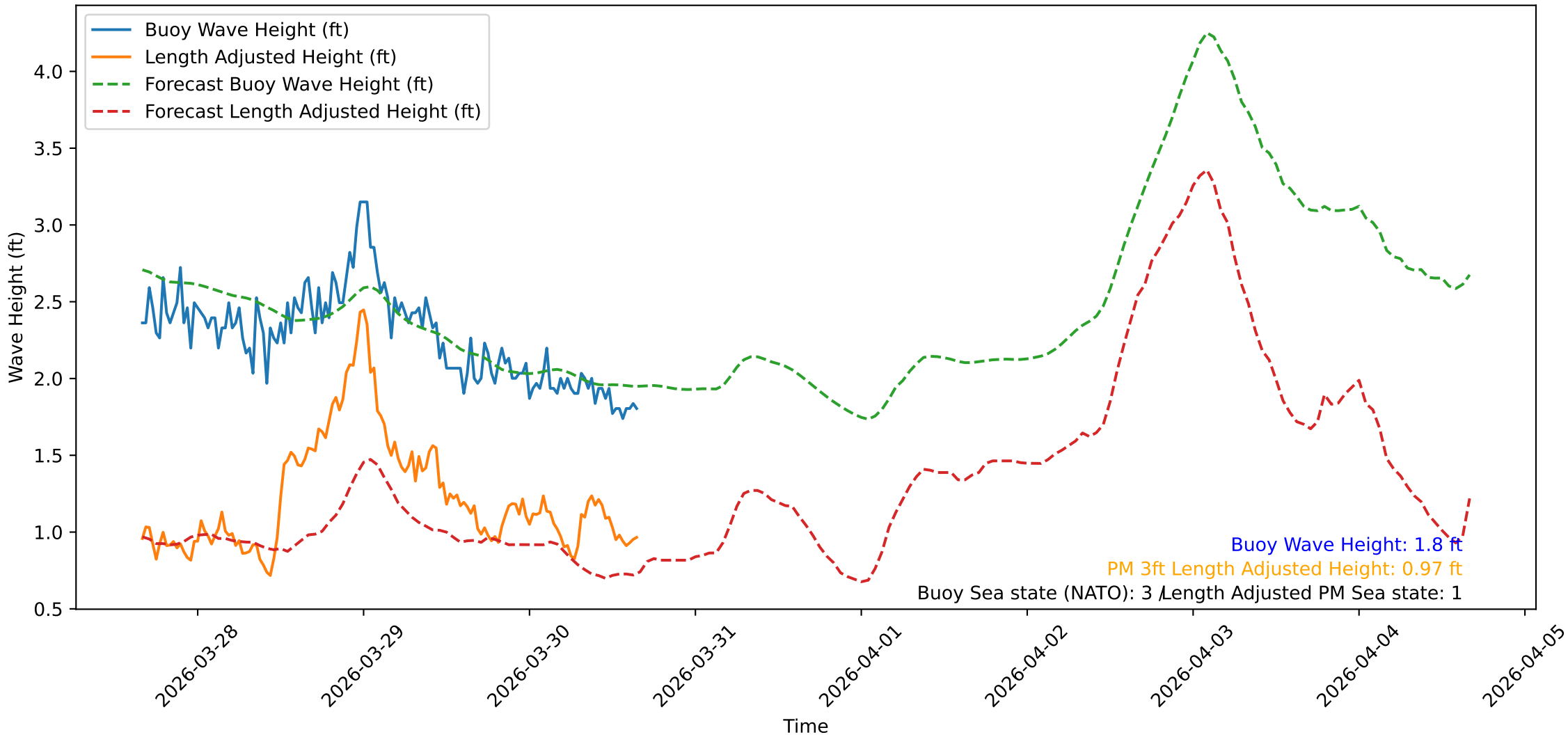
Wave Heights over Time for Oceanside Harbor at 2026-03-30 16:10:32
