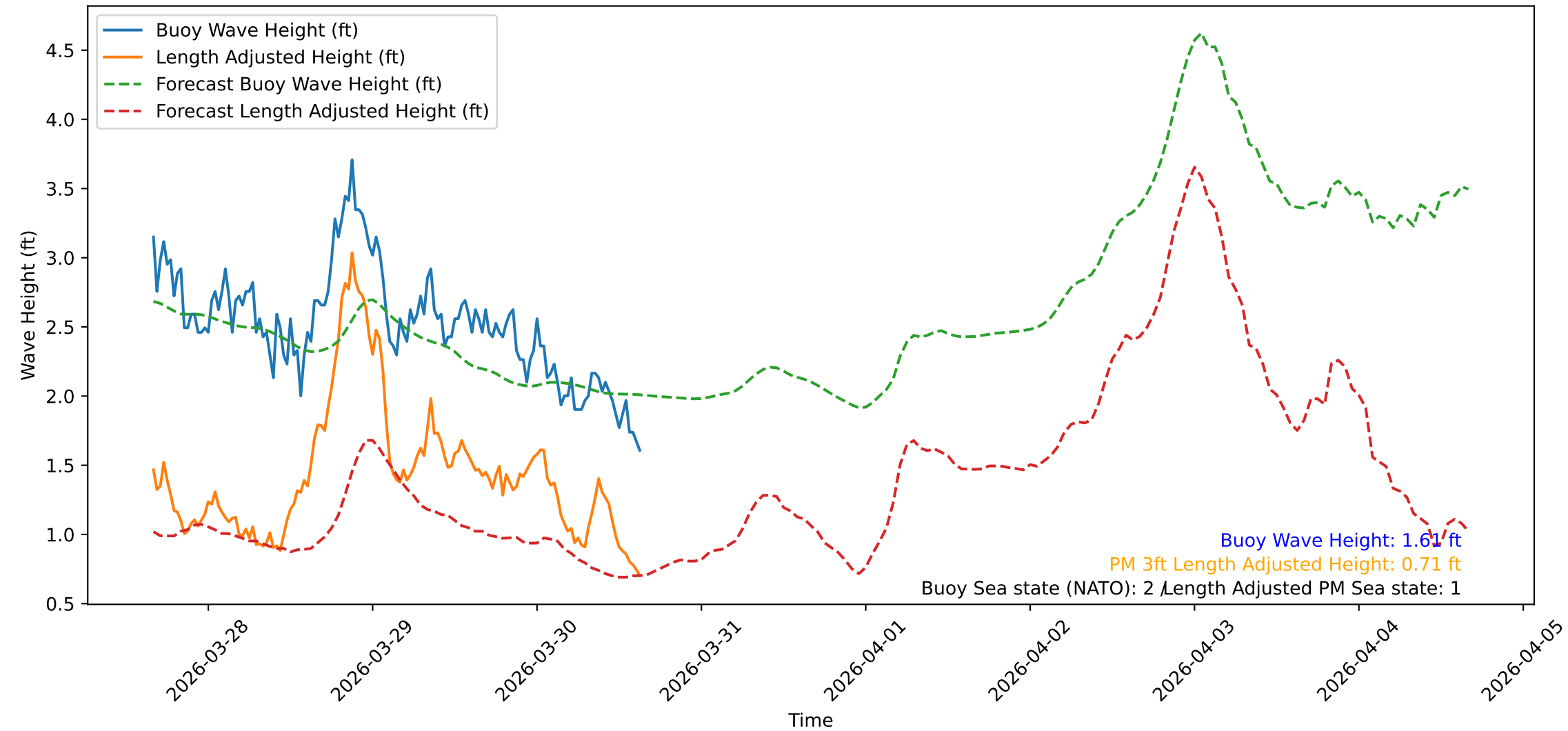
Wave Heights over Time for Green Beach at 2026-03-30 16:11:10
