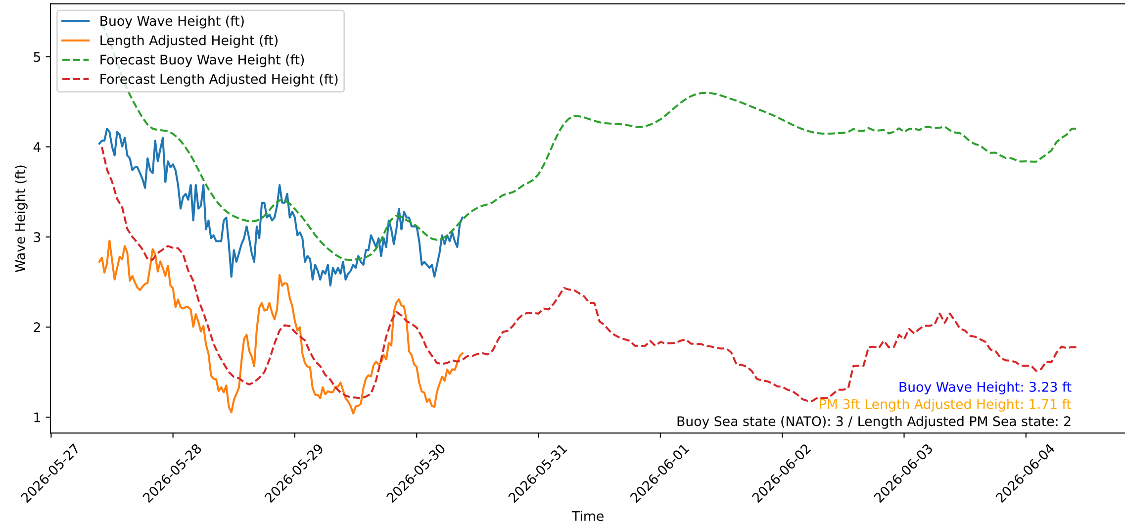
Wave Heights over Time for Green Beach at 2026-05-30 09:41:06
