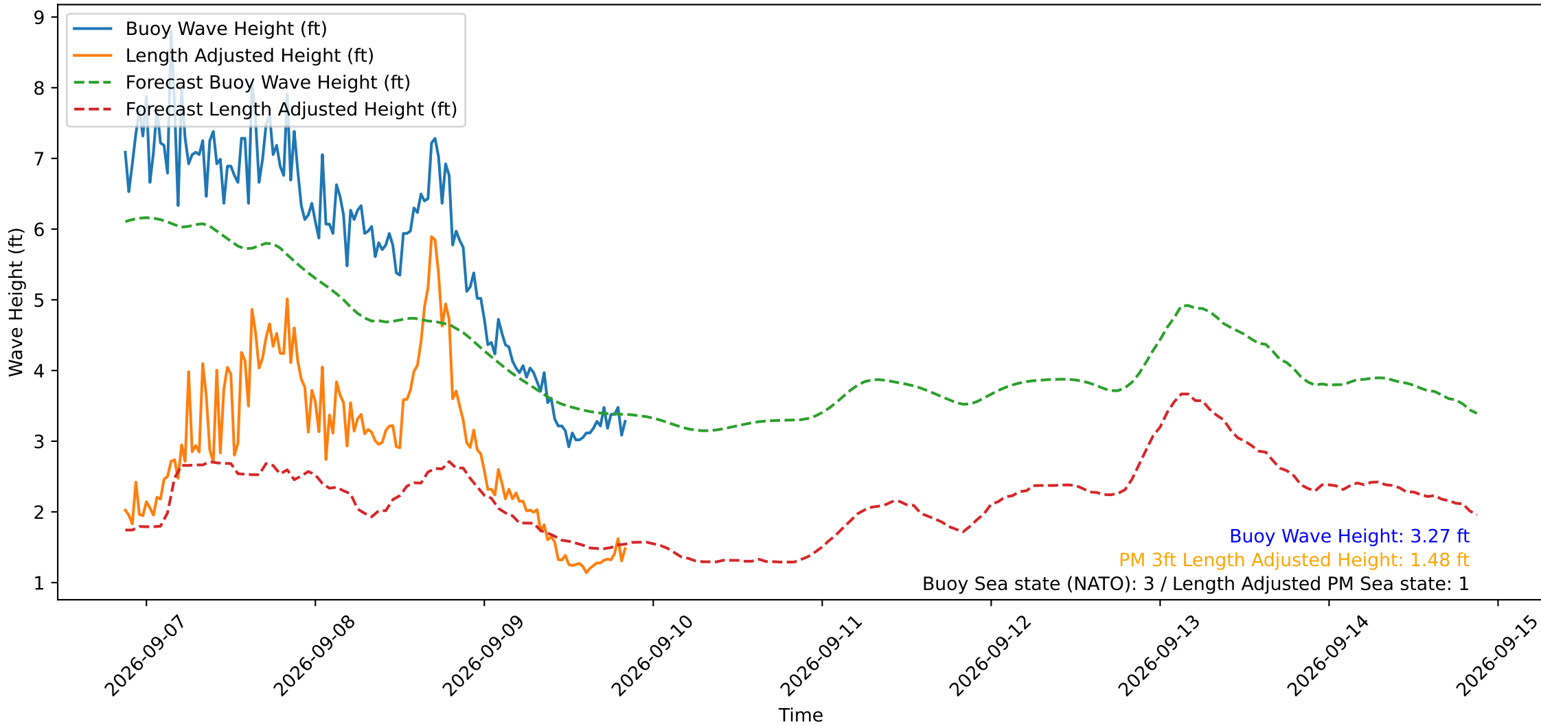
Wave Heights over Time for Green Beach at 2026-09-09 20:51:12
