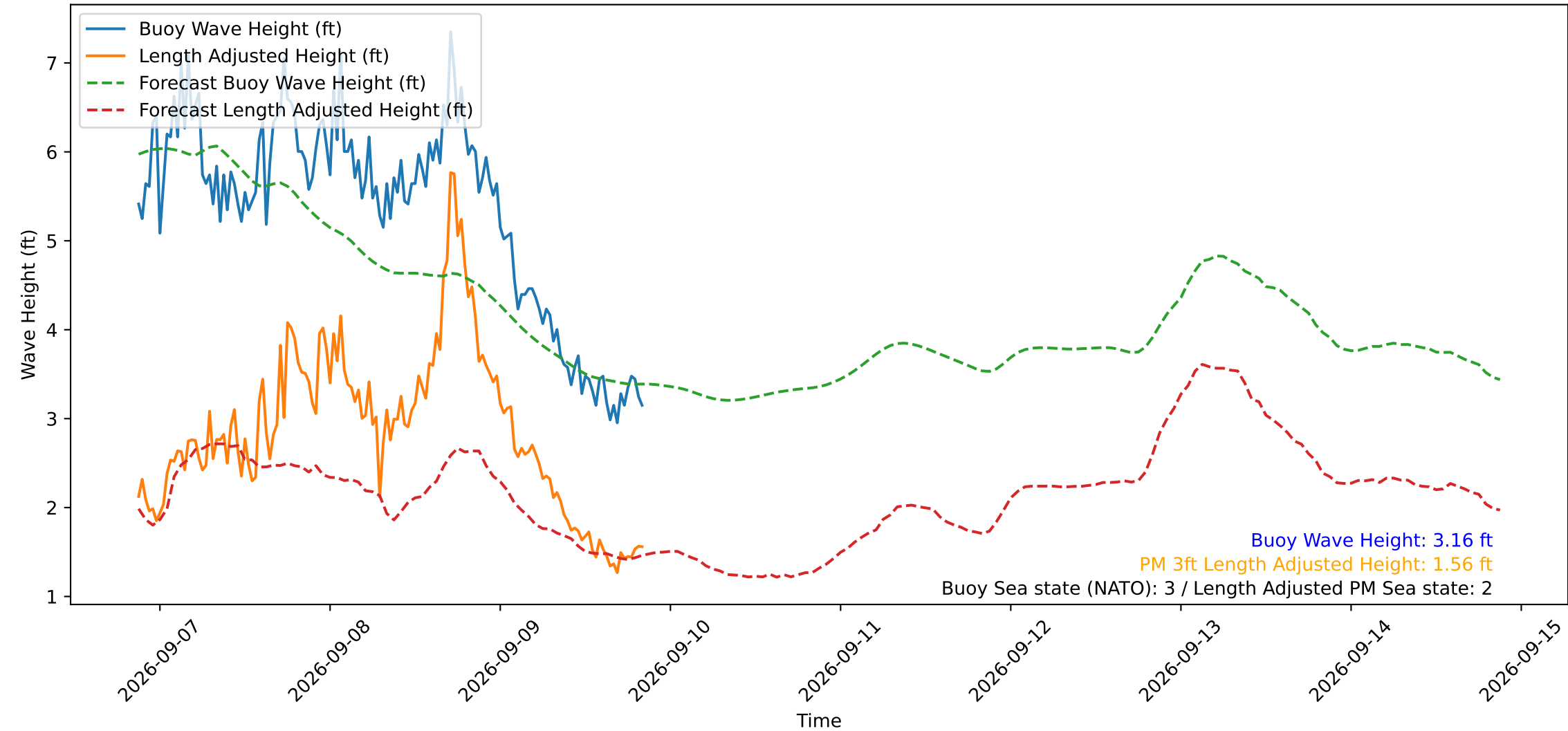
Wave Heights over Time for Oceanside Harbor at 2026-09-09 20:50:29
