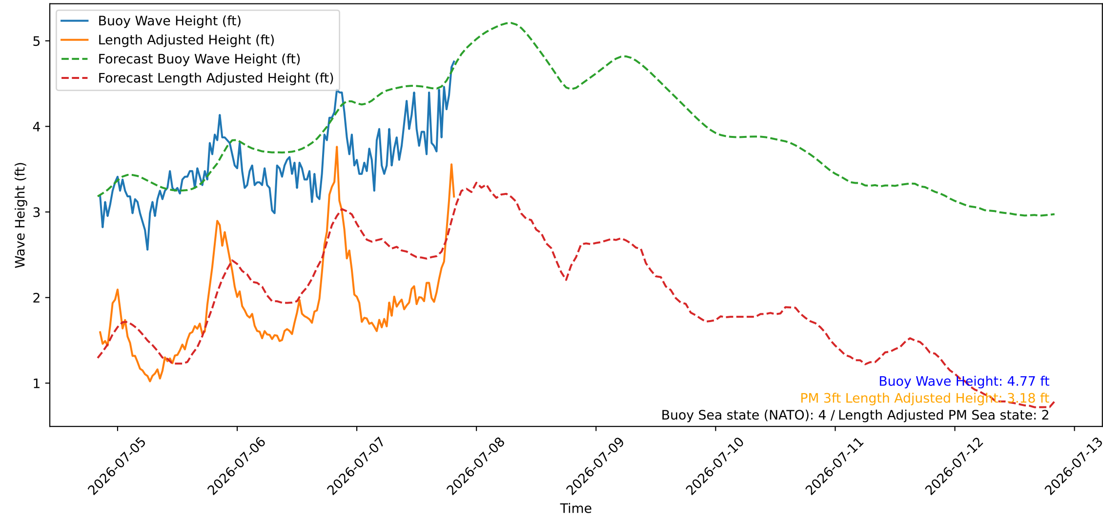
Wave Heights over Time for Green Beach at 2026-07-07 20:21:10
