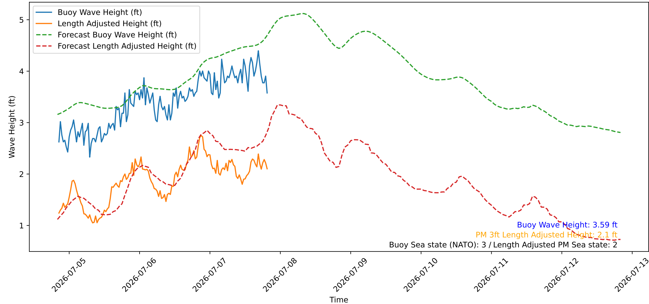
Wave Heights over Time for Oceanside Harbor at 2026-07-07 20:20:26
