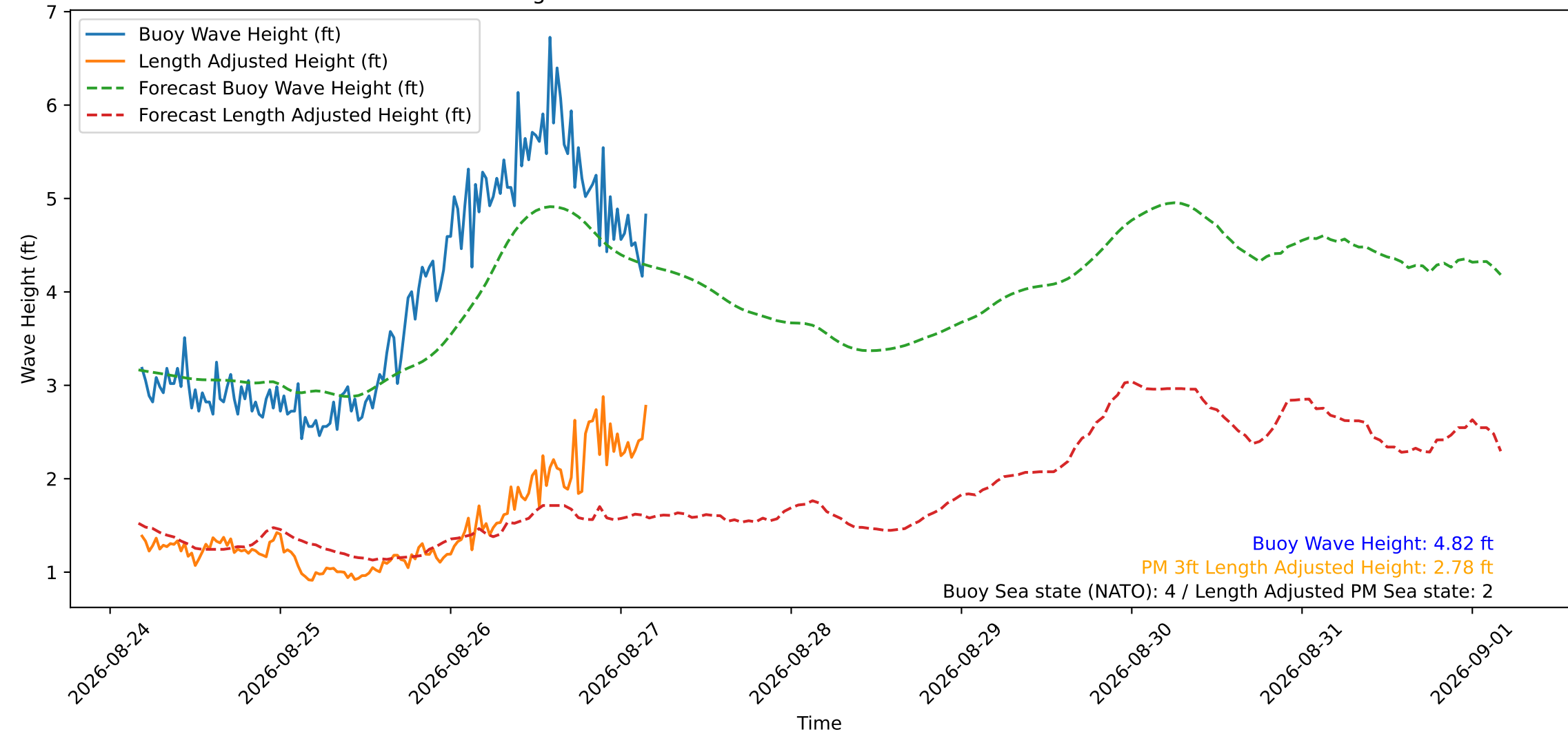
Wave Heights over Time for Oceanside Harbor at 2026-08-27 04:20:29
