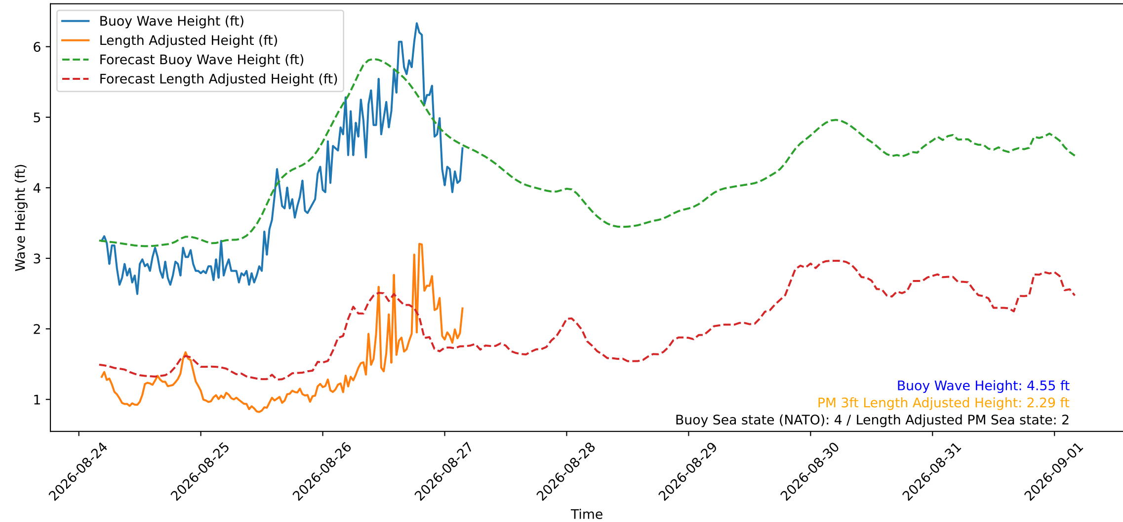
Wave Heights over Time for Green Beach at 2026-08-27 04:21:14
