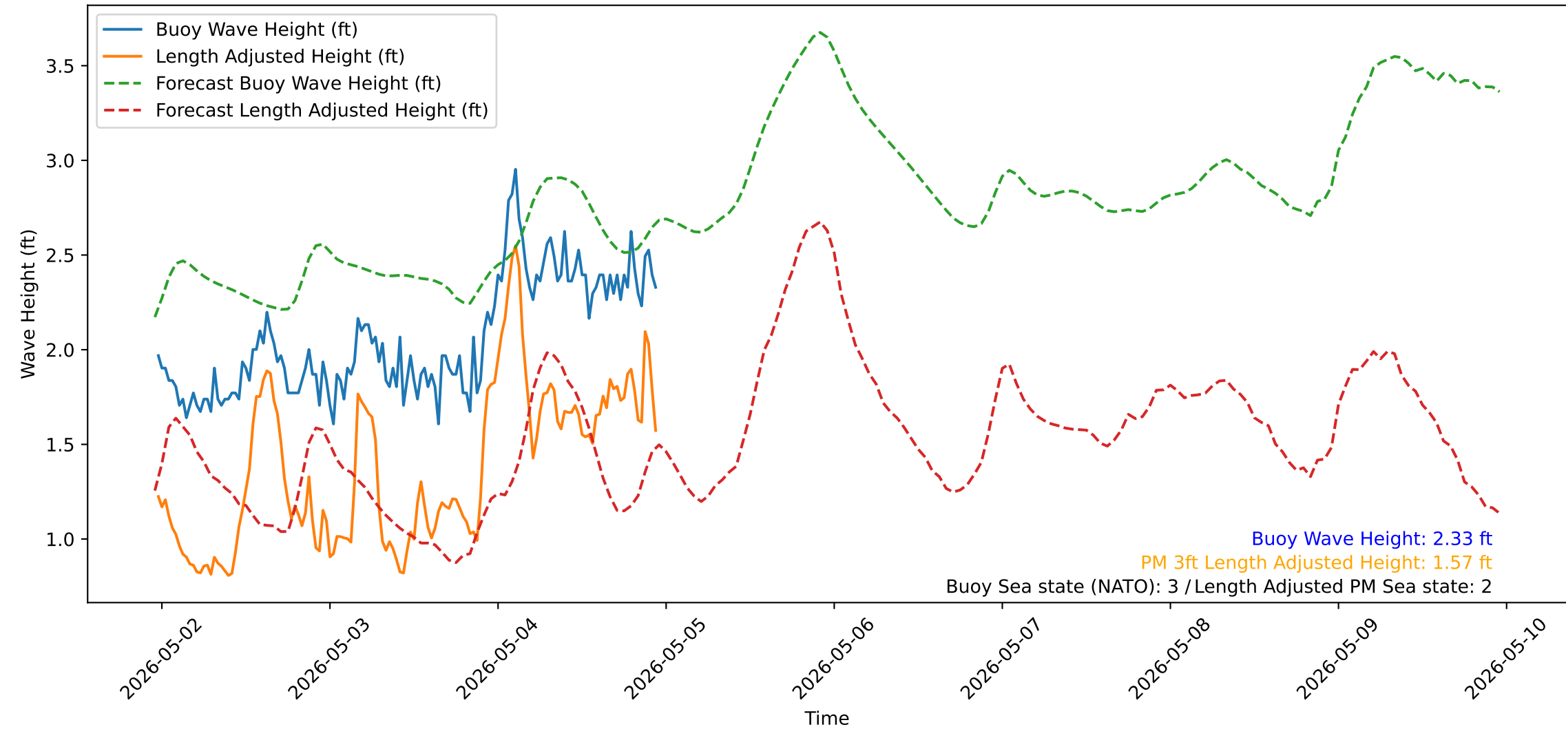
Wave Heights over Time for Red Beach at 2026-05-04 23:20:52
