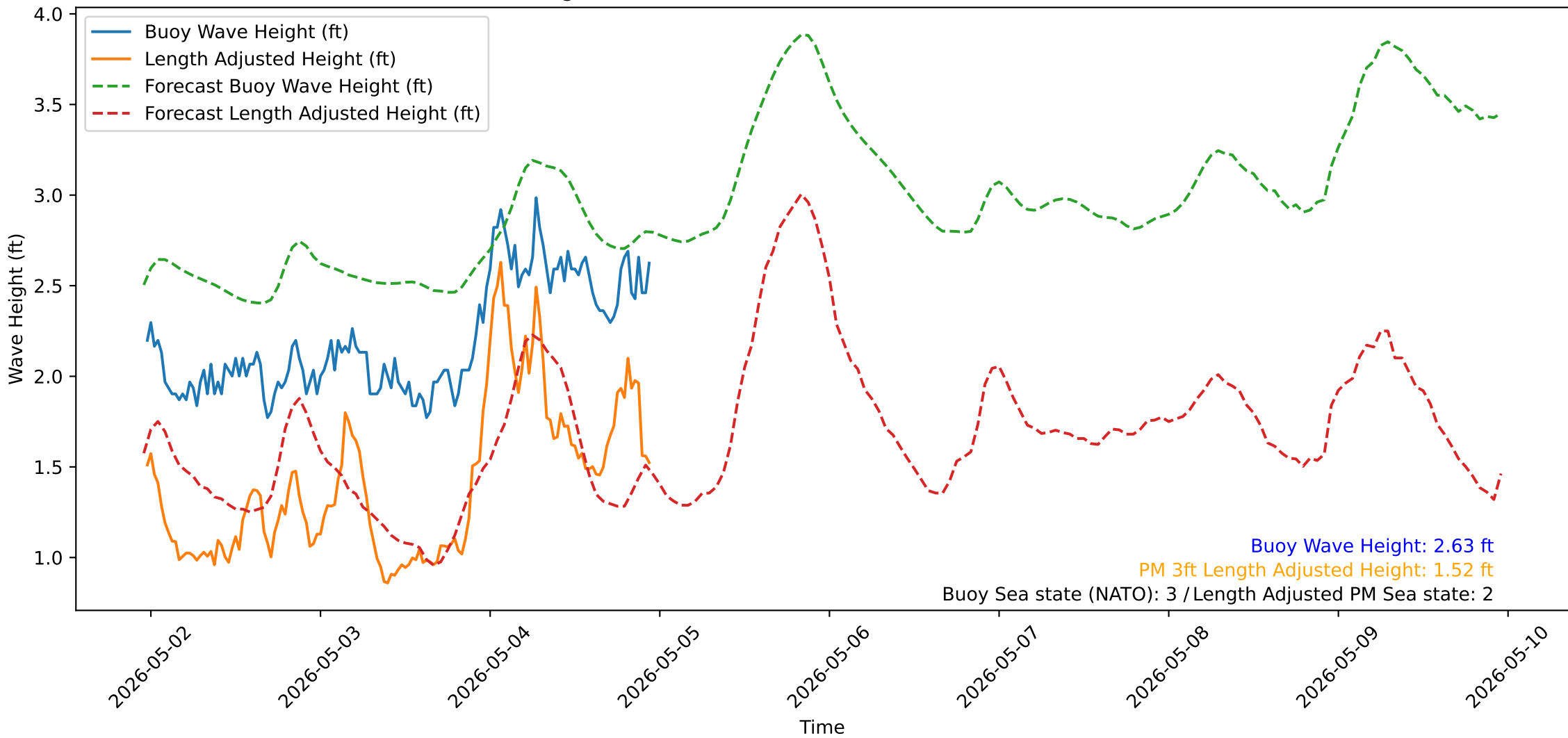
Wave Heights over Time for Green Beach at 2026-05-04 23:21:15
