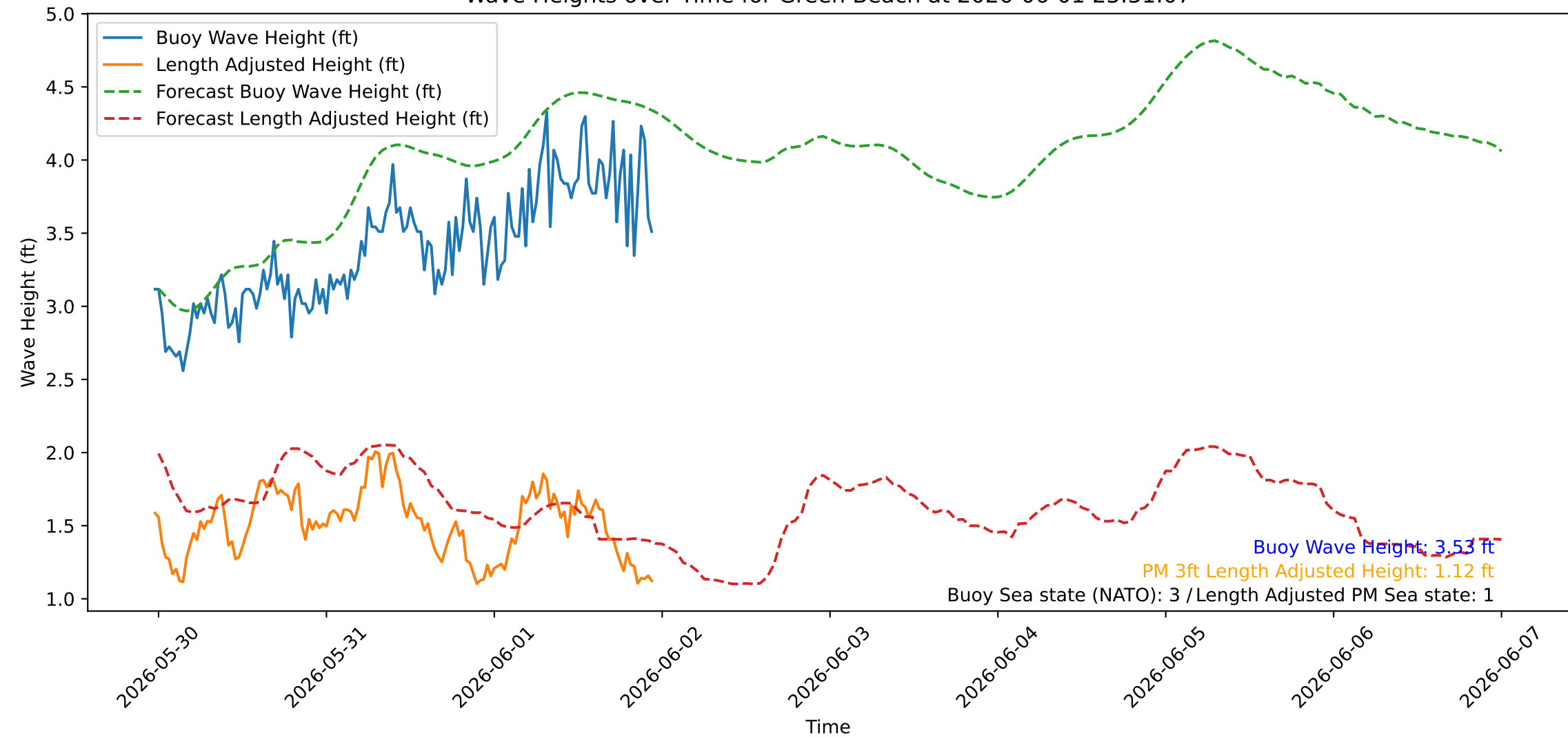
Wave Heights over Time for Green Beach at 2026-06-01 23:31:07
