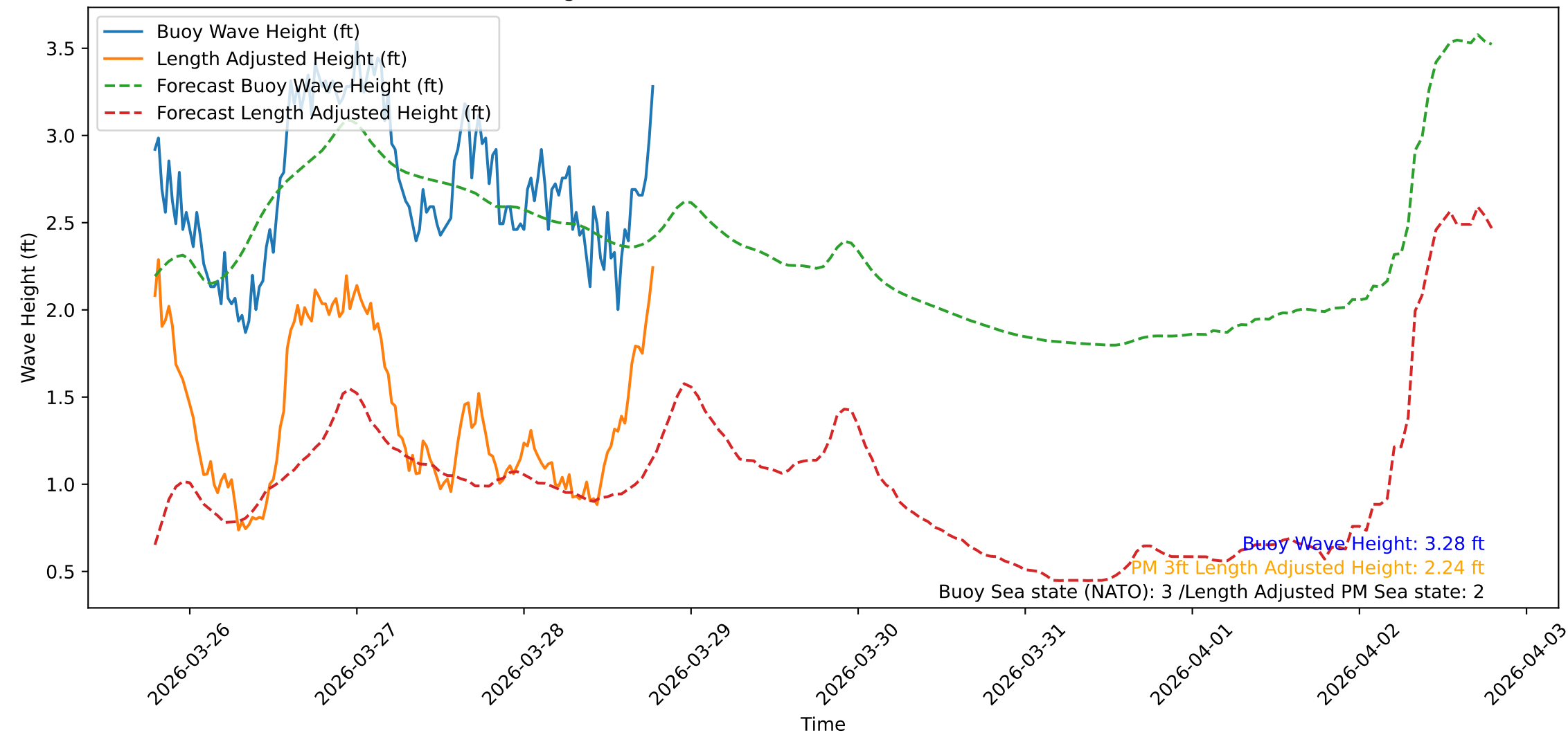
Wave Heights over Time for Green Beach at 2026-03-28 19:11:08
