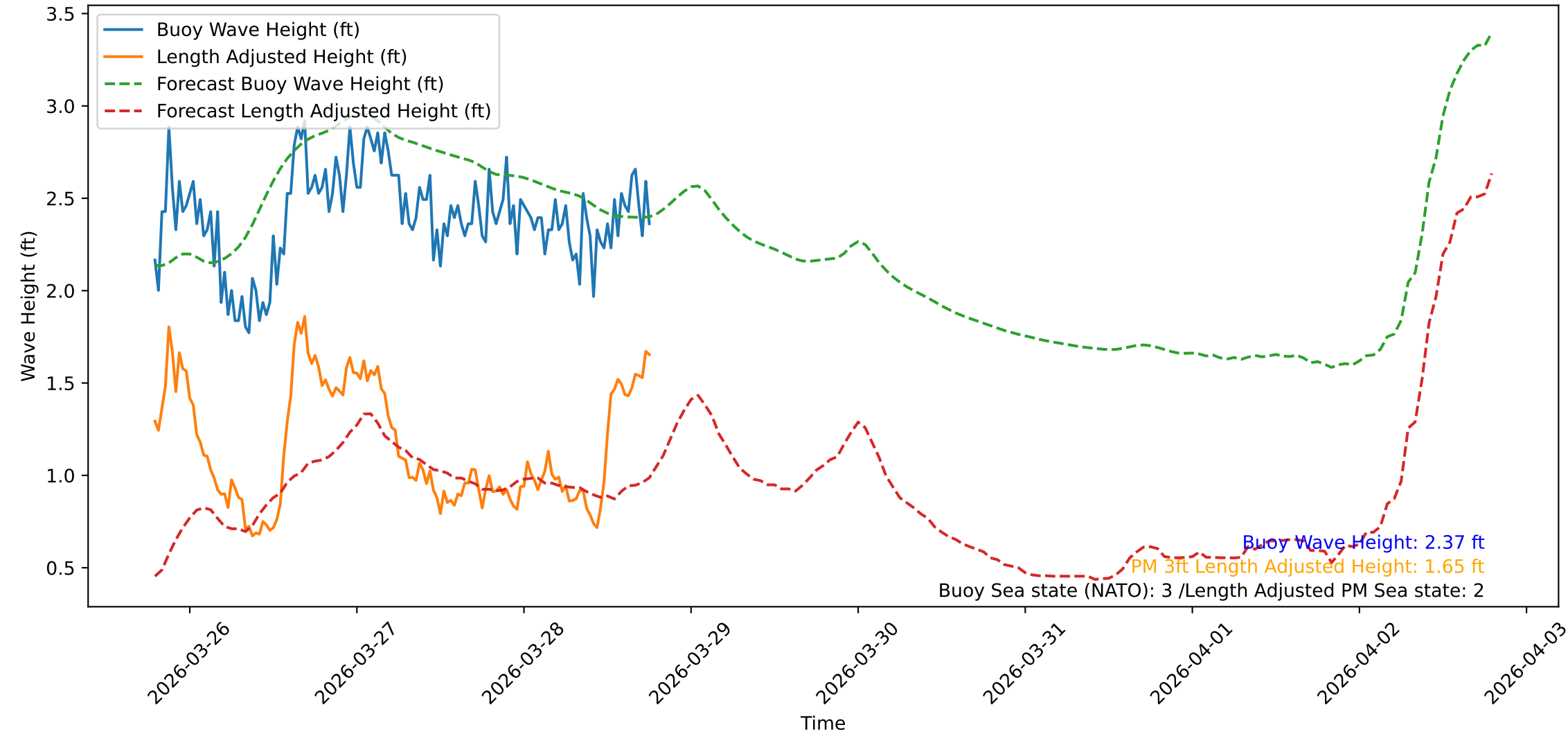
Wave Heights over Time for Oceanside Harbor at 2026-03-28 19:10:31
