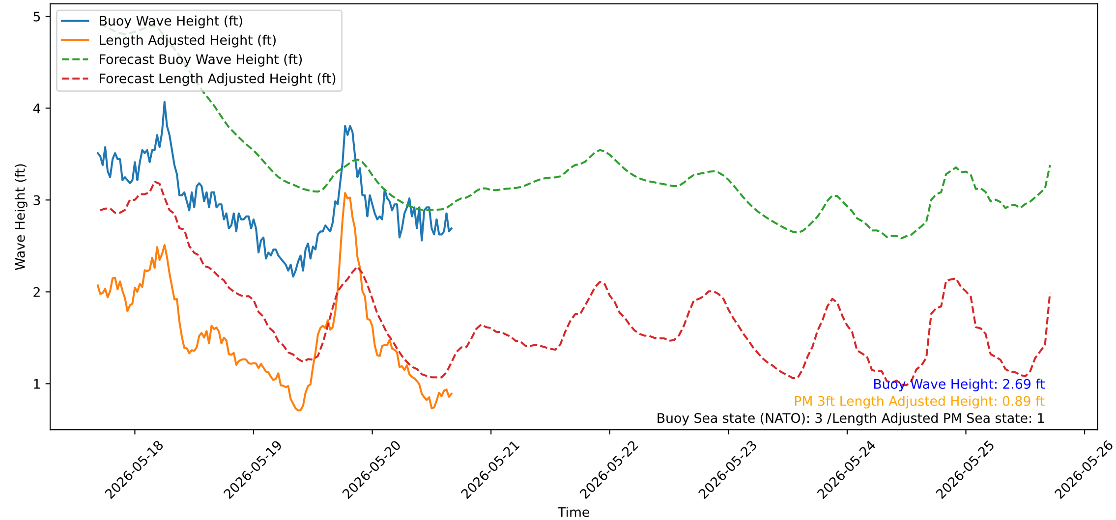
Wave Heights over Time for Green Beach at 2026-05-20 16:41:14
