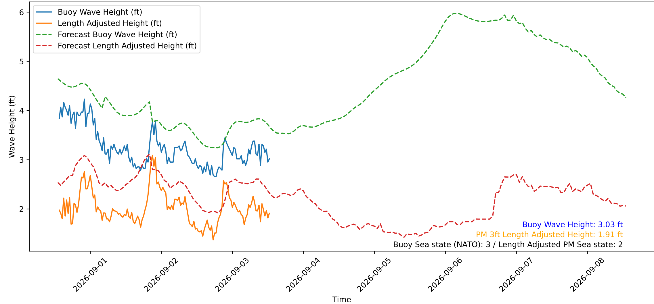
Wave Heights over Time for Green Beach at 2026-09-03 13:21:15
