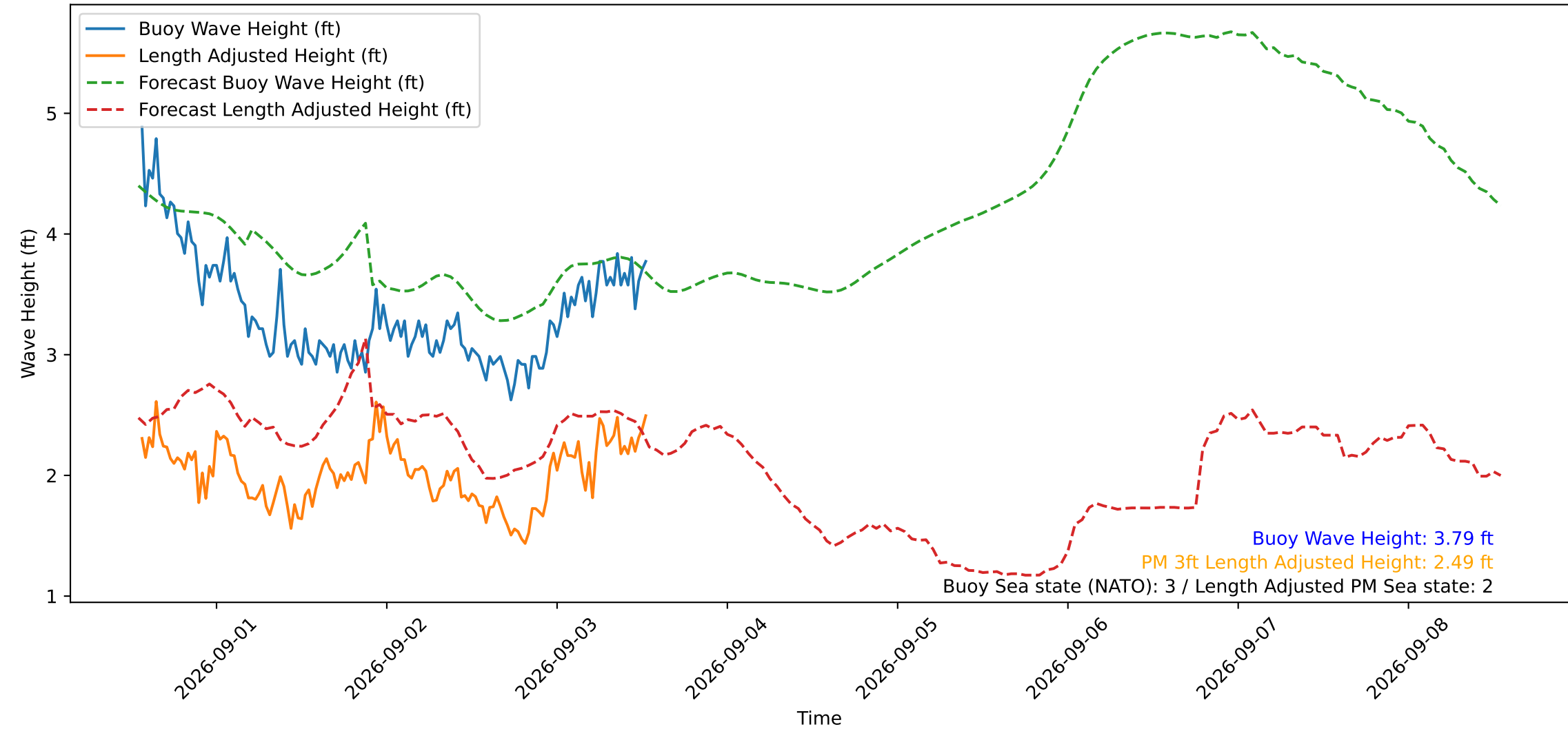
Wave Heights over Time for Oceanside Harbor at 2026-09-03 13:20:30
