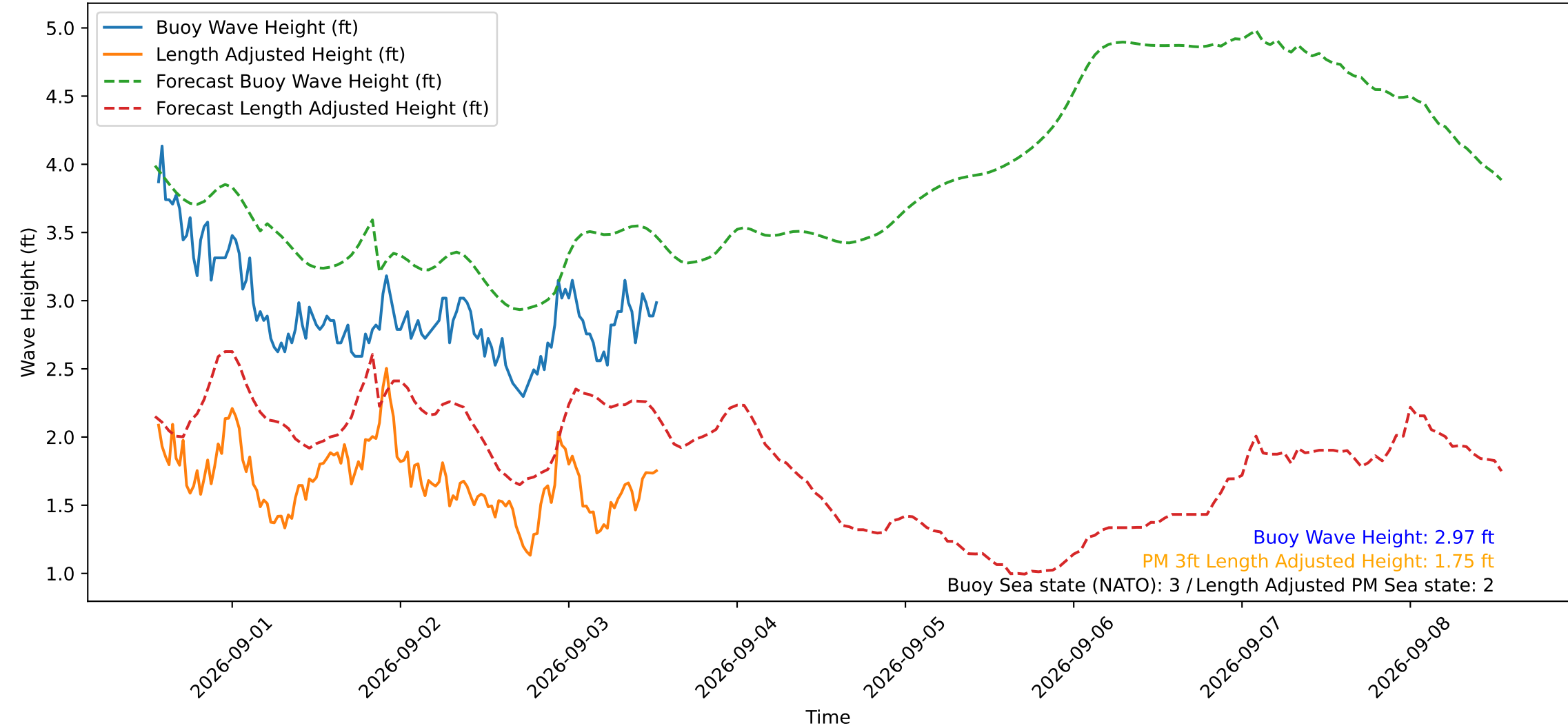
Wave Heights over Time for Red Beach at 2026-09-03 13:20:51
