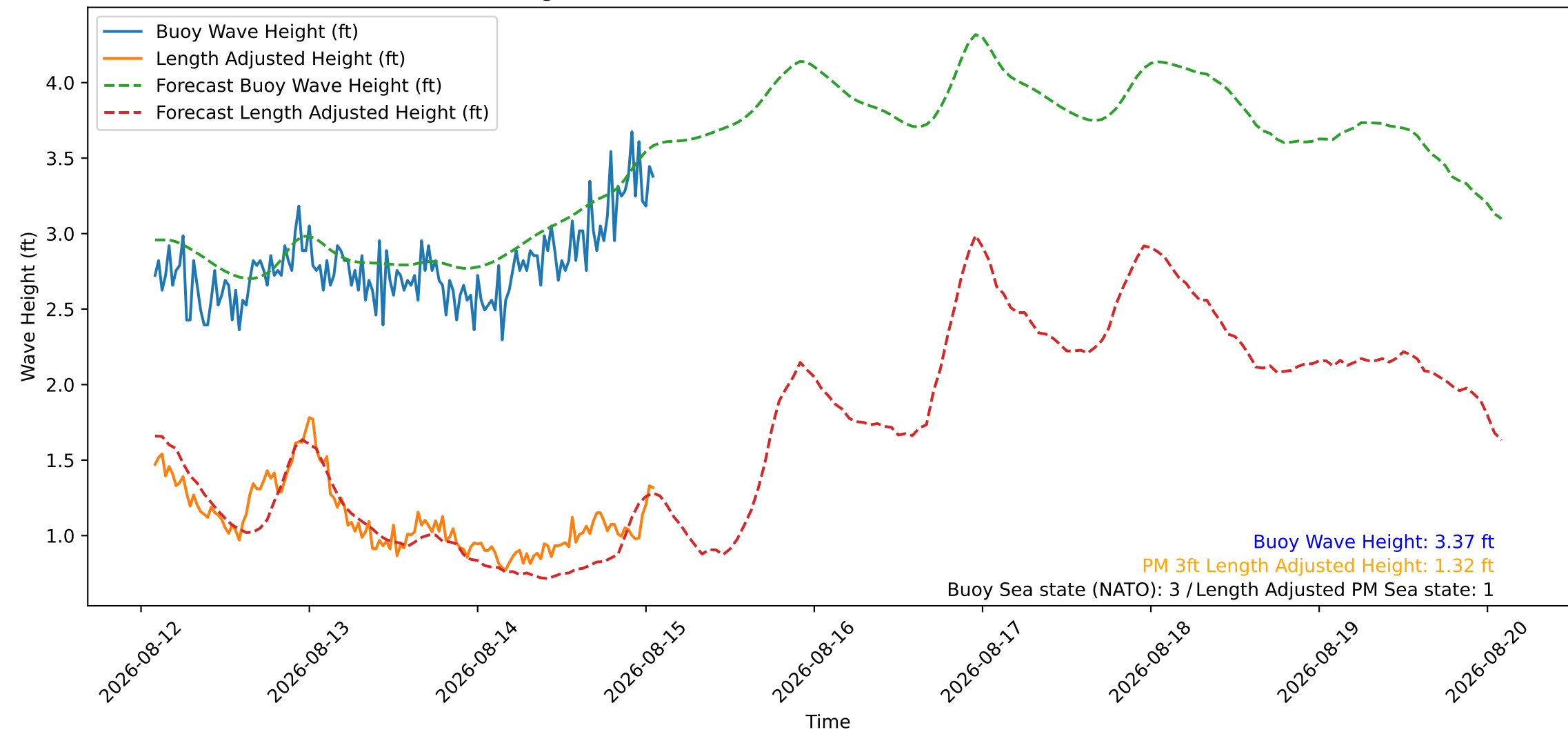
Wave Heights over Time for Oceanside Harbor at 2026-08-15 02:00:26
