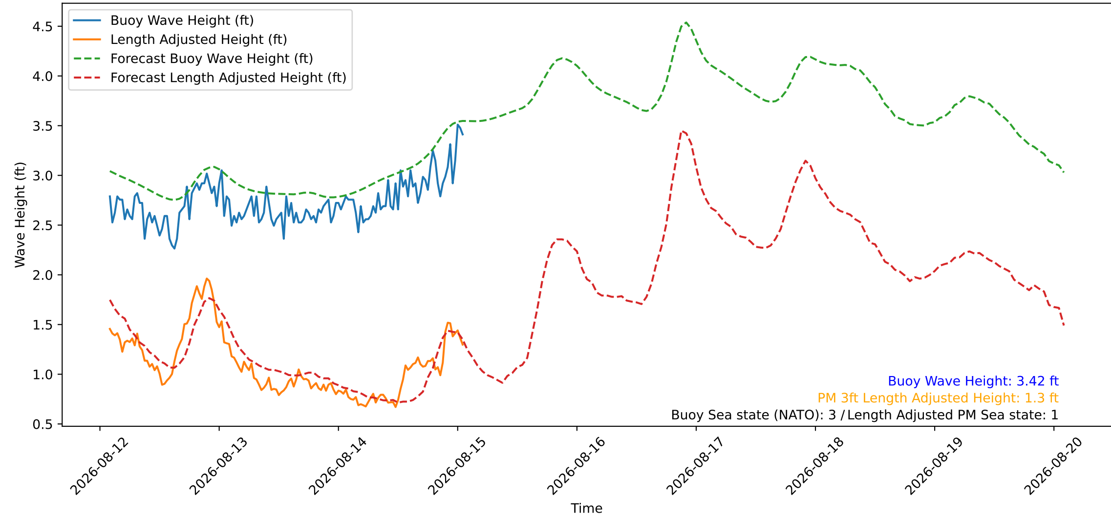
Wave Heights over Time for Green Beach at 2026-08-15 02:01:09
