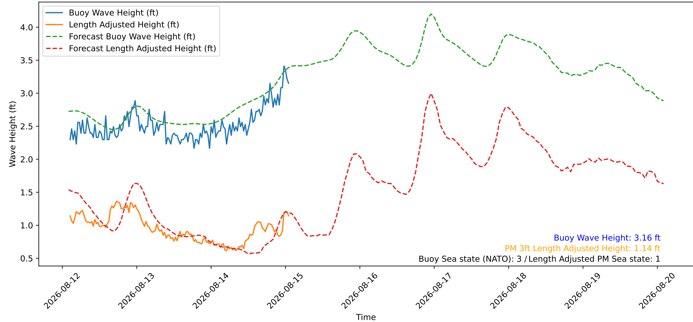
Wave Heights over Time for Red Beach at 2026-08-15 02:00:46
