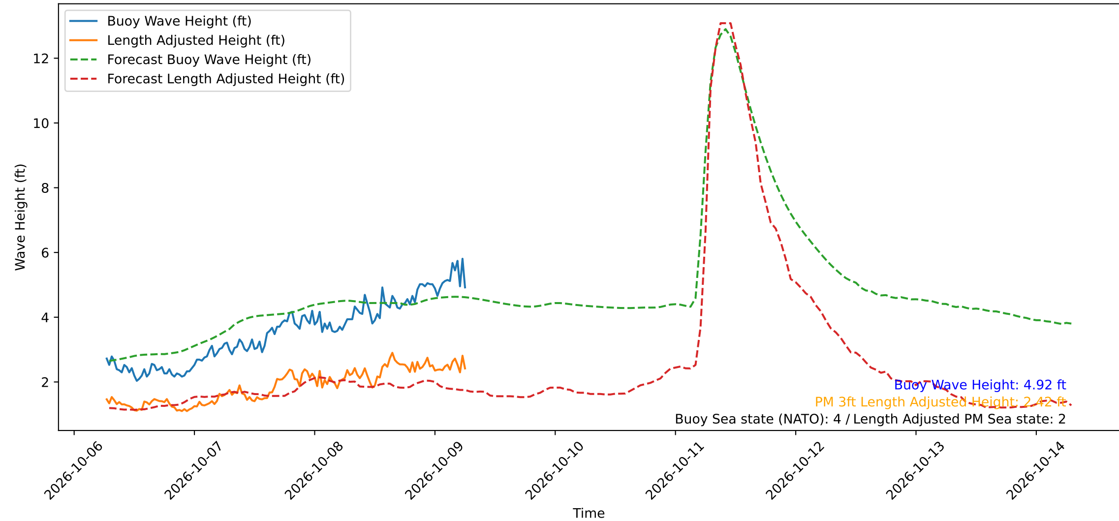
Wave Heights over Time for Oceanside Harbor at 2026-10-09 06:40:29
