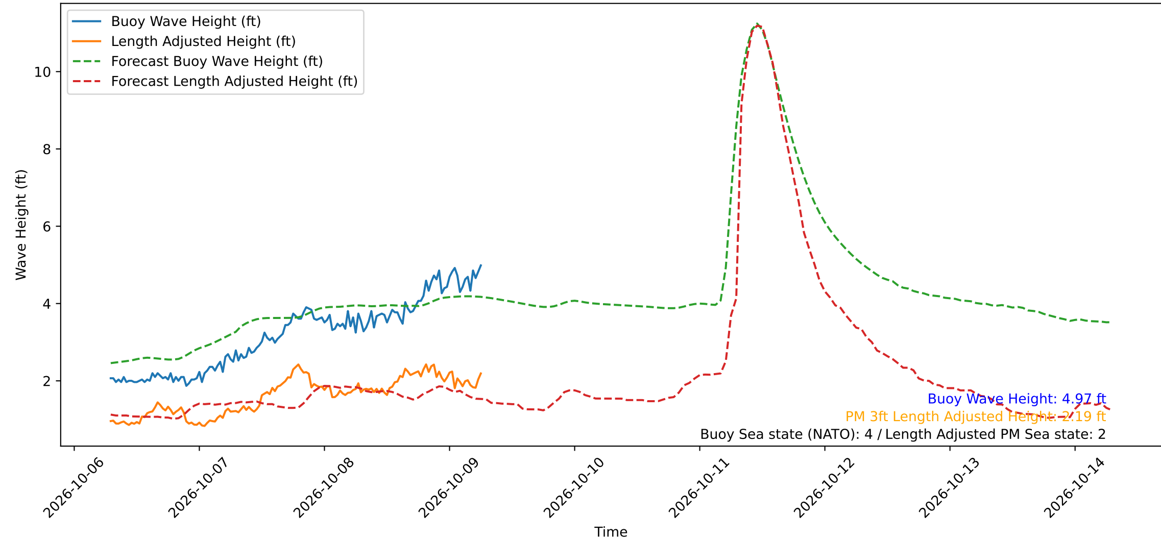
Wave Heights over Time for Red Beach at 2026-10-09 06:40:49
