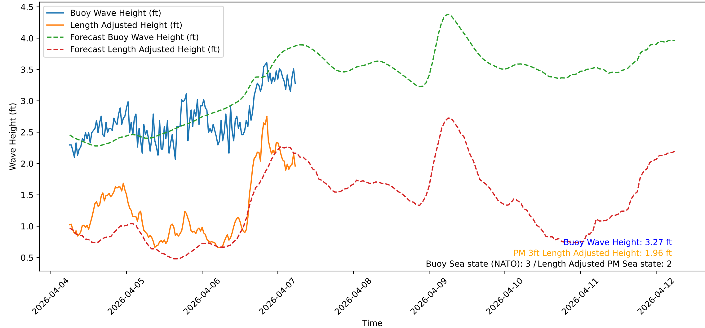
Wave Heights over Time for Oceanside Harbor at 2026-04-07 06:10:31
