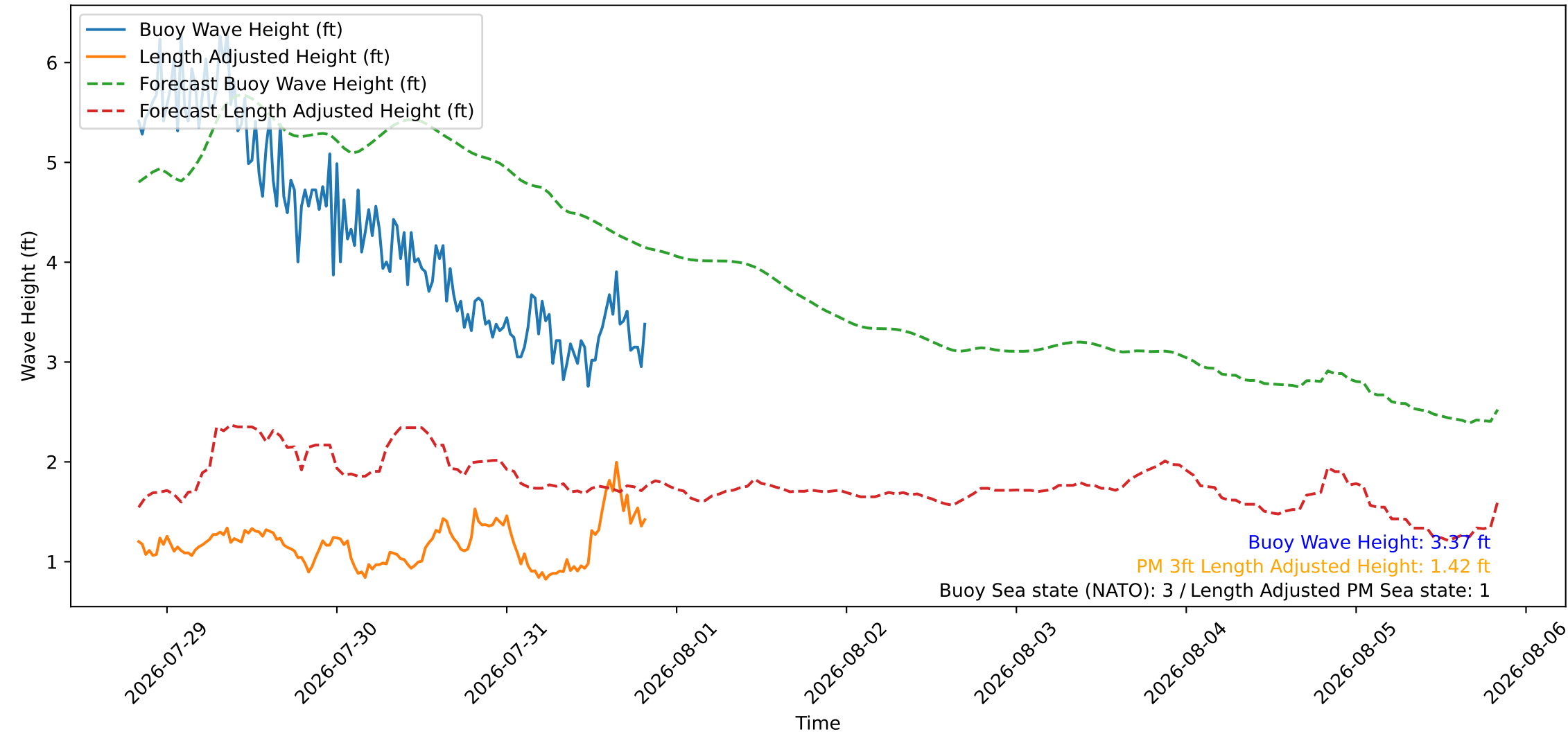
Wave Heights over Time for Green Beach at 2026-07-31 20:11:09
