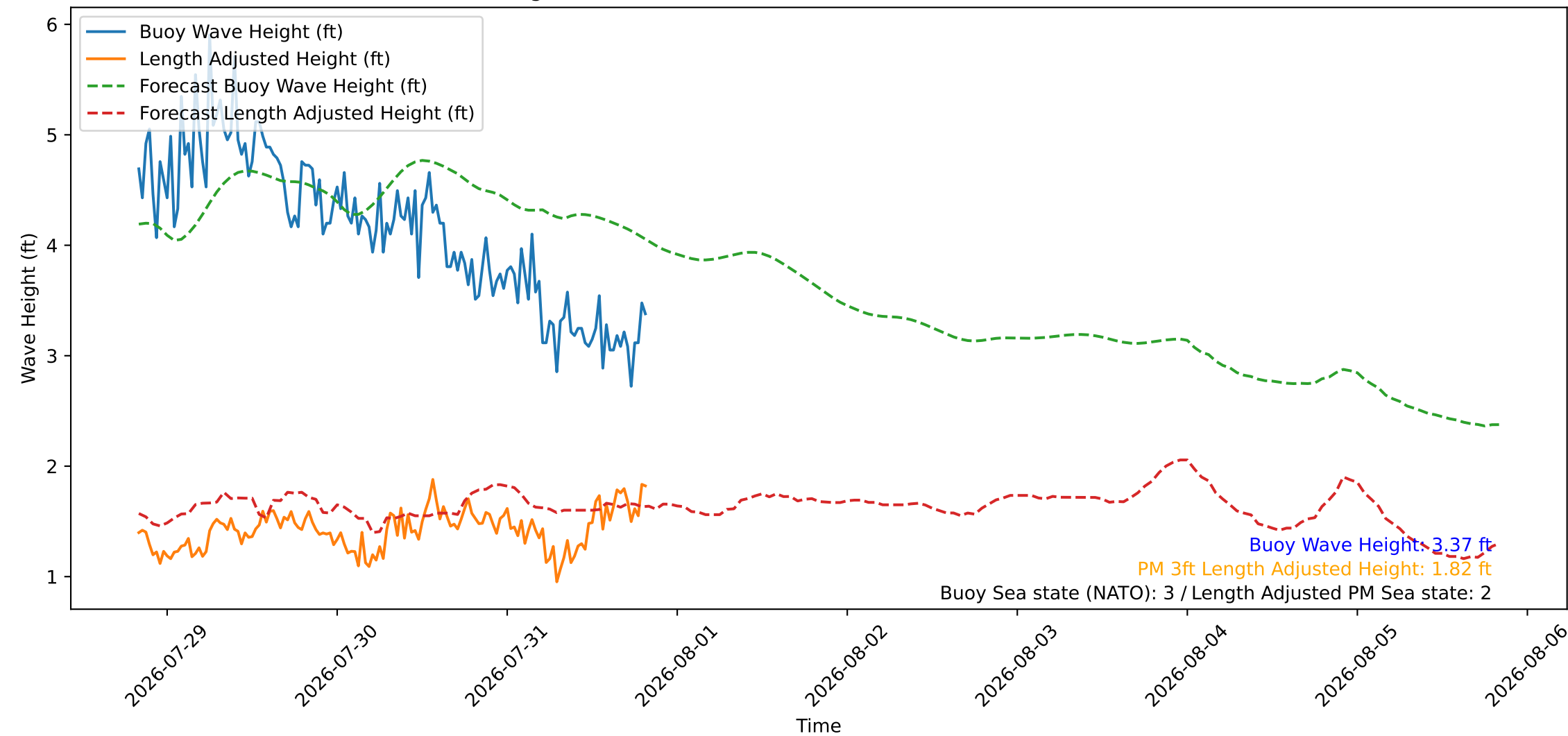
Wave Heights over Time for Oceanside Harbor at 2026-07-31 20:10:27
