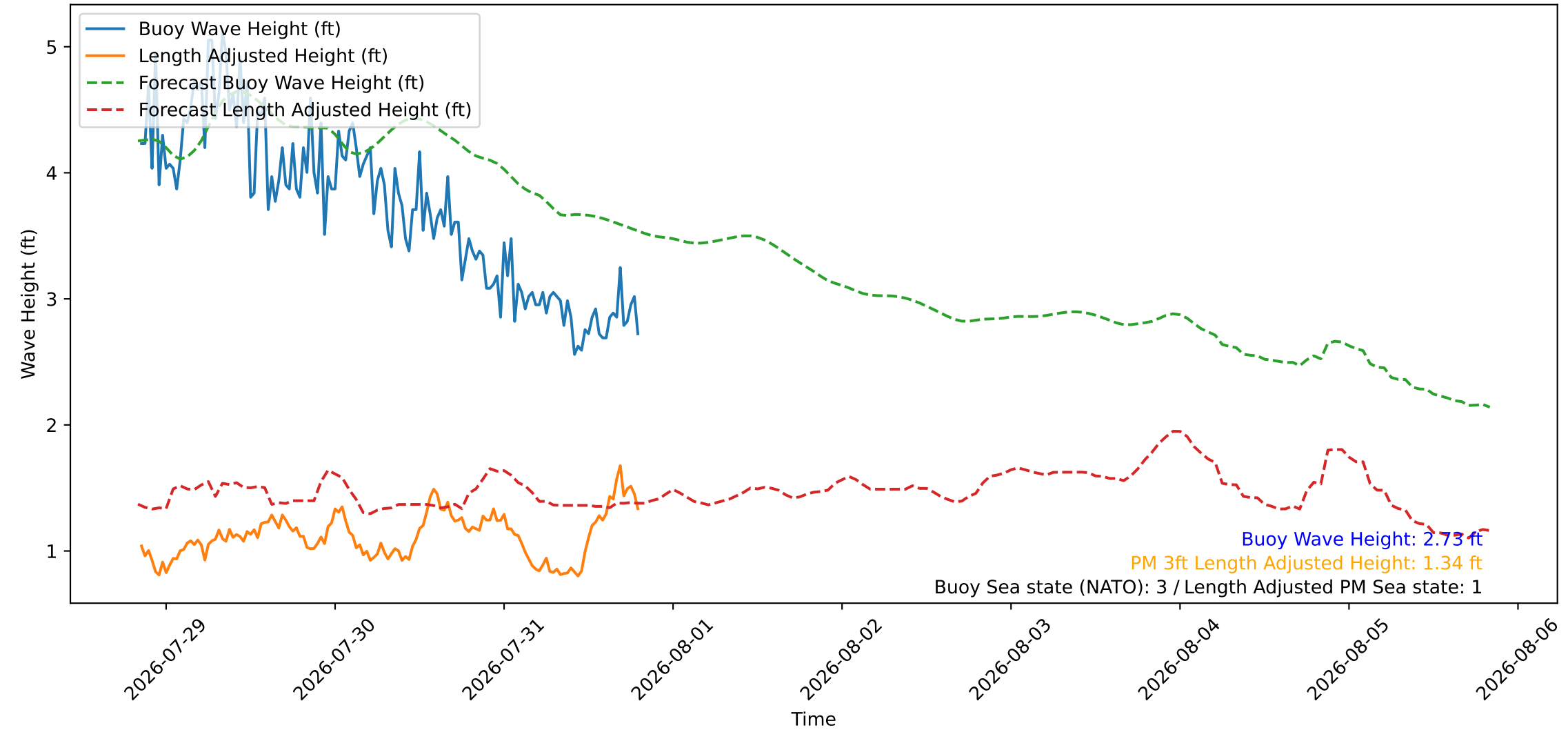
Wave Heights over Time for Red Beach at 2026-07-31 20:10:46
