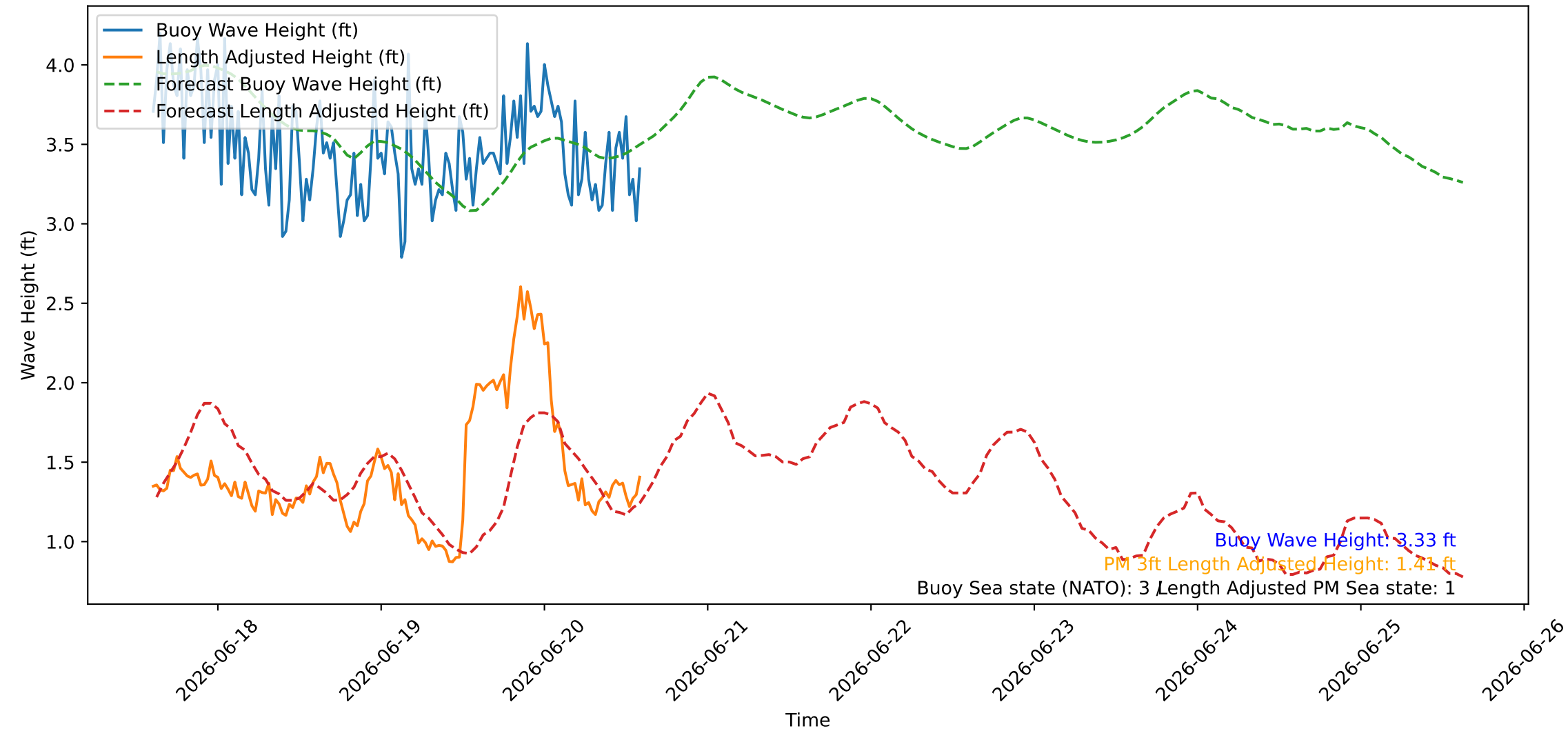
Wave Heights over Time for Oceanside Harbor at 2026-06-20 14:40:26
