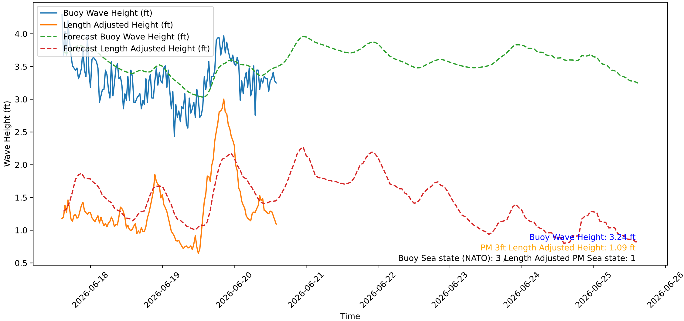
Wave Heights over Time for Green Beach at 2026-06-20 14:41:07
