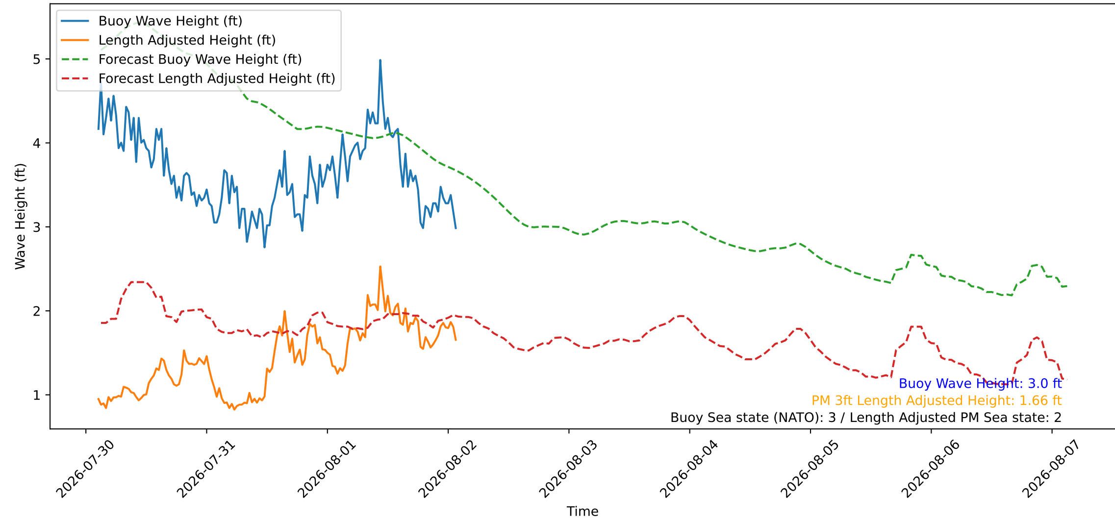
Wave Heights over Time for Green Beach at 2026-08-02 02:31:08
