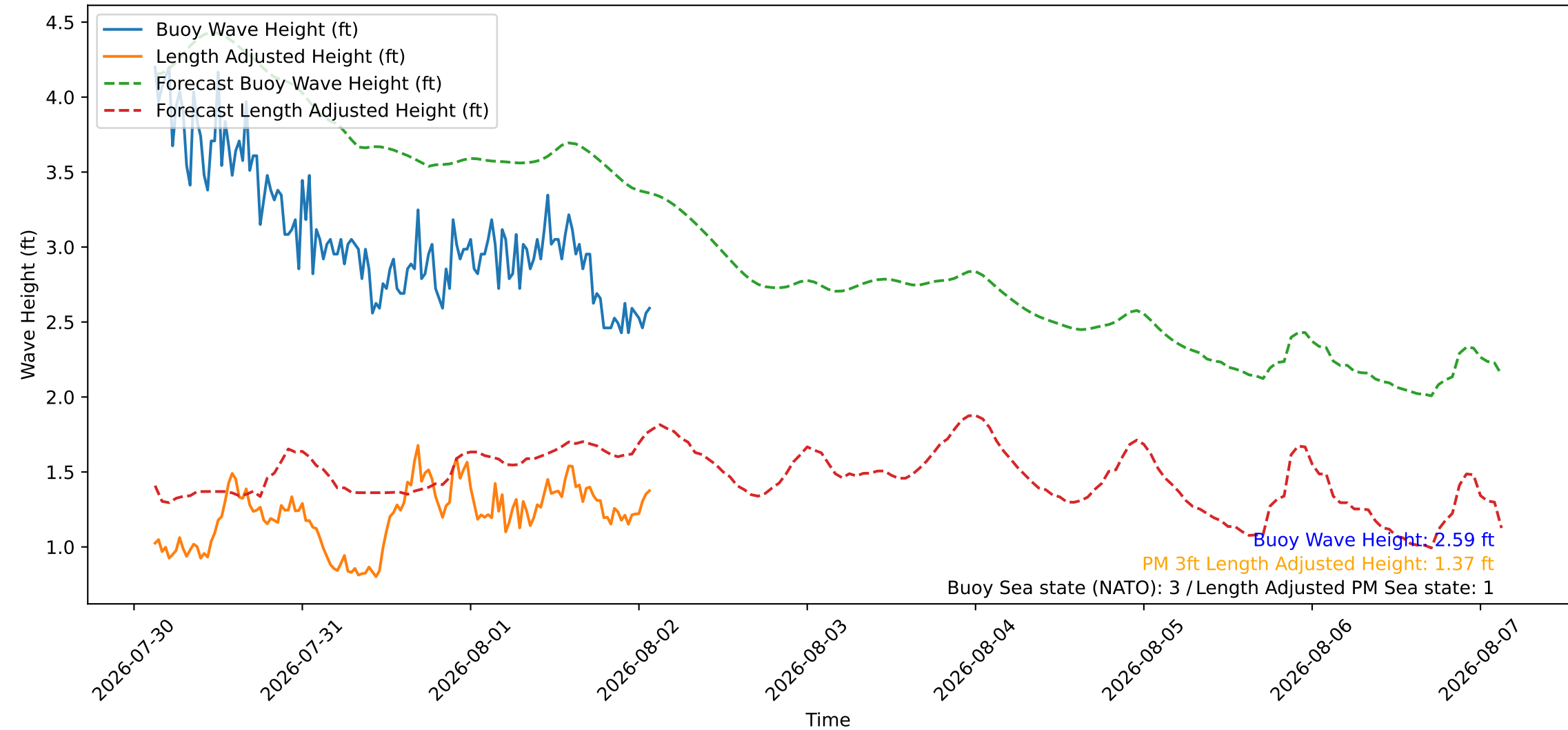
Wave Heights over Time for Red Beach at 2026-08-02 02:30:46
