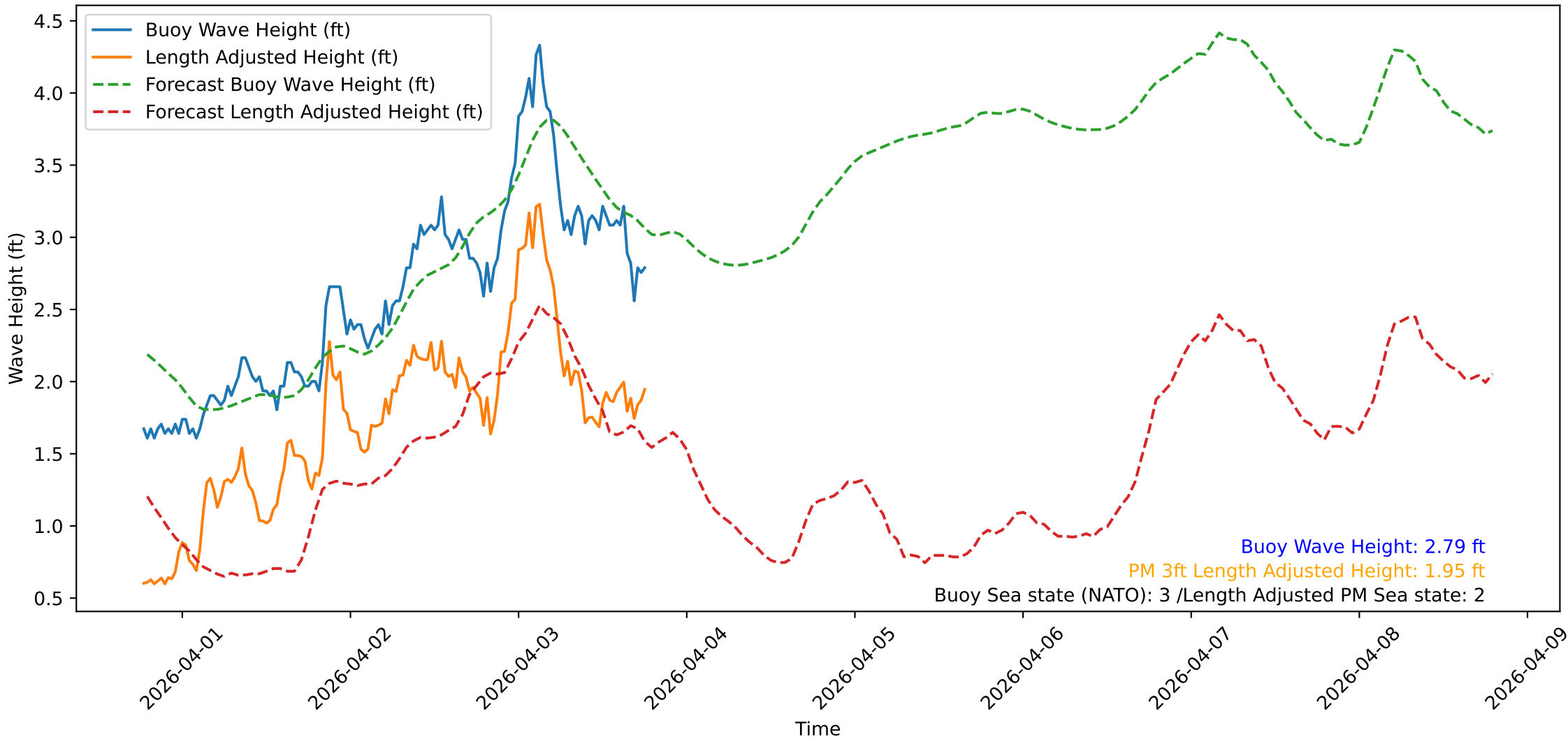
Wave Heights over Time for Green Beach at 2026-04-03 18:41:16
