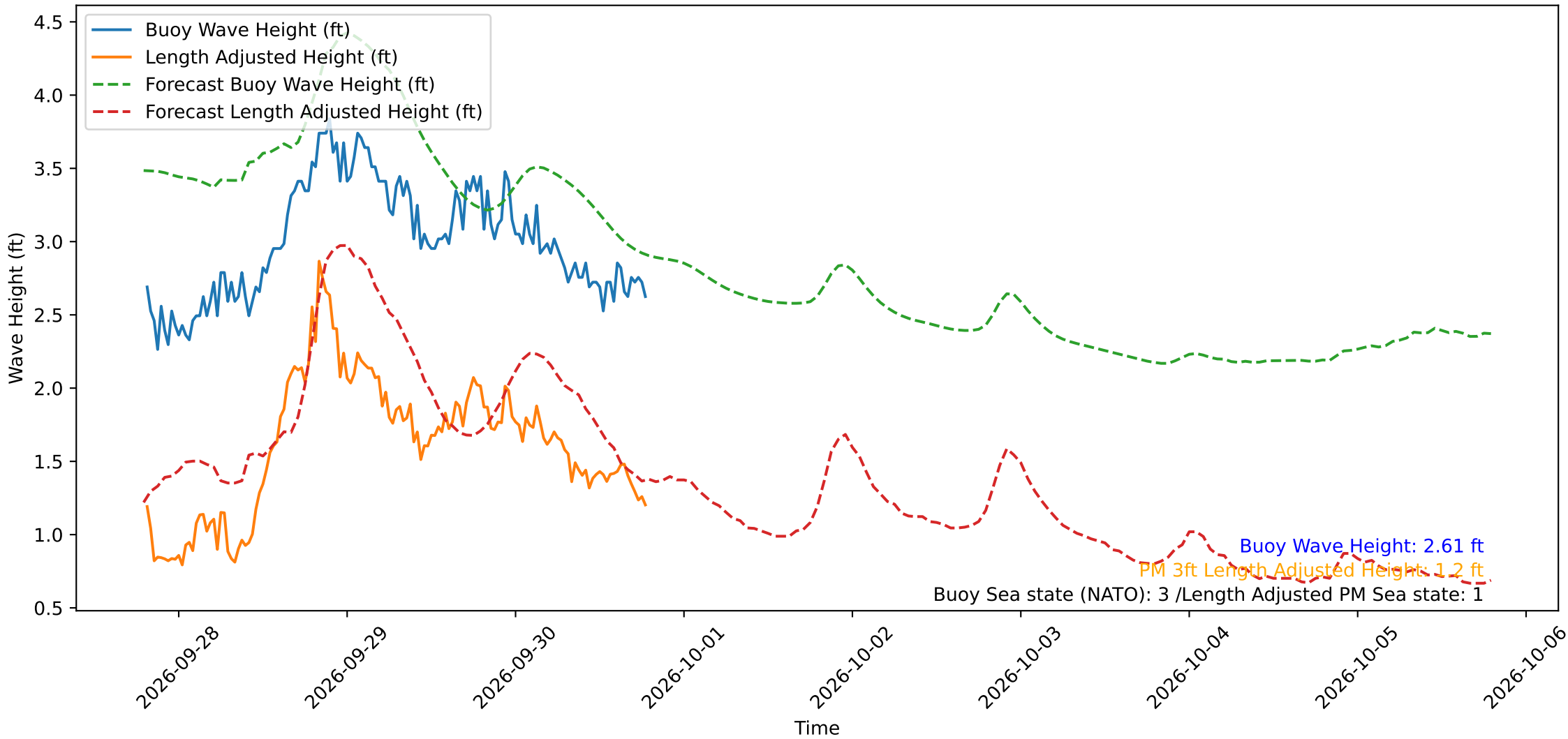
Wave Heights over Time for Red Beach at 2026-09-30 19:10:49
