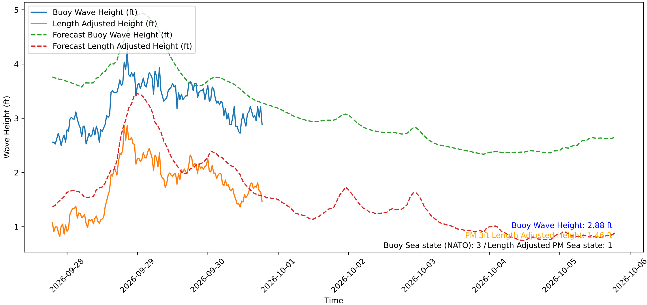
Wave Heights over Time for Oceanside Harbor at 2026-09-30 19:10:30
