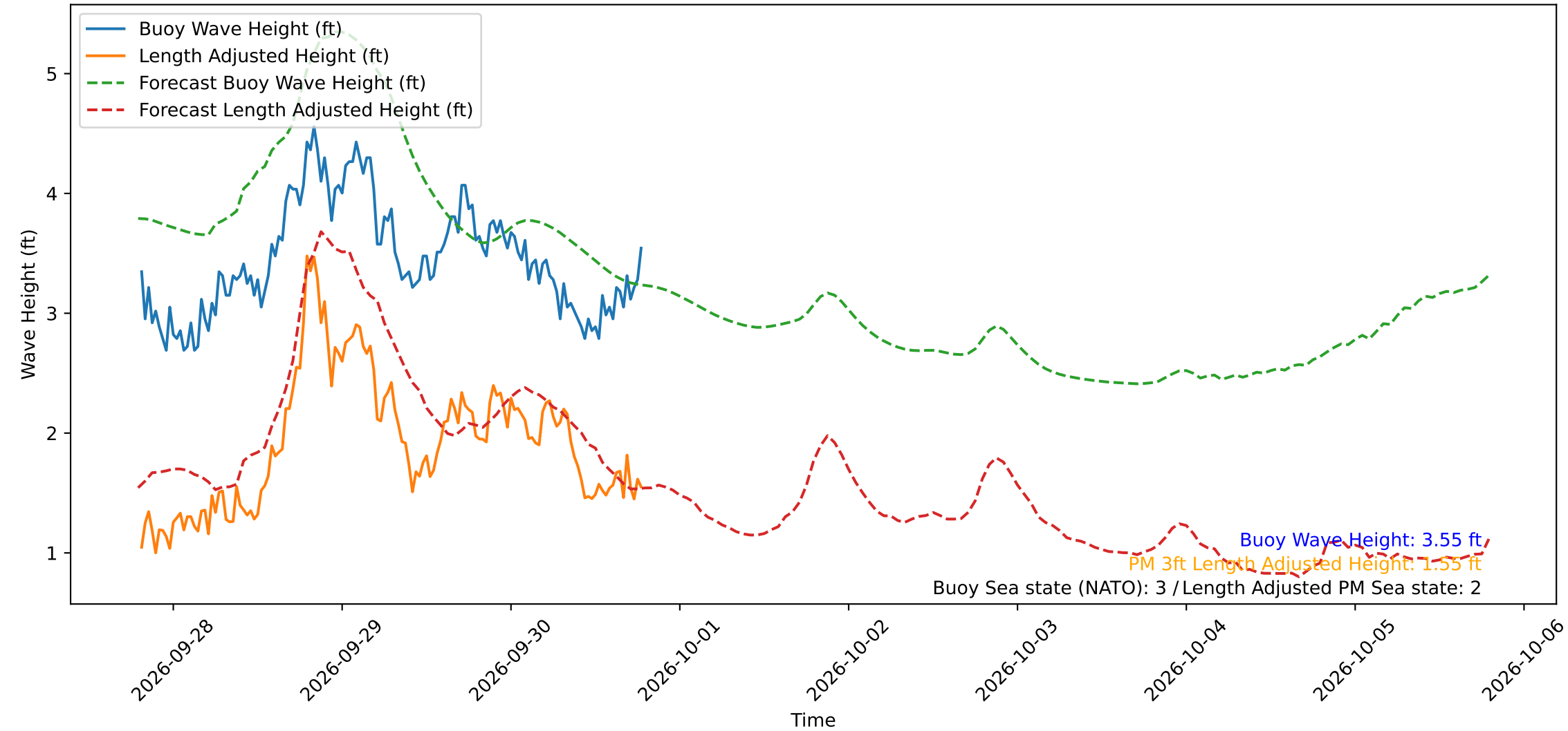
Wave Heights over Time for Green Beach at 2026-09-30 19:11:12
