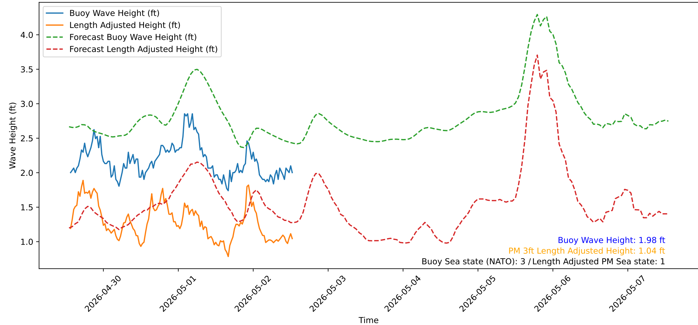
Wave Heights over Time for Green Beach at 2026-05-02 13:21:14
