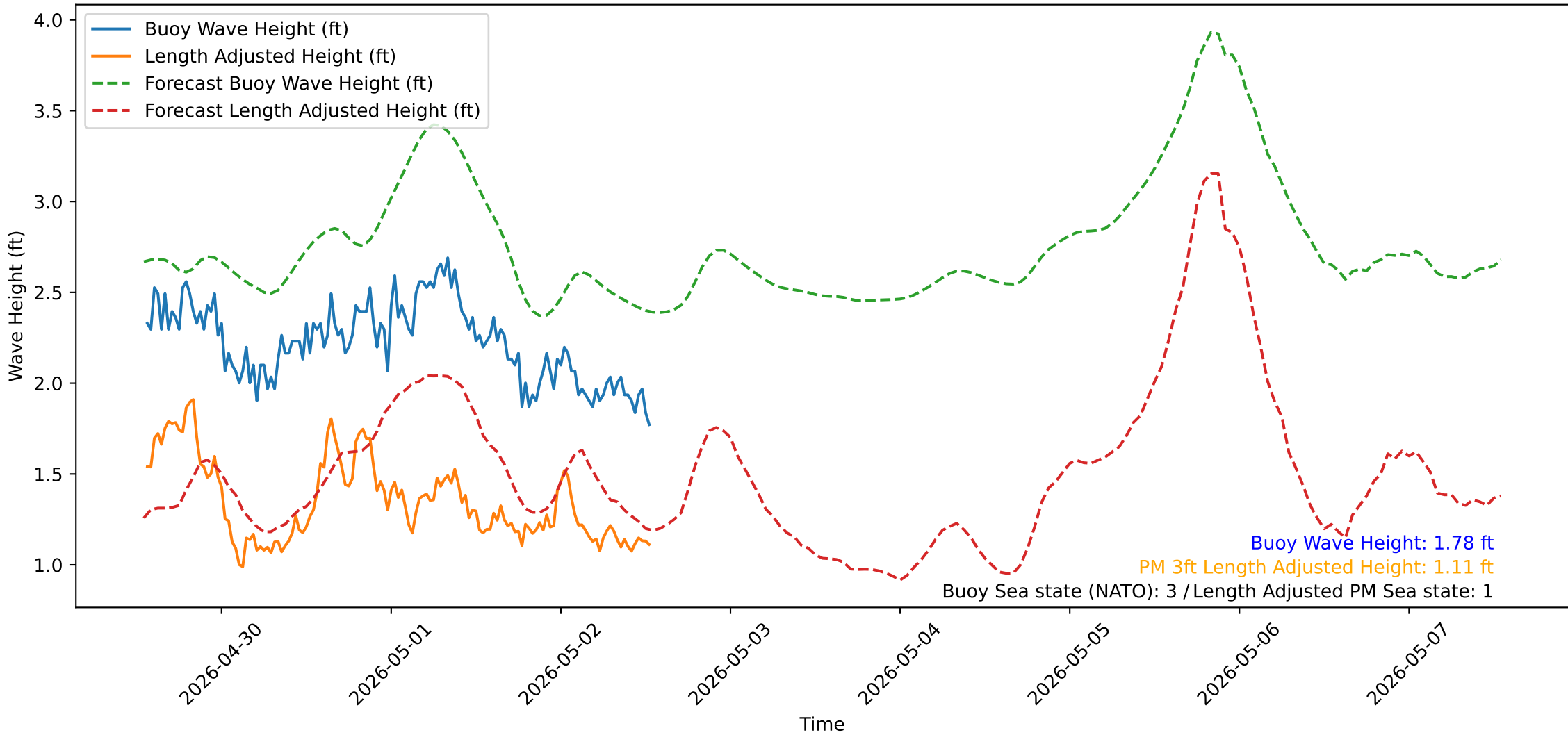
Wave Heights over Time for Oceanside Harbor at 2026-05-02 13:20:31
