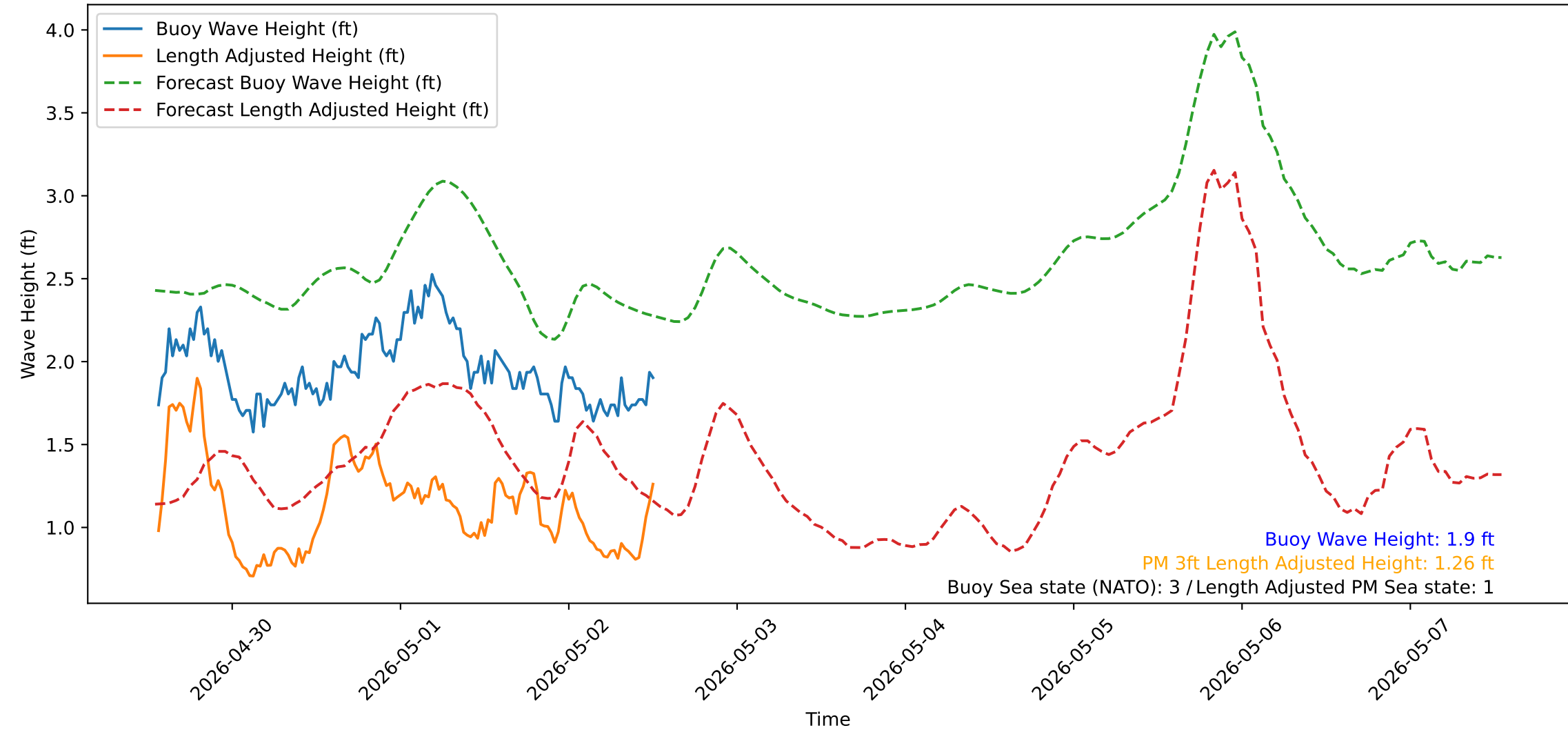
Wave Heights over Time for Red Beach at 2026-05-02 13:20:52
