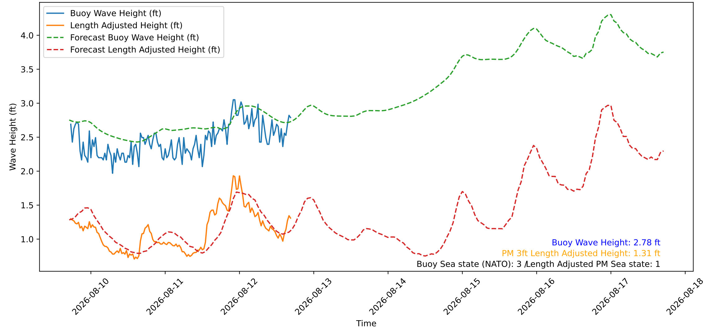
Wave Heights over Time for Oceanside Harbor at 2026-08-12 17:20:26
