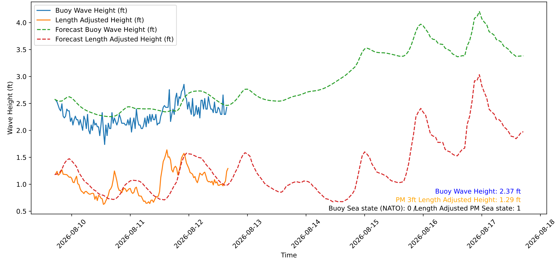
Wave Heights over Time for Red Beach at 2026-08-12 17:20:47
